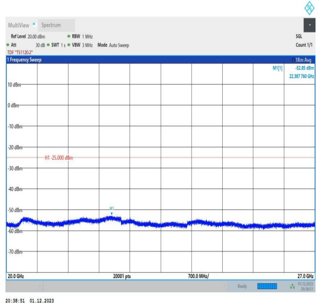
7-7-20MHz-20MHz-16QAM-16QAM-20850-21048-1RB#0-1RB #99-20000~27000MHz-PASS
