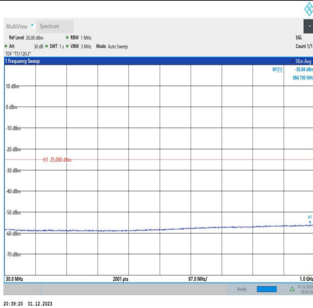
7-7-20MHz-20MHz-64QAM-64QAM-20850-21048-1RB#0-1RB #99-30~1000MHz-PASS
