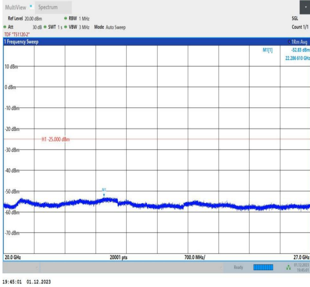
7-7-20MHz-15MHz-16QAM-16QAM-21201-21372-1RB#99-0R B#0-20000~27000MHz-PASS
