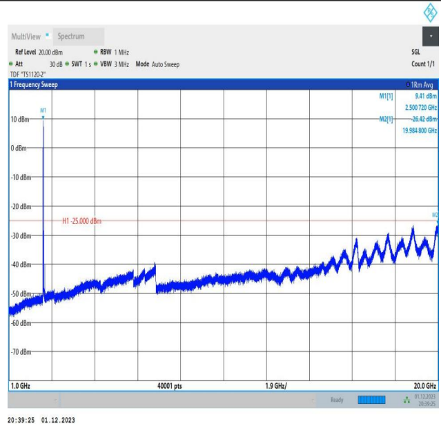
7-7-20MHz-20MHz-64QAM-64QAM-20850-21048-1RB#0-1RB #99-1000~20000MHz-PASS
