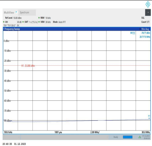
7-7-20MHz-20MHz-16QAM-16QAM-20850-21048-100RB#0-1 00RB#0-0.15~30MHz-PASS
