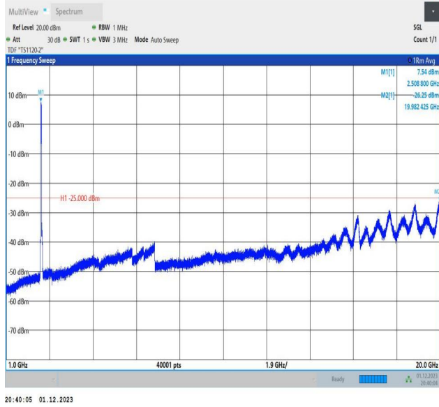
7-7-20MHz-20MHz-QPSK-QPSK-20850-21048-100RB#0-100 RB#0-1000~20000MHz-PASS
