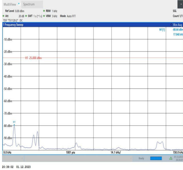
7-7-20MHz-20MHz-64QAM-64QAM-20850-21048-1RB#0-1RB #99-0.009~0.15MHz-PASS
