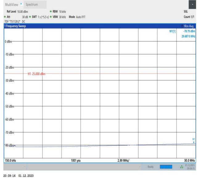
7-7-20MHz-20MHz-64QAM-64QAM-20850-21048-1RB#0-1RB #99-0.15~30MHz-PASS
