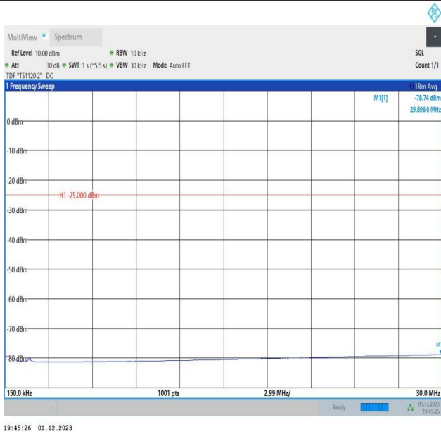
7-7-20MHz-15MHz-64QAM-64QAM-21201-21372-1RB#99-0R B#0-0.15~30MHz-PASS
