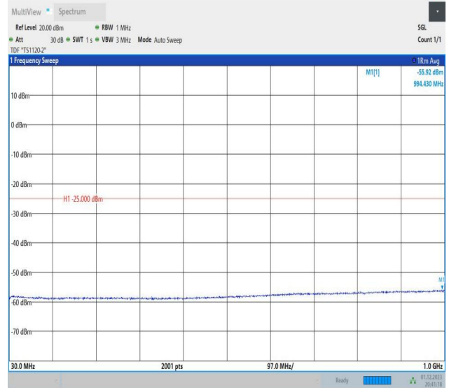
7-7-20MHz-20MHz-64QAM-64QAM-20850-21048-100RB#0-1 00RB#0-30~1000MHz-PASS
