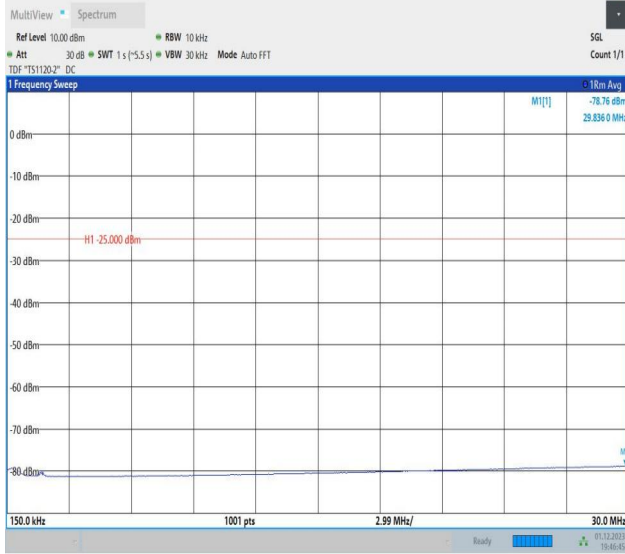
7-7-20MHz-15MHz-16QAM-16QAM-21201-21372-1RB#0-1RB #74-0.15~30MHz-PASS
