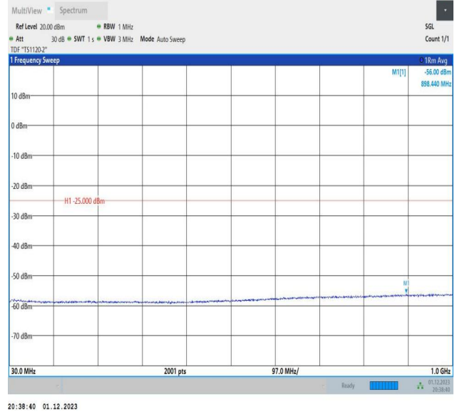
7-7-20MHz-20MHz-16QAM-16QAM-20850-21048-1RB#0-1RB #99-30~1000MHz-PASS
