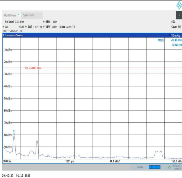
7-7-20MHz-20MHz-16QAM-16QAM-20850-21048-100RB#0-1 00RB#0-0.009~0.15MHz-PASS
