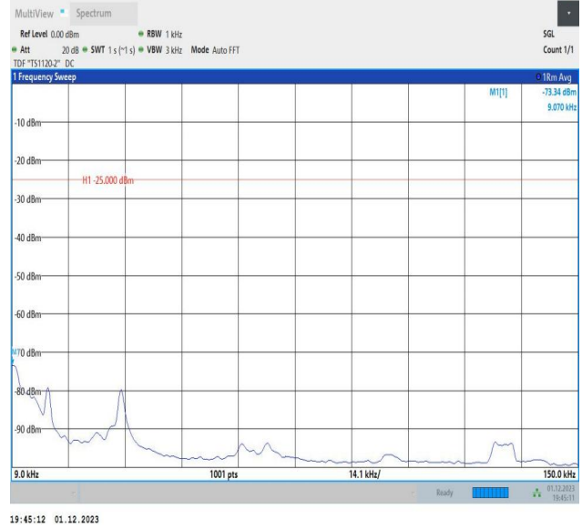
7-7-20MHz-15MHz-64QAM-64QAM-21201-21372-1RB#99-0R B#0-0.009~0.15MHz-PASS
