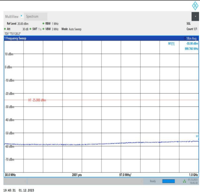
7-7-20MHz-15MHz-64QAM-64QAM-21201-21372-1RB#99-0R B#0-30~1000MHz-PASS
