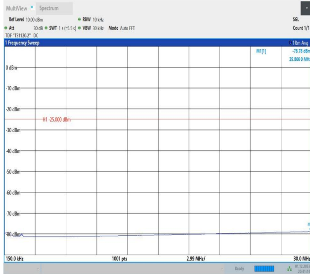
7-7-20MHz-20MHz-64QAM-64QAM-20850-21048-100RB#0-1 00RB#0-0.15~30MHz-PASS
