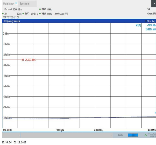
7-7-20MHz-20MHz-16QAM-16QAM-20850-21048-1RB#0-1RB #99-0.15~30MHz-PASS
