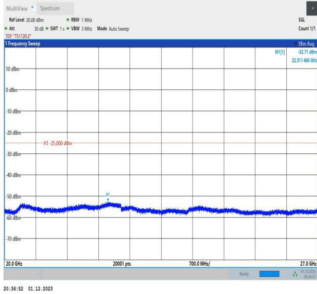
7-7-20MHz-20MHz-16QAM-16QAM-20850-21048-1RB#99-0R B#0-20000~27000MHz-PASS
