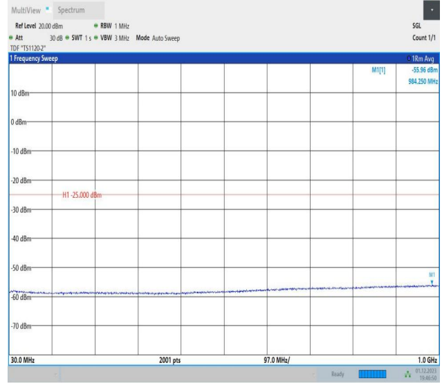
7-7-20MHz-15MHz-16QAM-16QAM-21201-21372-1RB#0-1RB #74-30~1000MHz-PASS
