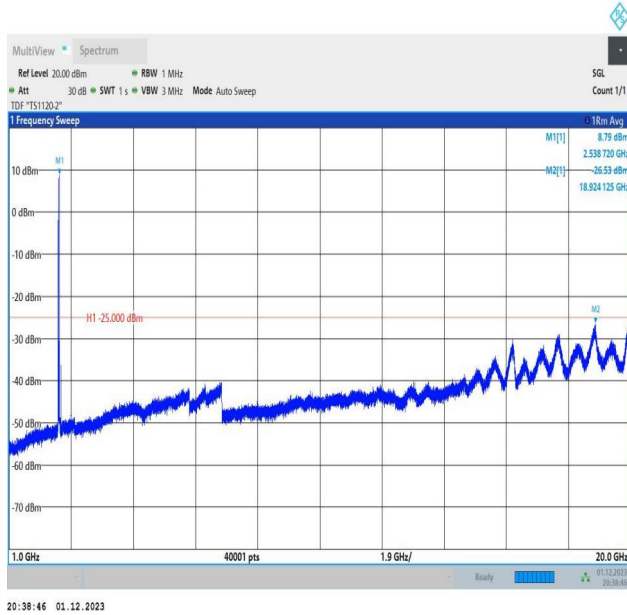
7-7-20MHz-20MHz-16QAM-16QAM-20850-21048-1RB#0-1RB #99-1000~20000MHz-PASS
