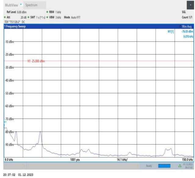
7-7-20MHz-20MHz-64QAM-64QAM-20850-21048-1RB#99-0R B#0-0.009~0.15MHz-PASS
