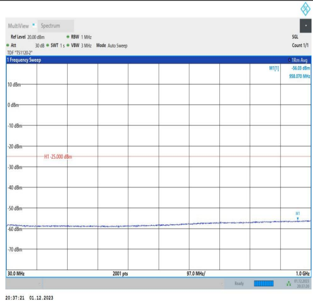
7-7-20MHz-20MHz-64QAM-64QAM-20850-21048-1RB#99-0R B#0-30~1000MHz-PASS
