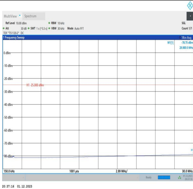
7-7-20MHz-20MHz-64QAM-64QAM-20850-21048-1RB#99-0R B#0-0.15~30MHz-PASS
