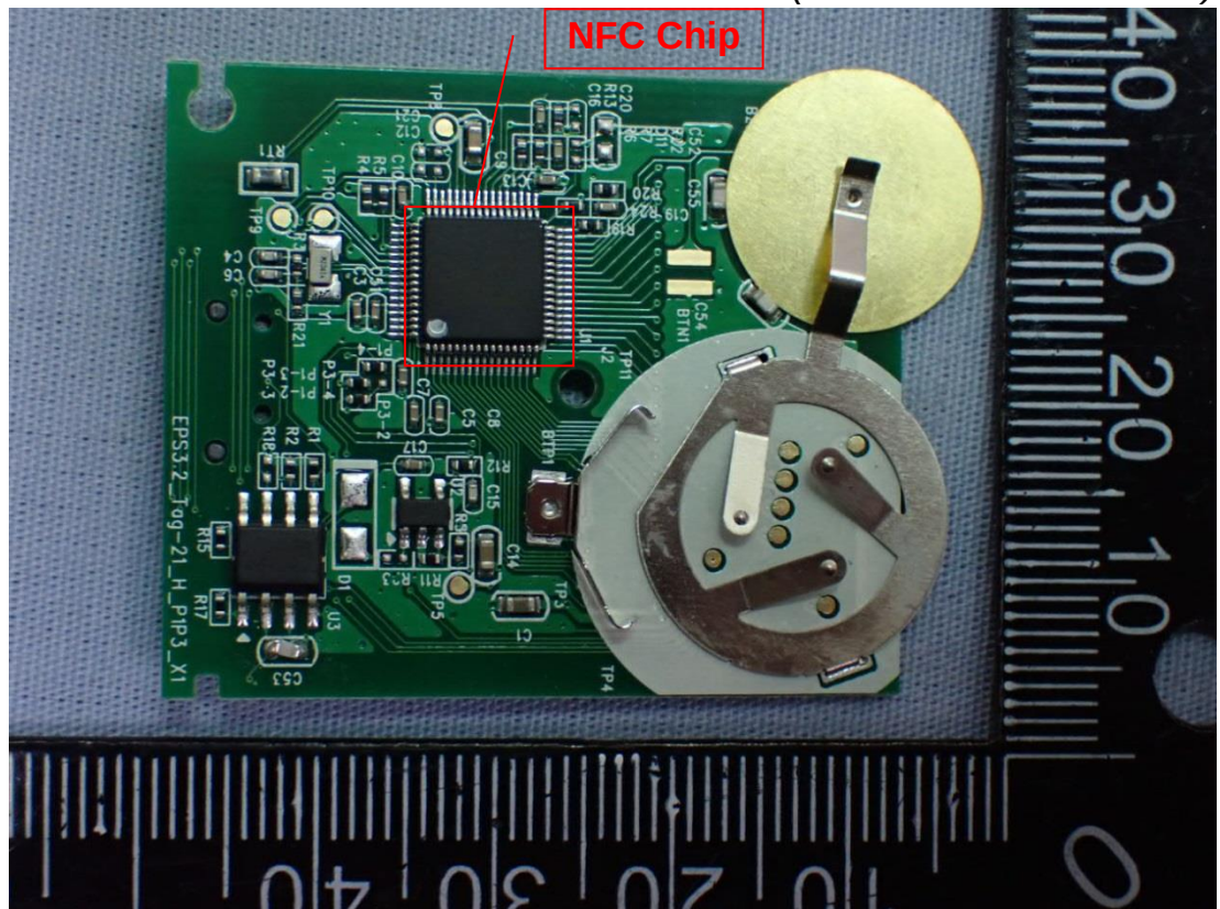
Figure 26 Internal View(Main Board/ Front View)
