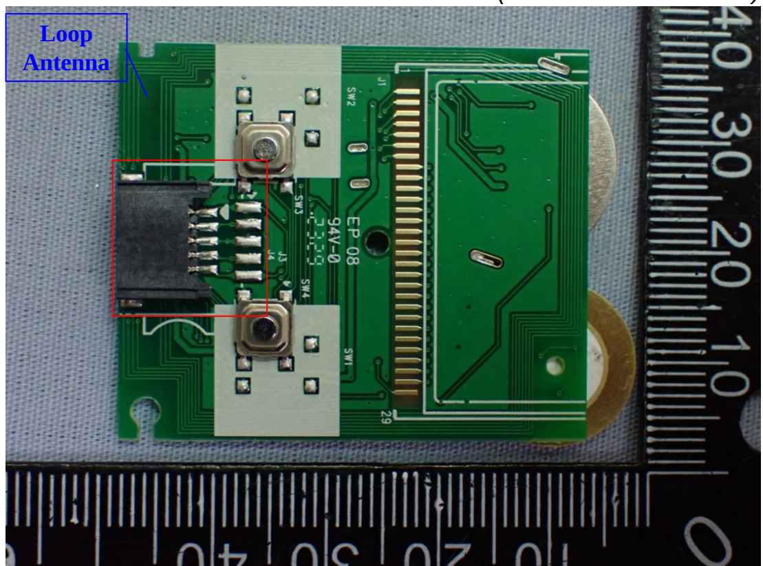
Figure 27 Internal View(Main Board/ Back View)
