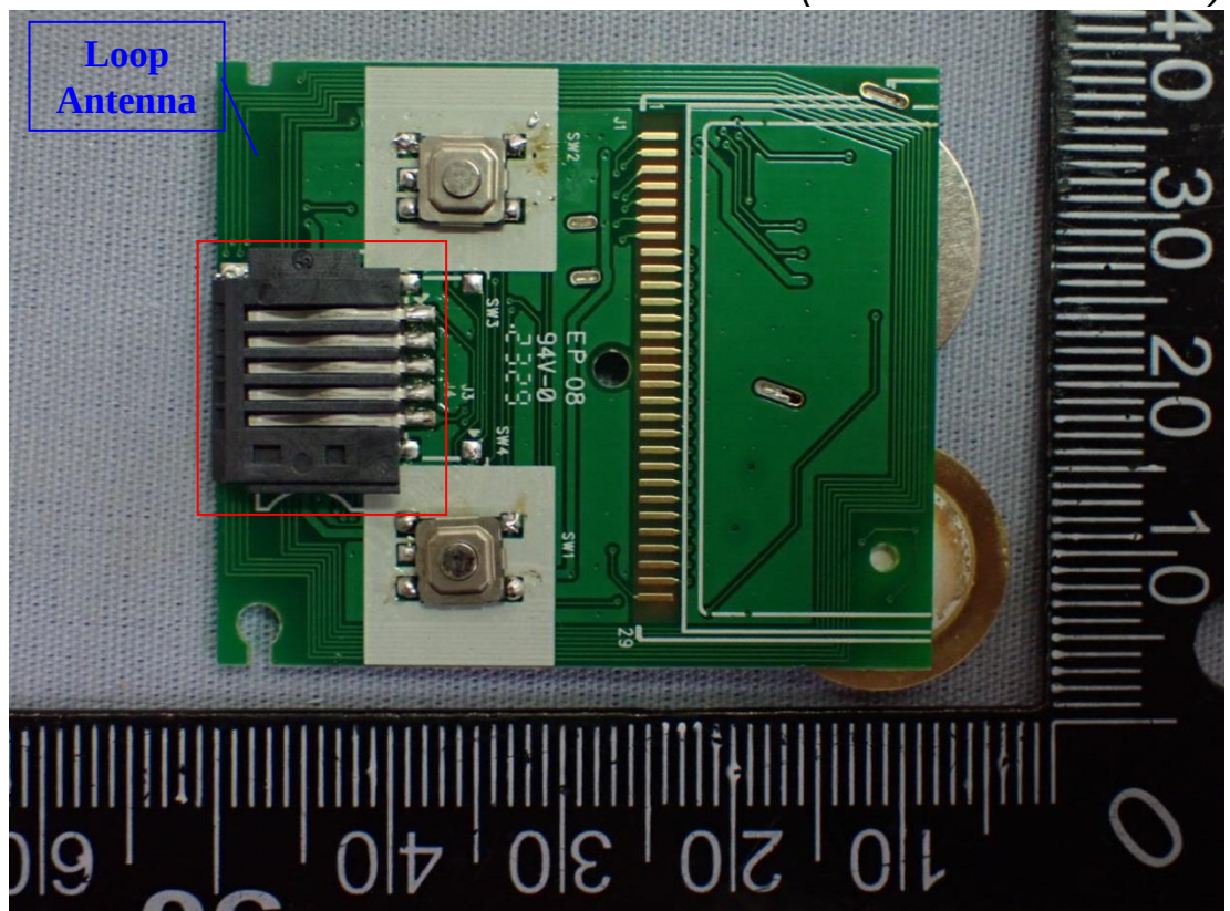
Figure 15 Internal View(Main Board/ Back View)
