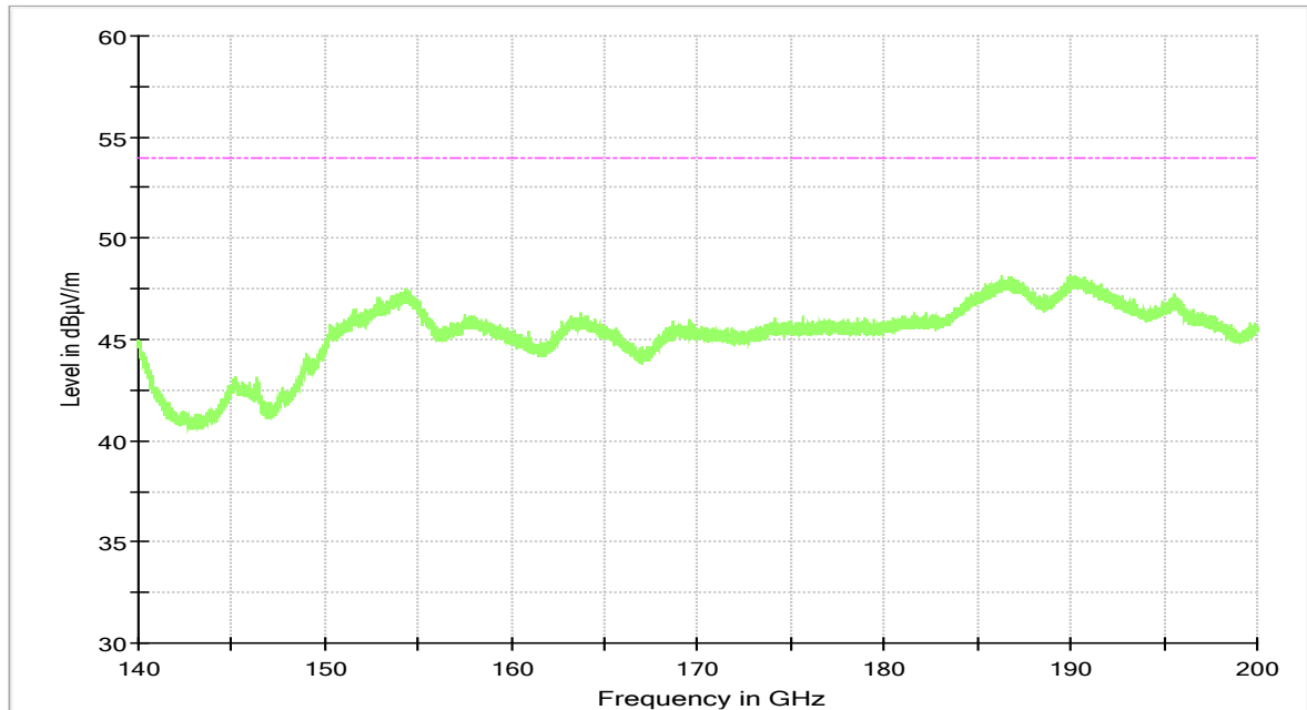
S01_AC01 140 GHz – 200 GHz
