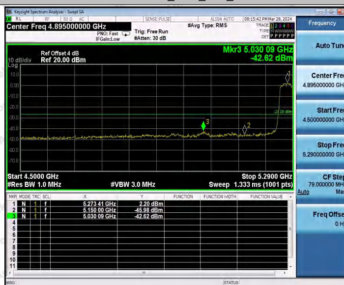
11AC40MIMO_Ant1_High_5310
