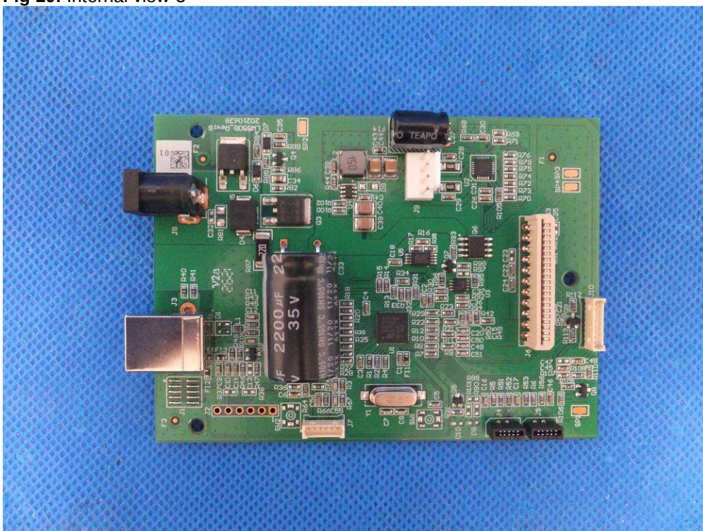
Fig 11: Main PCB top view
