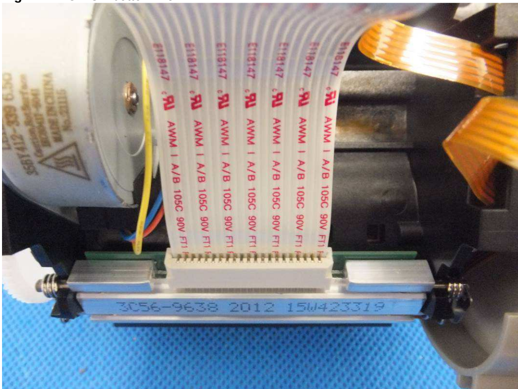
Fig 15: Print header view
