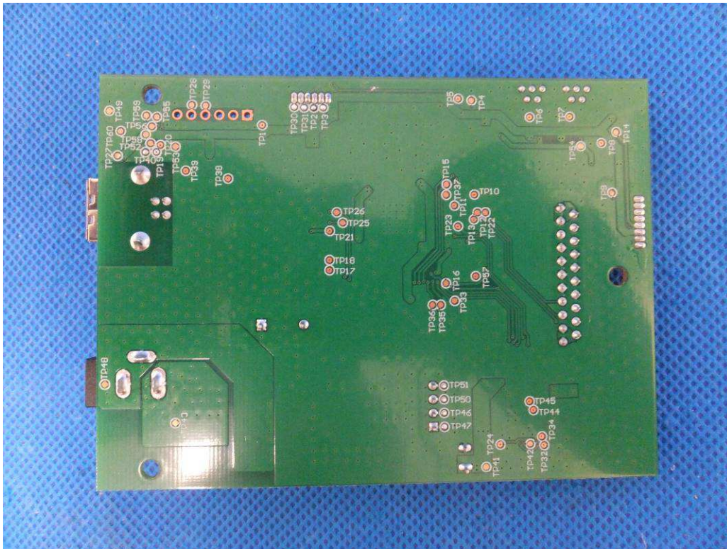
Fig 12: Main PCB bottom view
