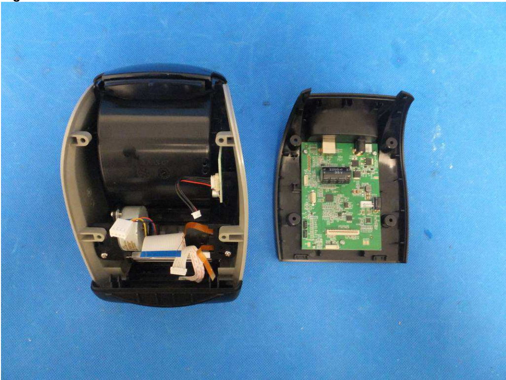
Fig 9: Internal view-2
