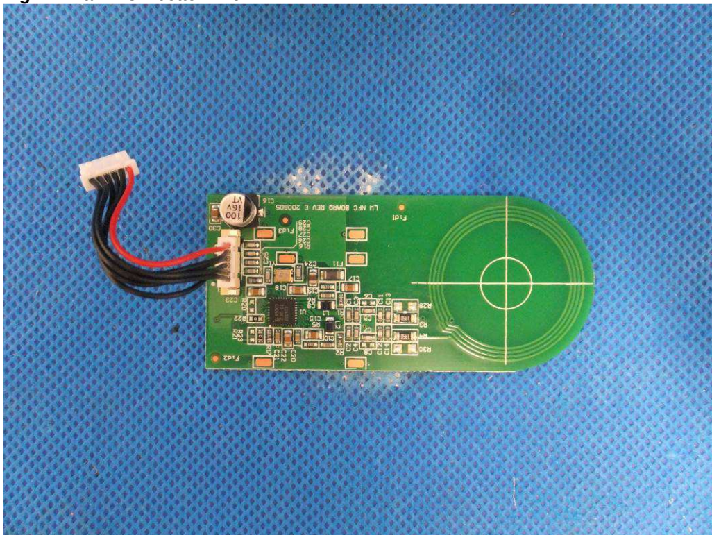
Fig 13: NFC PCB top view
