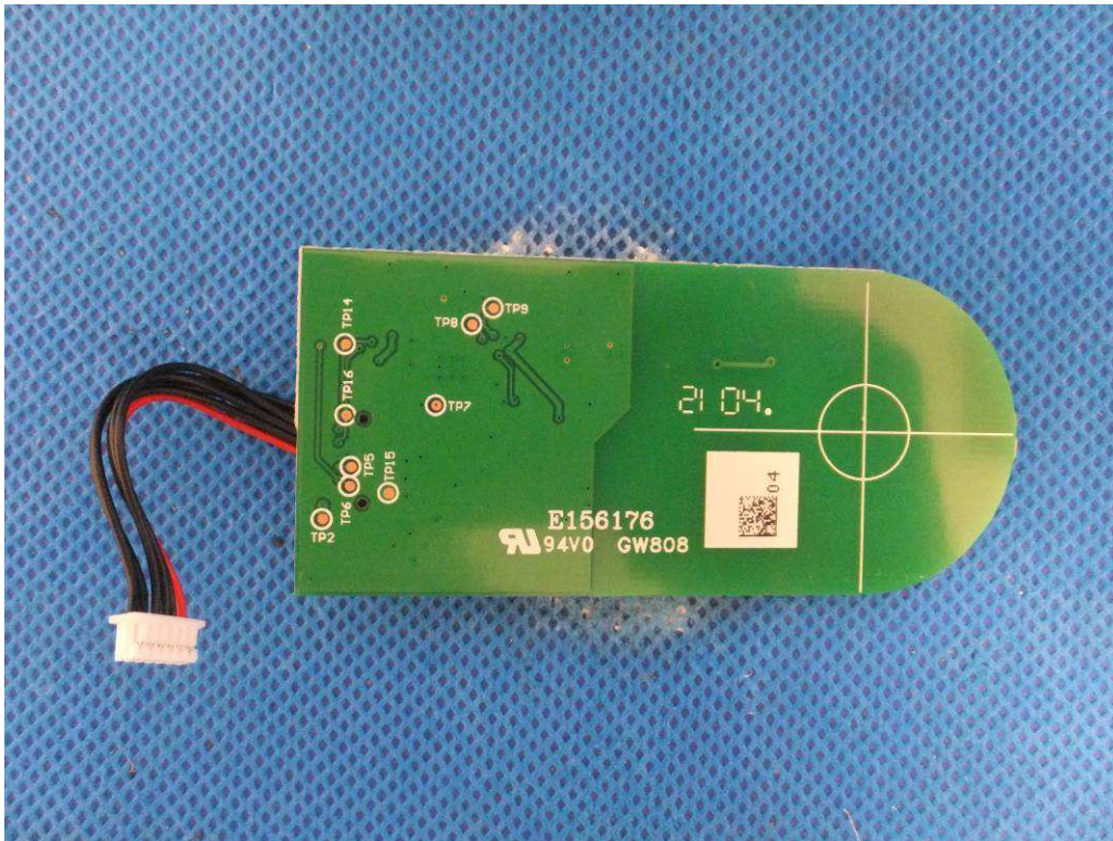
Fig 14: NFC PCB bottom view
