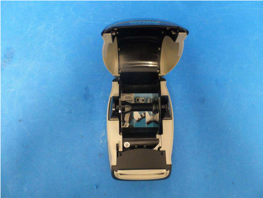
Fig 8: Internal view-1
