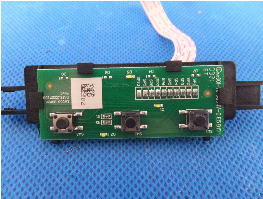
Fig 16: Button PCB view
