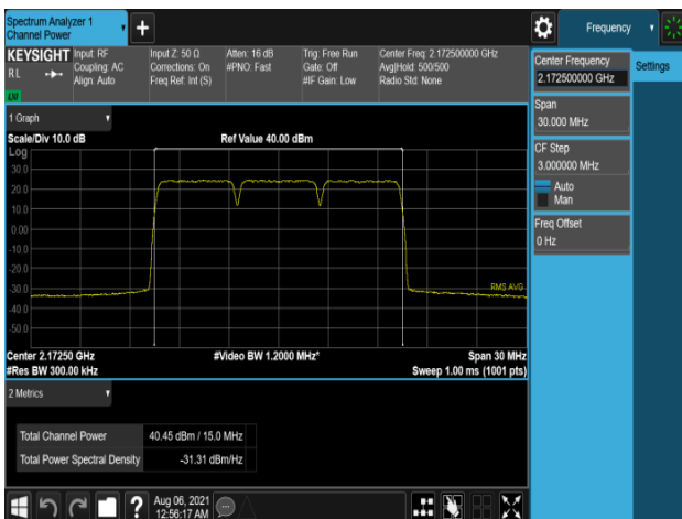
Plot 7-467. Conducted Average Output Power Plot (B66_5M+5M+5M_3C_64QAM - High Channel, Port 2)
