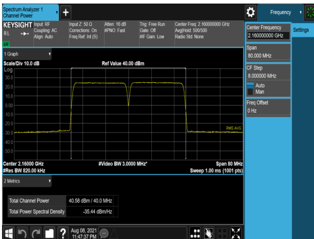
Plot 7-455. Conducted Average Output Power Plot (B66_20M+20M_2C_64QAM – High Channel, Port 2)
