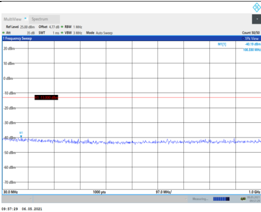
Band2-20MHz-16QAM-18700-1RB#0- Range1:30~1000MHz
