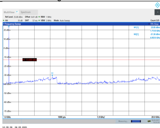
Band66-3MHz-16QAM-131987-1RB#0- Range2:1000~20000MHz
