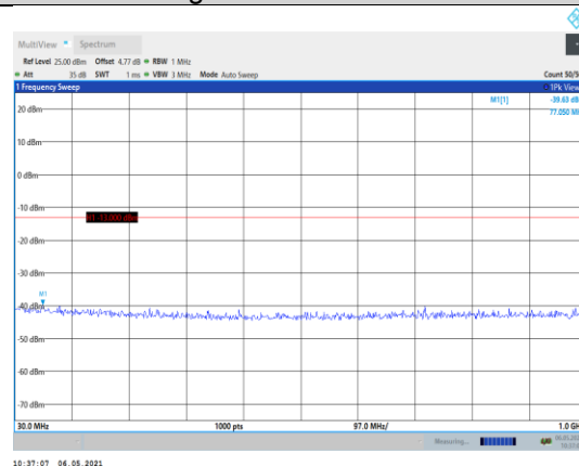
Band66-3MHz-16QAM-132657-1RB#0- Range1:30~1000MHz
