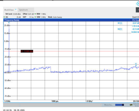
Band4-10MHz-16QAM-20350-1RB#0- Range2:1000~20000MHz
