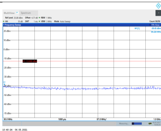
Band66-15MHz-QPSK-132047-1RB#0- Range1:30~1000MHz
