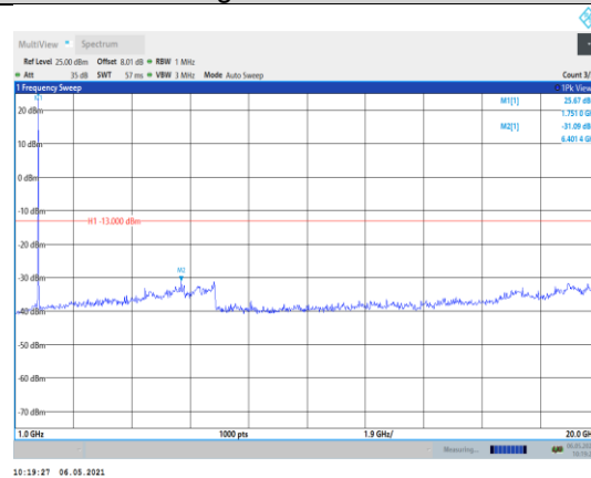
Band4-5MHz-16QAM-20375-1RB#0- Range2:1000~20000MHz
