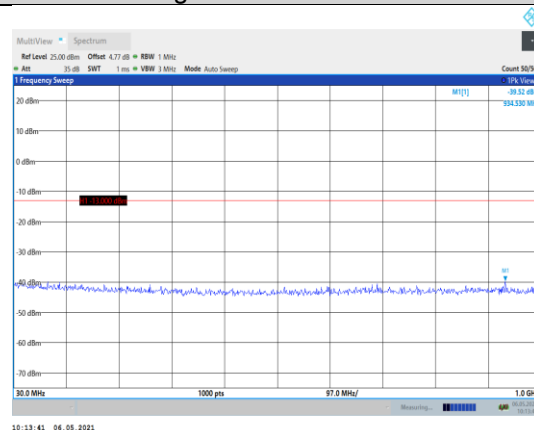
Band4-3MHz-QPSK-20385-1RB#0- Range1:30~1000MHz
