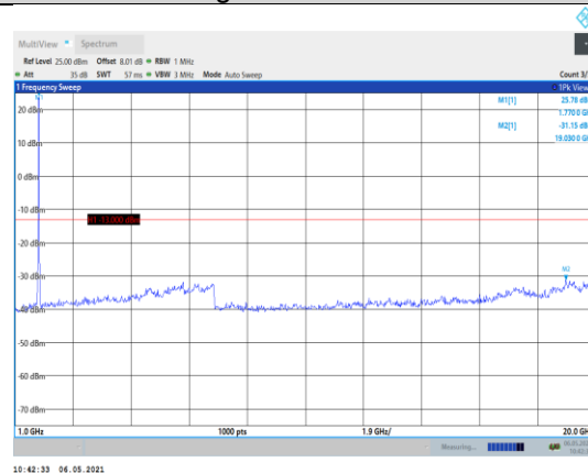
Band66-15MHz-16QAM-132597-1RB#0- Range2:1000~20000MHz
