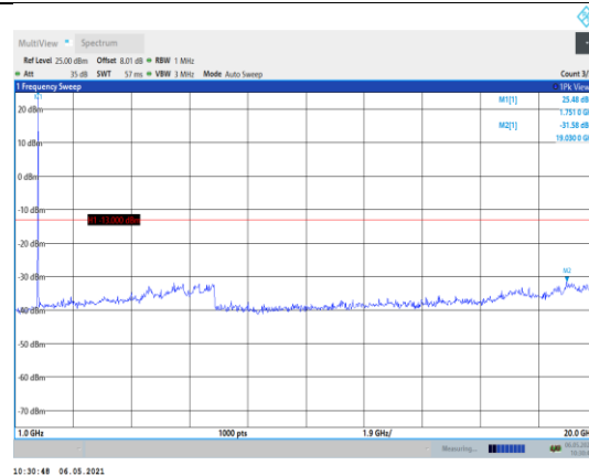
Band66-5MHz-QPSK-132322-1RB#0- Range2:1000~20000MHz
