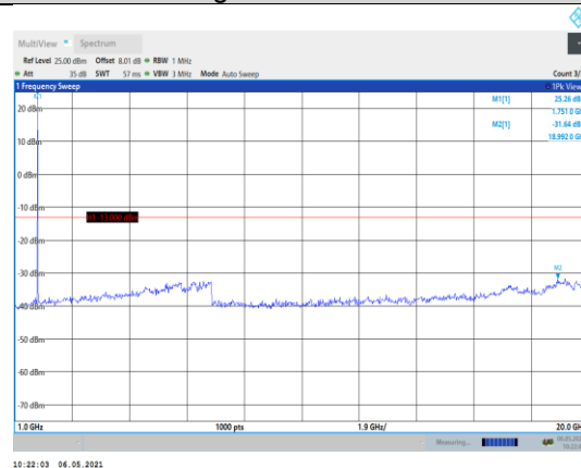
Band4-1.4MHz-16QAM-20393-1RB#0- Range2:1000~20000MHz
