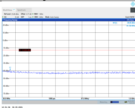
Band66-5MHz-16QAM-132322-1RB#0- Range1:30~1000MHz
