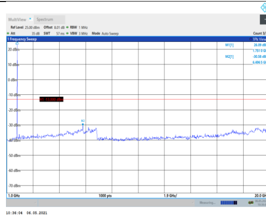
Band66-3MHz-QPSK-132322-1RB#0- Range2:1000~20000MHz
