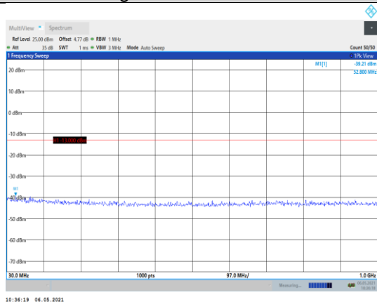
Band66-3MHz-16QAM-132322-1RB#0- Range1:30~1000MHz
