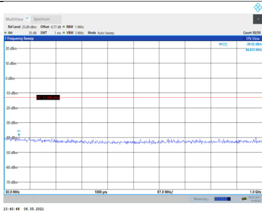
Band66-15MHz-16QAM-132047-1RB#0- Range1:30~1000MHz
