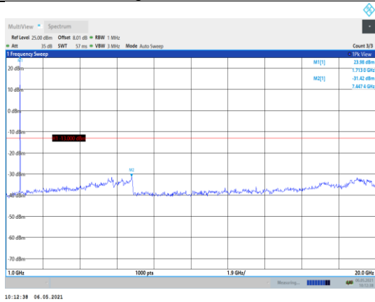
Band4-3MHz-16QAM-19965-1RB#0- Range2:1000~20000MHz
