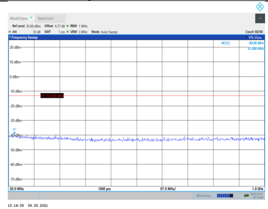
Band4-3MHz-16QAM-20385-1RB#0- Range1:30~1000MHz
