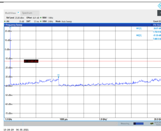
Band4-20MHz-16QAM-20175-1RB#0- Range2:1000~20000MHz
