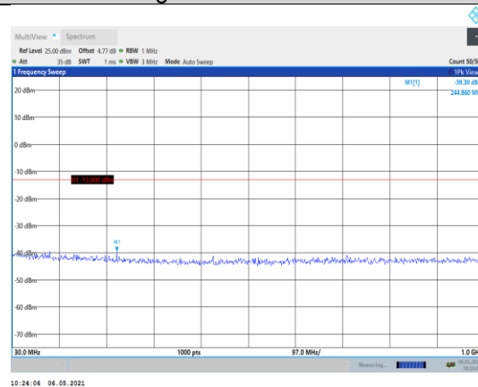
Band4-15MHz-QPSK-20325-1RB#0- Range1:30~1000MHz
