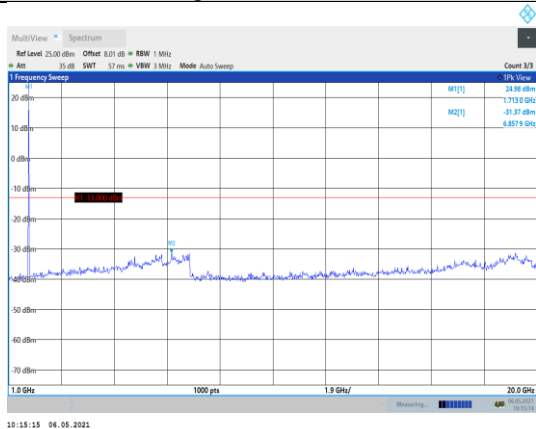
Band4-10MHz-16QAM-20000-1RB#0- Range2:1000~20000MHz
