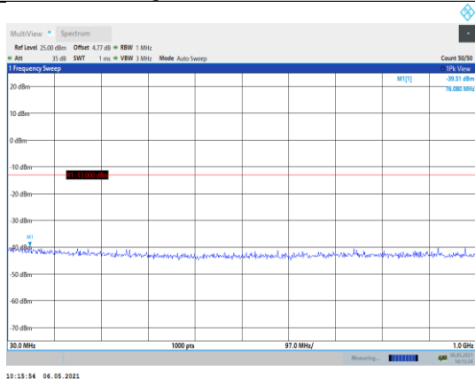
Band4-10MHz-16QAM-20175-1RB#0- Range1:30~1000MHz
