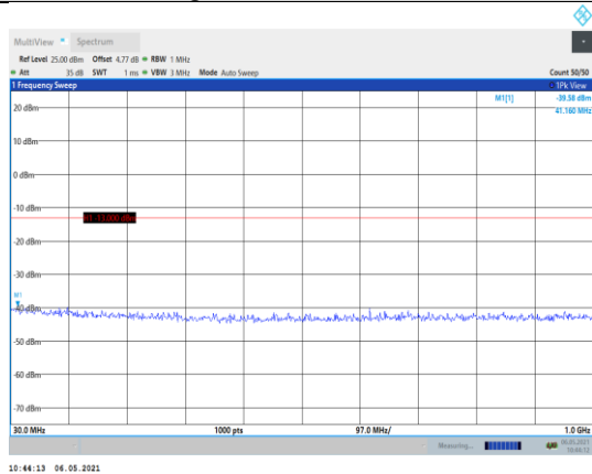
Band66-10MHz-16QAM-132322-1RB#0- Range1:30~1000MHz
