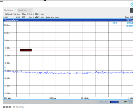
Band4-5MHz-16QAM-20375-1RB#0- Range1:30~1000MHz
