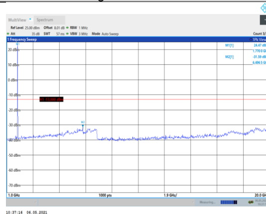
Band66-3MHz-16QAM-132657-1RB#0- Range2:1000~20000MHz
