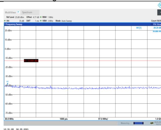
Band66-5MHz-QPSK-132647-1RB#0- Range1:30~1000MHz
