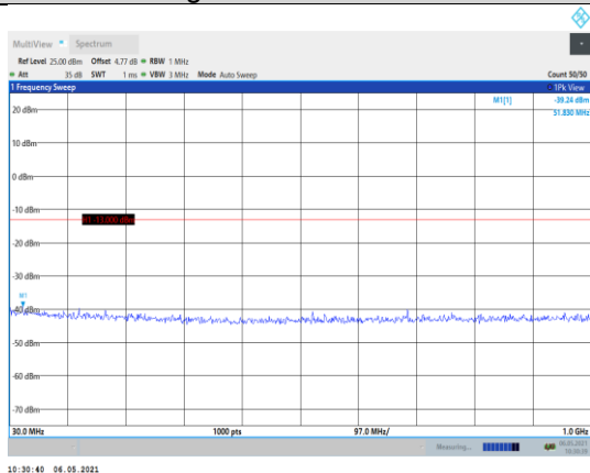
Band66-5MHz-QPSK-132322-1RB#0- Range1:30~1000MHz
