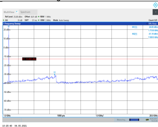
Band4-20MHz-16QAM-20050-1RB#0- Range2:1000~20000MHz
