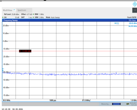
Band4-10MHz-QPSK-20175-1RB#0- Range1:30~1000MHz
