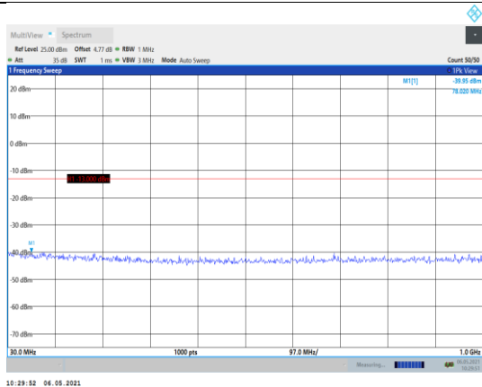
Band66-5MHz-QPSK-131997-1RB#0- Range1:30~1000MHz
