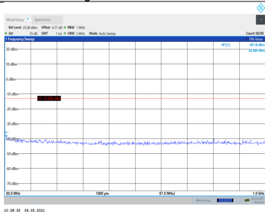
Band66-1.4MHz-QPSK-132322-1RB#0- Range1:30~1000MHz
