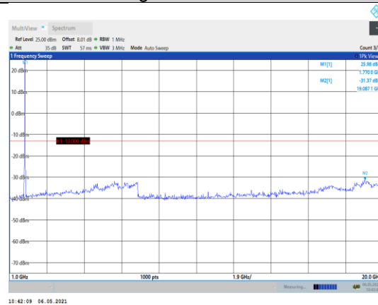
Band66-15MHz-QPSK-132597-1RB#0- Range2:1000~20000MHz
