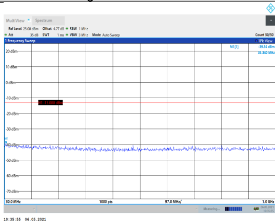
Band66-3MHz-QPSK-132322-1RB#0- Range1:30~1000MHz
