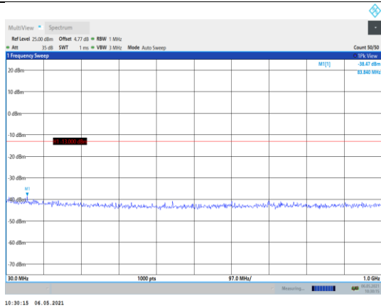
Band66-5MHz-16QAM-131997-1RB#0- Range1:30~1000MHz
