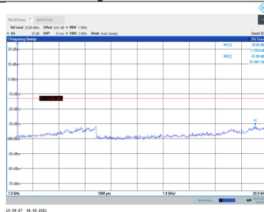
Band66-1.4MHz-QPSK-132665-1RB#0- Range2:1000~20000MHz
