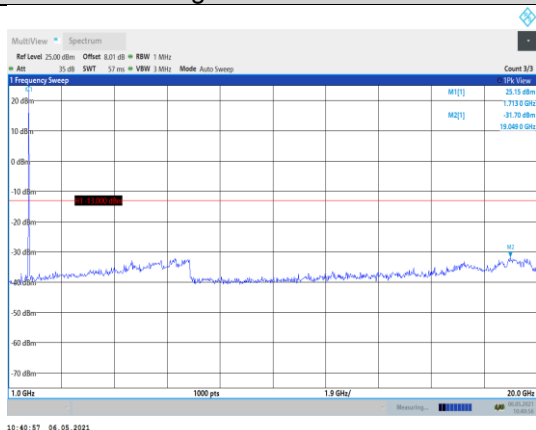
Band66-15MHz-16QAM-132047-1RB#0- Range2:1000~20000MHz
