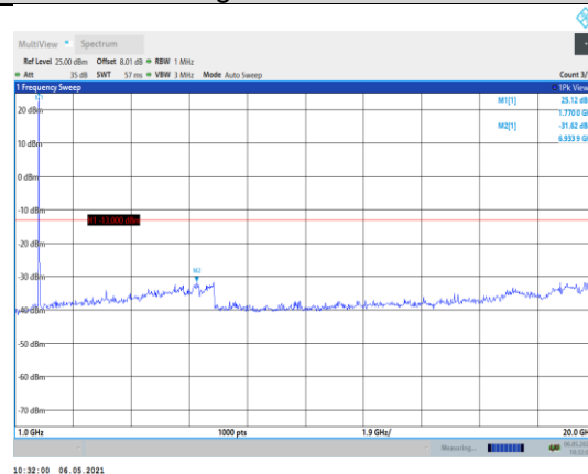
Band66-5MHz-16QAM-132647-1RB#0- Range2:1000~20000MHz
