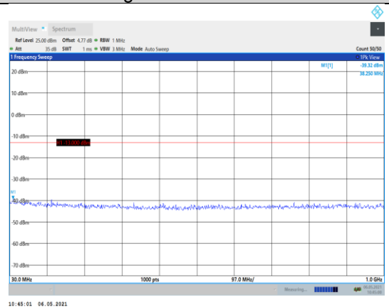
Band66-10MHz-16QAM-132622-1RB#0- Range1:30~1000MHz
