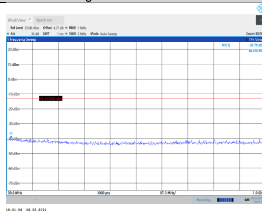
Band4-1.4MHz-16QAM-20393-1RB#0- Range1:30~1000MHz
