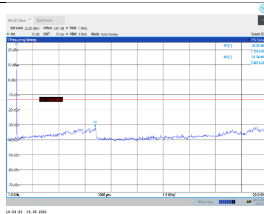
Band4-15MHz-QPSK-20175-1RB#0- Range2:1000~20000MHz
