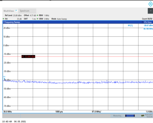
Band66-10MHz-QPSK-132322-1RB#0- Range1:30~1000MHz
