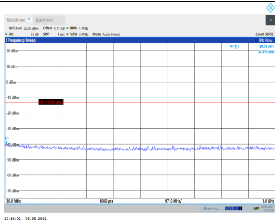
Band66-10MHz-QPSK-132022-1RB#0- Range1:30~1000MHz
