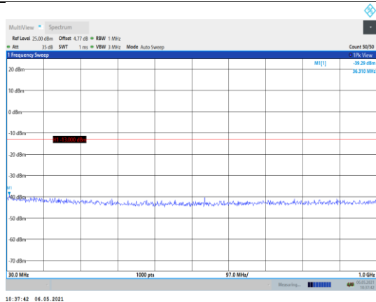
Band66-1.4MHz-QPSK-131979-1RB#0- Range1:30~1000MHz
