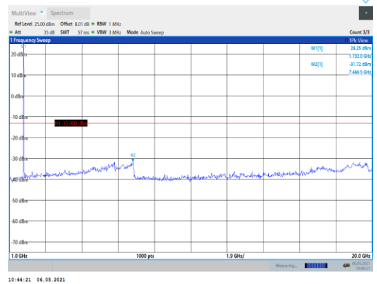
Band66-10MHz-16QAM-132322-1RB#0- Range2:1000~20000MHz
