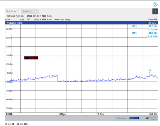
Band66-10MHz-QPSK-132322-1RB#0- Range2:1000~20000MHz
