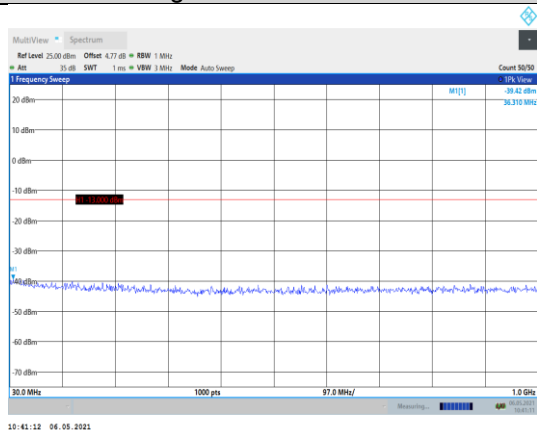
Band66-15MHz-QPSK-132322-1RB#0- Range1:30~1000MHz
