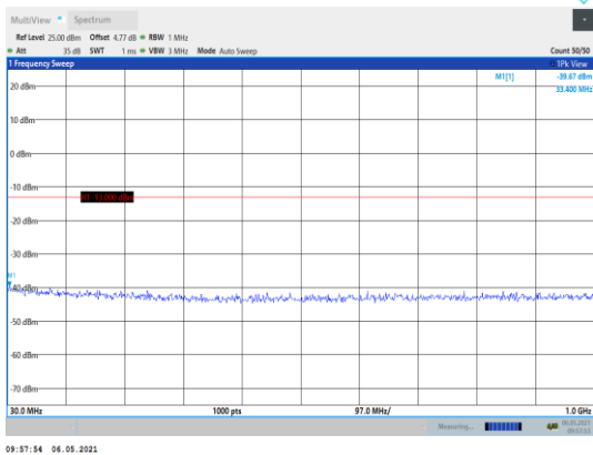
Band2-20MHz-QPSK-18900-1RB#0- Range1:30~1000MHz
