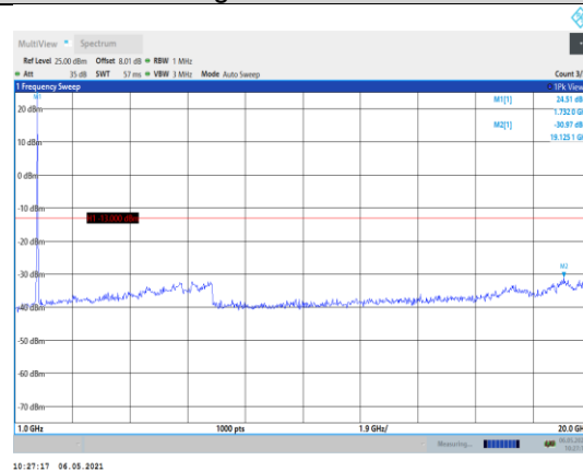
Band4-20MHz-16QAM-20300-1RB#0- Range2:1000~20000MHz
