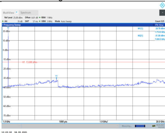
Band4-15MHz-16QAM-20025-1RB#0- Range2:1000~20000MHz
