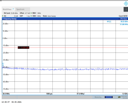
Band66-3MHz-QPSK-131987-1RB#0- Range1:30~1000MHz
