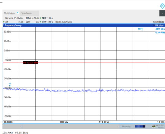
Band4-5MHz-16QAM-19975-1RB#0- Range1:30~1000MHz
