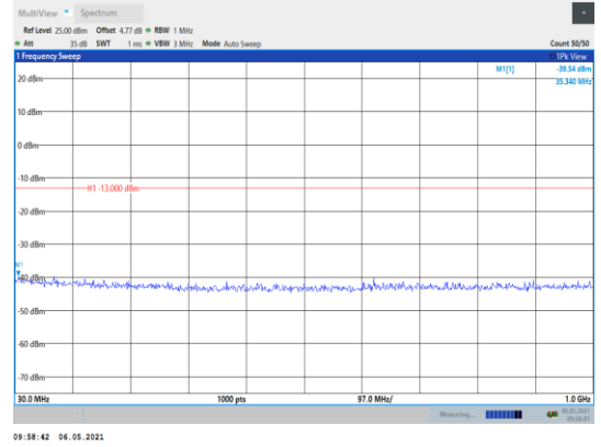
Band2-20MHz-QPSK-19100-1RB#0- Range1:30~1000MHz
