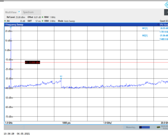
Band66-3MHz-16QAM-132322-1RB#0- Range2:1000~20000MHz
