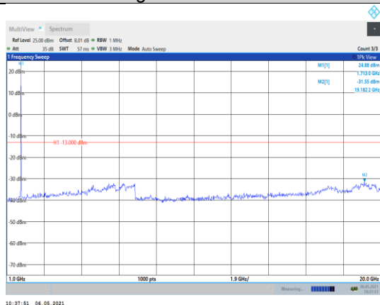
Band66-1.4MHz-QPSK-131979-1RB#0- Range2:1000~20000MHz
