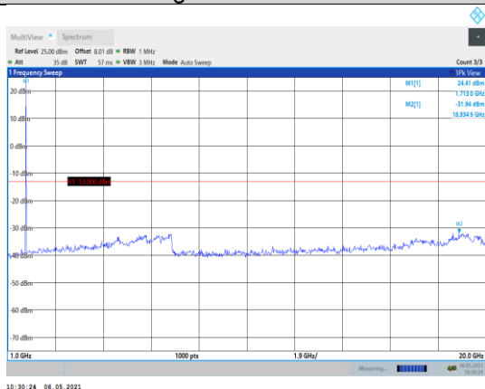
Band66-5MHz-16QAM-131997-1RB#0- Range2:1000~20000MHz
