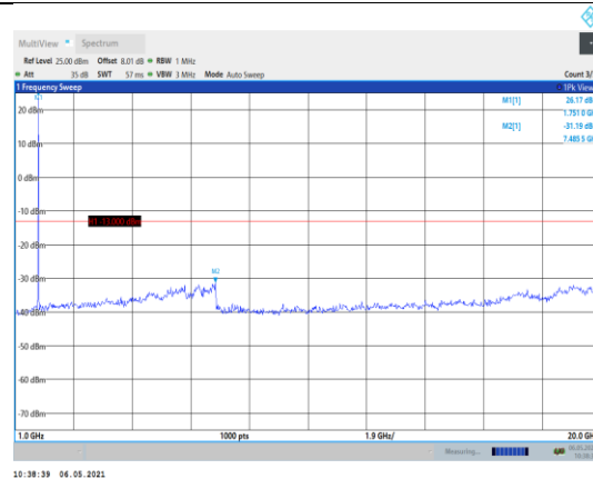
Band66-1.4MHz-QPSK-132322-1RB#0- Range2:1000~20000MHz
