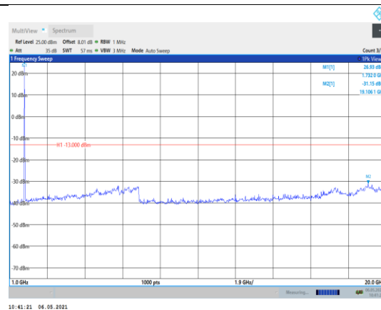
Band66-15MHz-QPSK-132322-1RB#0- Range2:1000~20000MHz
