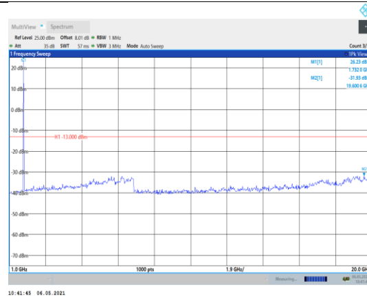
Band66-15MHz-16QAM-132322-1RB#0- Range2:1000~20000MHz
