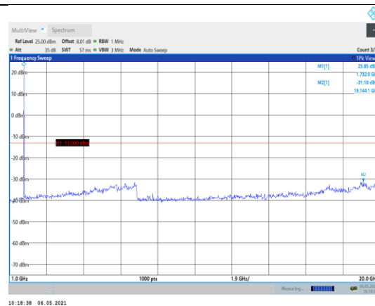
Band4-5MHz-16QAM-20175-1RB#0- Range2:1000~20000MHz
