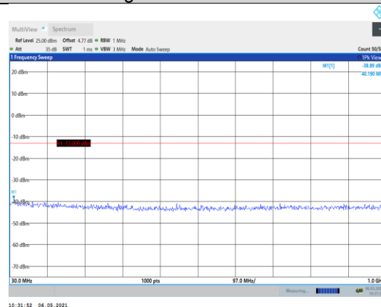
Band66-5MHz-16QAM-132647-1RB#0- Range1:30~1000MHz
