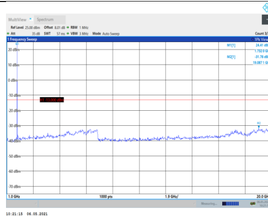
Band4-1.4MHz-16QAM-20175-1RB#0- Range2:1000~20000MHz
