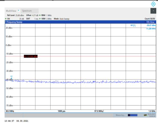
Band66-10MHz-QPSK-132622-1RB#0- Range1:30~1000MHz
