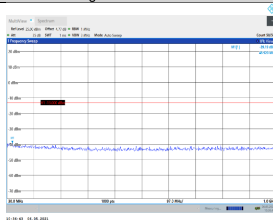
Band66-3MHz-QPSK-132657-1RB#0- Range1:30~1000MHz
