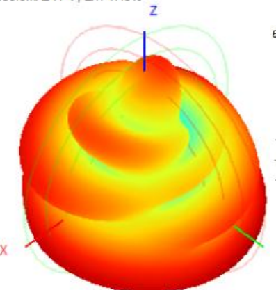
5550.0MHz H+V, Eff: 47.5%
