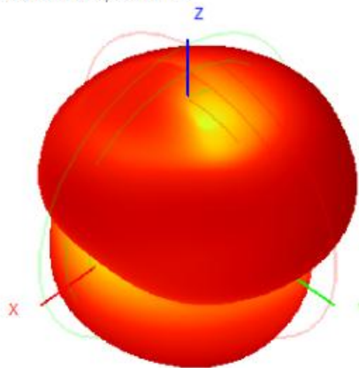
2450.0MHz H+V, Eff: 42.1%
