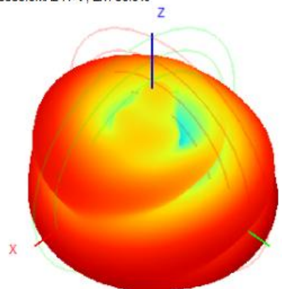
5350.0MHz H+V, Eff: 36.9%
