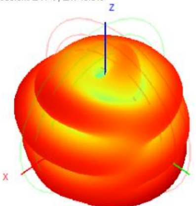
5850.0MHz H+V, Eff: 40.3%
