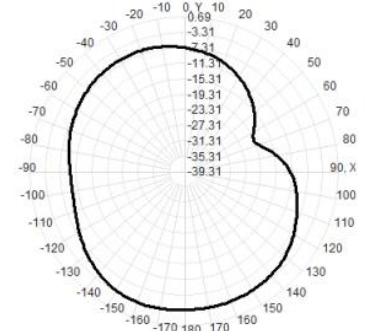
Total(H-XY), Max= -3.40dBi, CirD=16.23
