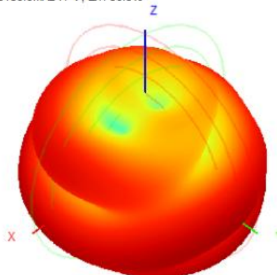
5150.0MHz H+V, Eff: 36.5%
