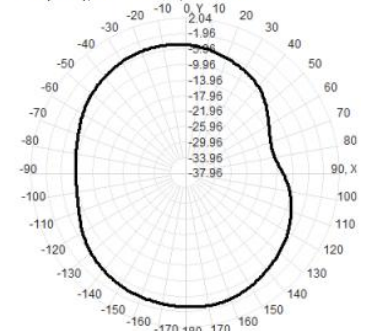
Total(H-XY), Max= -3.29dBi, CirD=11.52
