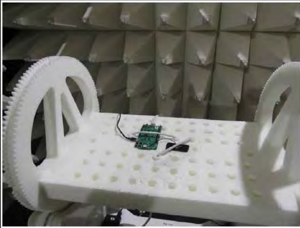
Setup above 1 GHz for Variant 2 (NORA-W101 with external antenna PN PRO-IS-237) -A
