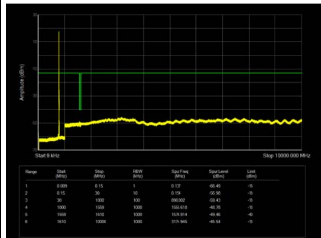
LTE Band 13 10MHz CH-Middle 9kHz ~10GHz
