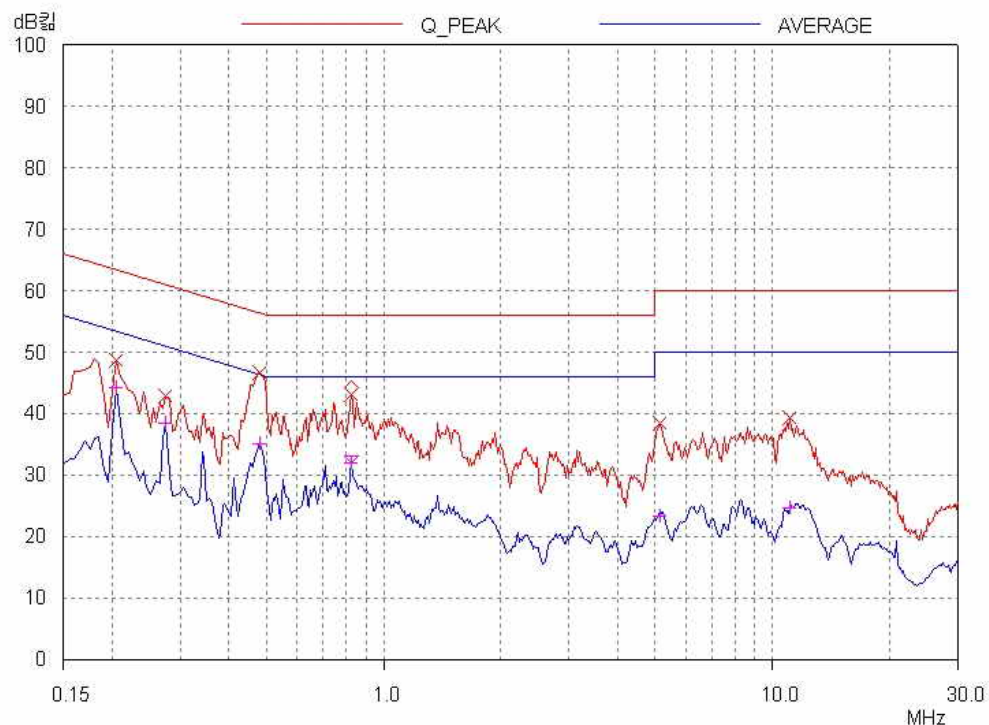
NEUTRAL LINE
