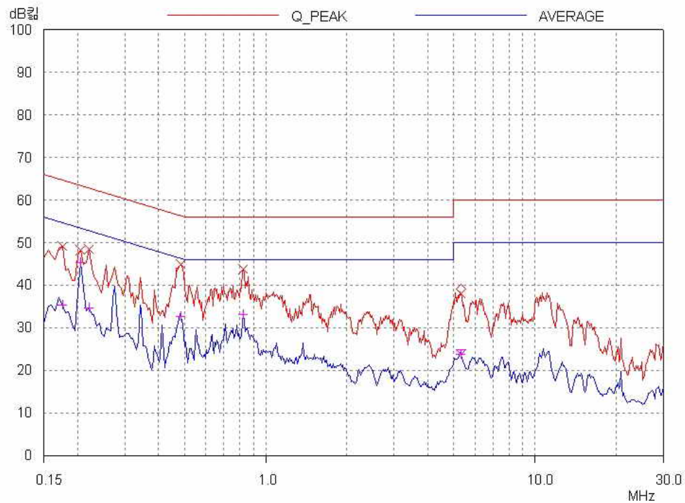
HOT LINE
