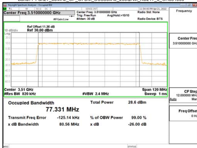
Band77-Part27_80MHz_CP_OFDM_SCS30kHz_256QAM_RB217_0_CH634000
