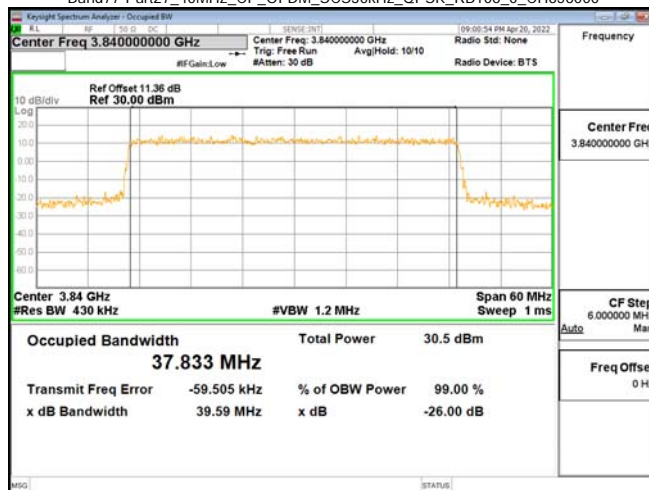
Band77-Part27_40MHz_CP_OFDM_SCS30kHz_QPSK_RB106_0_CH656000
