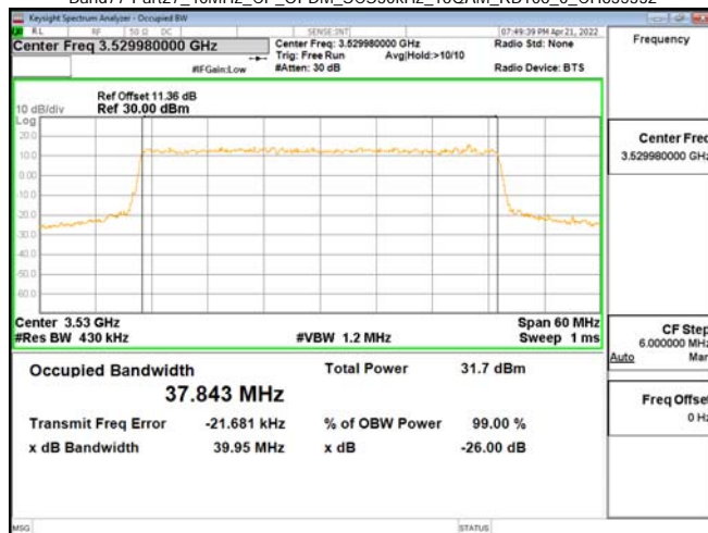
Band77-Part27_40MHz_CP_OFDM_SCS30kHz_16QAM_RB106_0_CH635332
