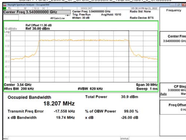
Band77-Part27_20MHz_CP_OFDM_SCS30kHz_16QAM_RB51_0_CH636000
