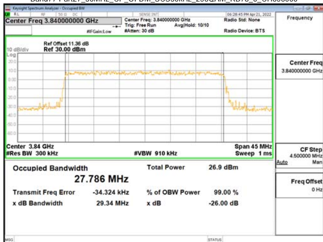
Band77-Part27_30MHz_CP_OFDM_SCS30kHz_256QAM_RB78_0_CH656000
