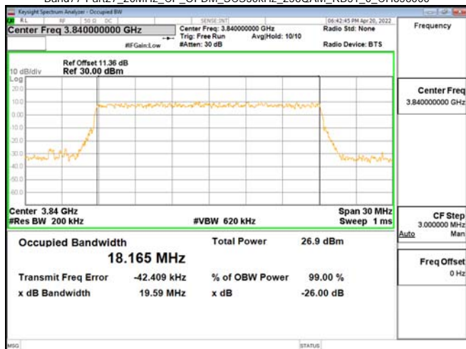
Band77-Part27_20MHz_CP_OFDM_SCS30kHz_256QAM_RB51_0_CH656000
