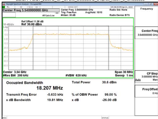
Band77-Part27_20MHz_CP_OFDM_SCS30kHz_64QAM_RB51_0_CH636000
