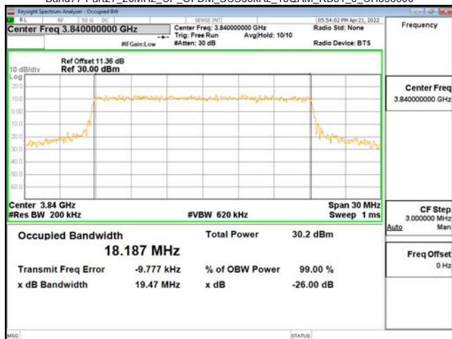
Band77-Part27_20MHz_CP_OFDM_SCS30kHz_16QAM_RB51_0_CH656000
