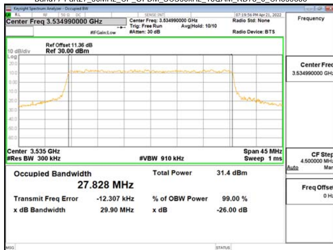
Band77-Part27_30MHz_CP_OFDM_SCS30kHz_16QAM_RB78_0_CH635666
