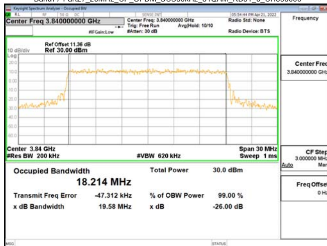
Band77-Part27_20MHz_CP_OFDM_SCS30kHz_64QAM_RB51_0_CH656000
