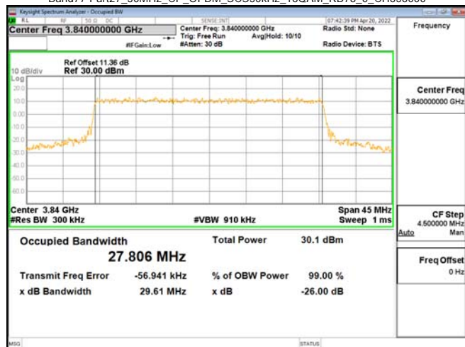
Band77-Part27_30MHz_CP_OFDM_SCS30kHz_16QAM_RB78_0_CH656000
