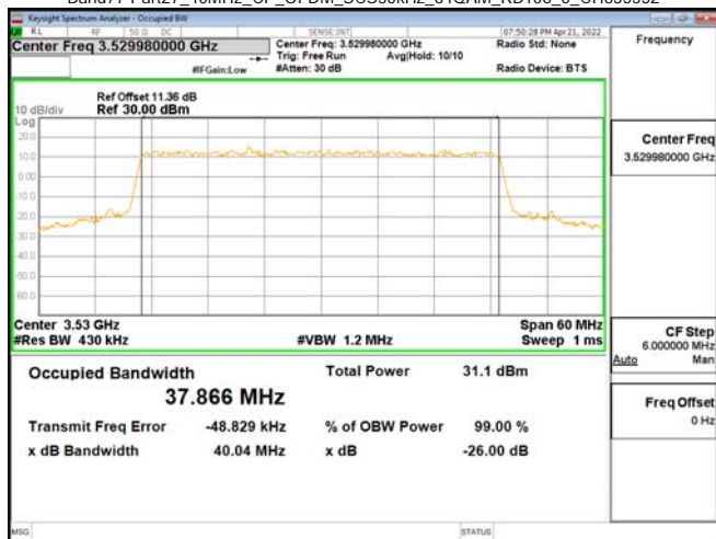
Band77-Part27_40MHz_CP_OFDM_SCS30kHz_64QAM_RB106_0_CH635332
