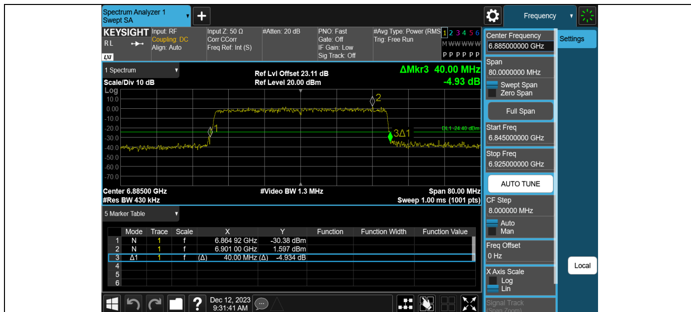
11AX40MIMO-Ant2-6885
