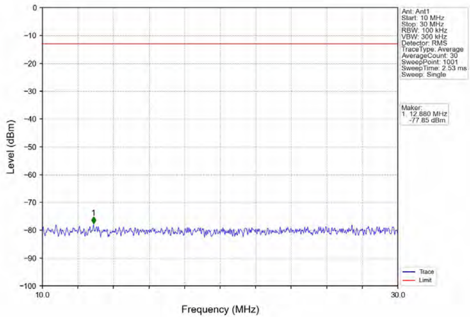
Band17_5MHz_16QAM_HCH_713.5MHz_RB_1_0_NTNV
