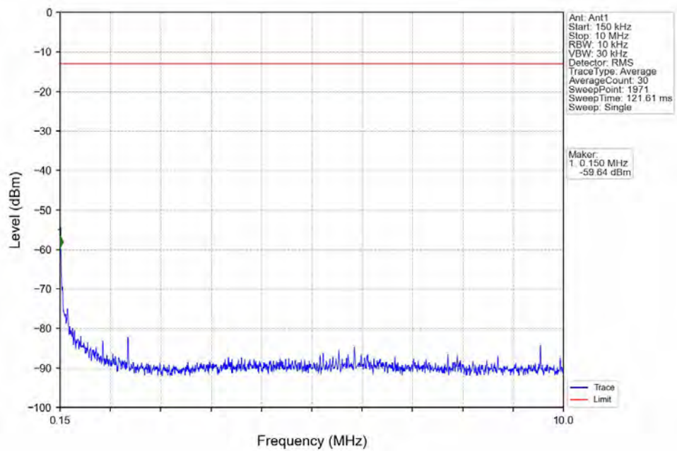
Band17_10MHz_16QAM_HCH_711MHz_RB_1_0_NTNV
