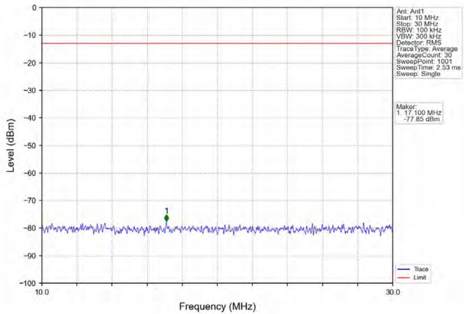
Band17_10MHz_16QAM_MCH_710MHz_RB_1_0_NTNV
