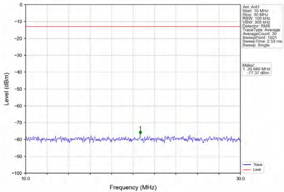
Band17_5MHz_QPSK_MCH_710MHz_RB_1_0_NTNV
