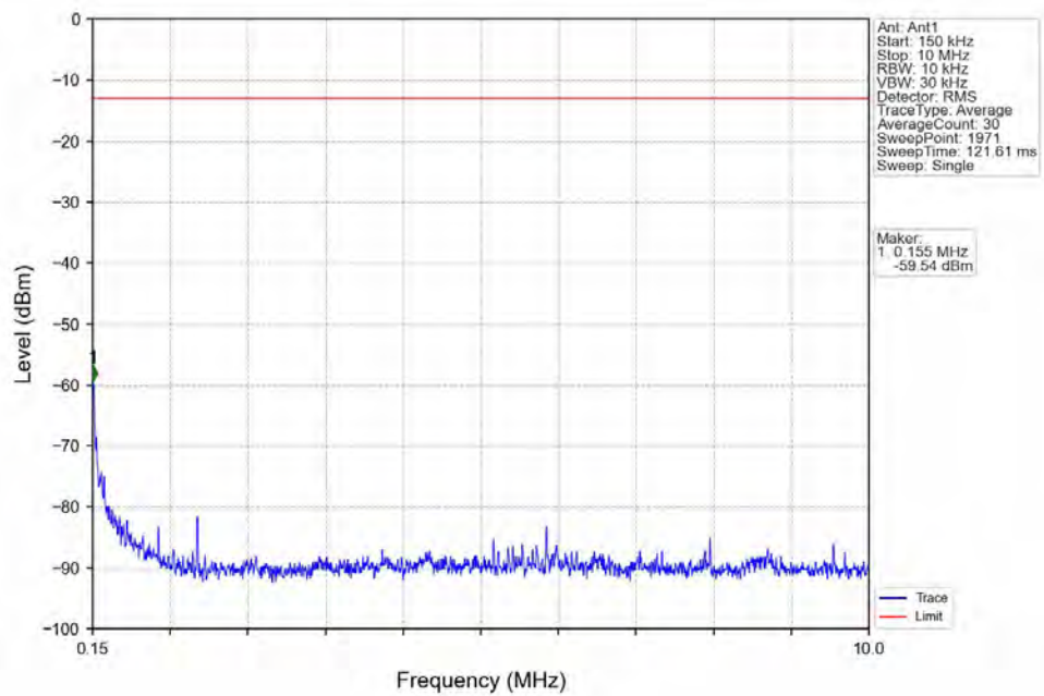
Band17_5MHz_16QAM_HCH_713.5MHz_RB_1_0_NTNV
