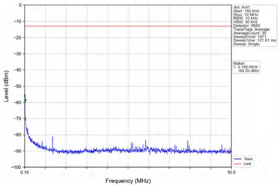
Band17_10MHz_16QAM_MCH_710MHz_RB_1_0_NTNV
