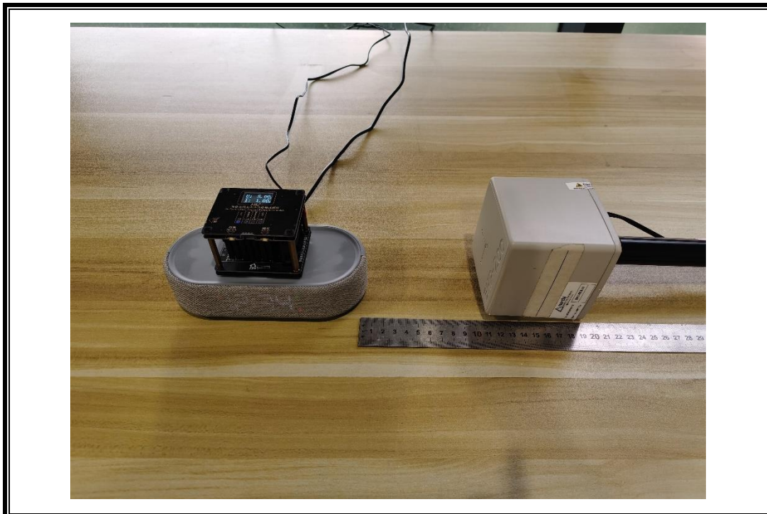
E-FILED AND H-FILED STRENGTH MEASUREMENT SETUP-1
