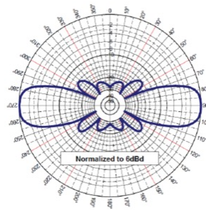
Elevation Pattern (Y, Z or H-plane)
