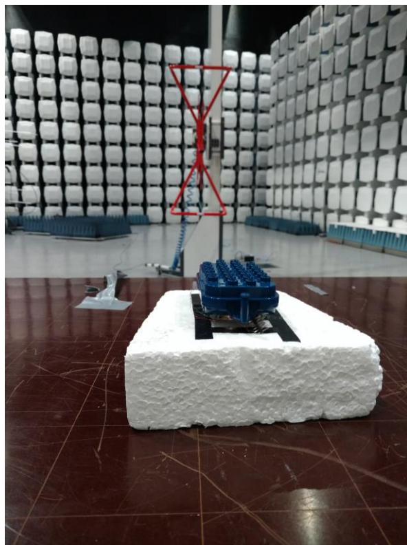
Radiated Emissions 30 – 1000 MHz, device in XY-orientation
