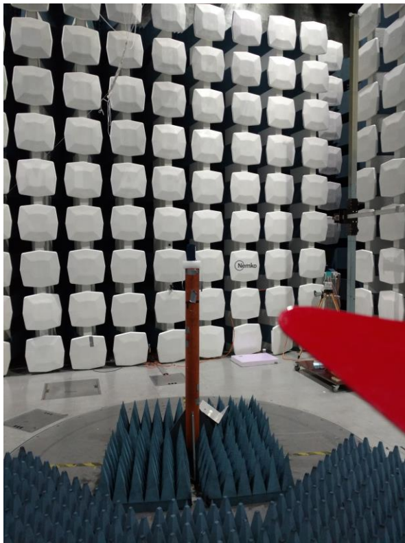
Radiated Emissions 1 – 18 GHz The EMCO 3117PA antenna is used for spurious measurements
