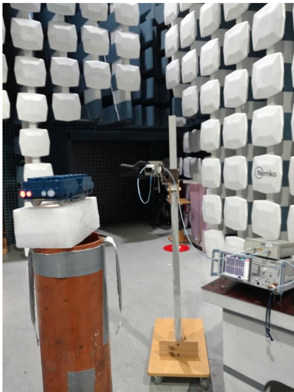
Radiated Emissions 18 – 26 GHz, device in XY-orientation. Antenna, preamplifier and spectrum analyser in background
