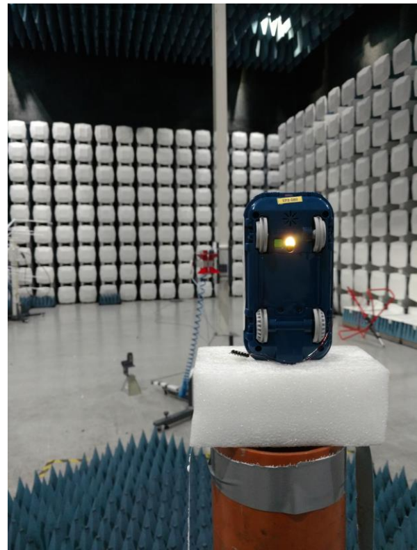
Radiated Emissions 1 – 18 GHz from device, device in YZ-orientation
