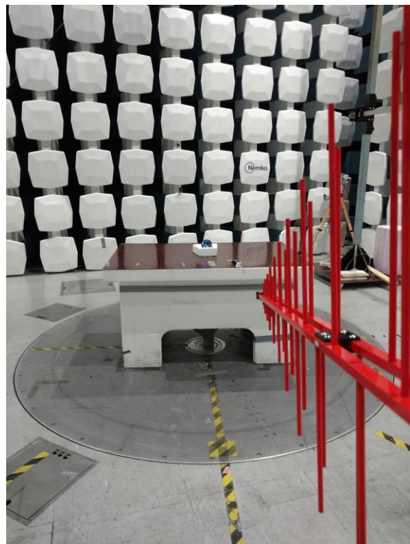
Radiated Emissions 30 – 1000 MHz from antenna
