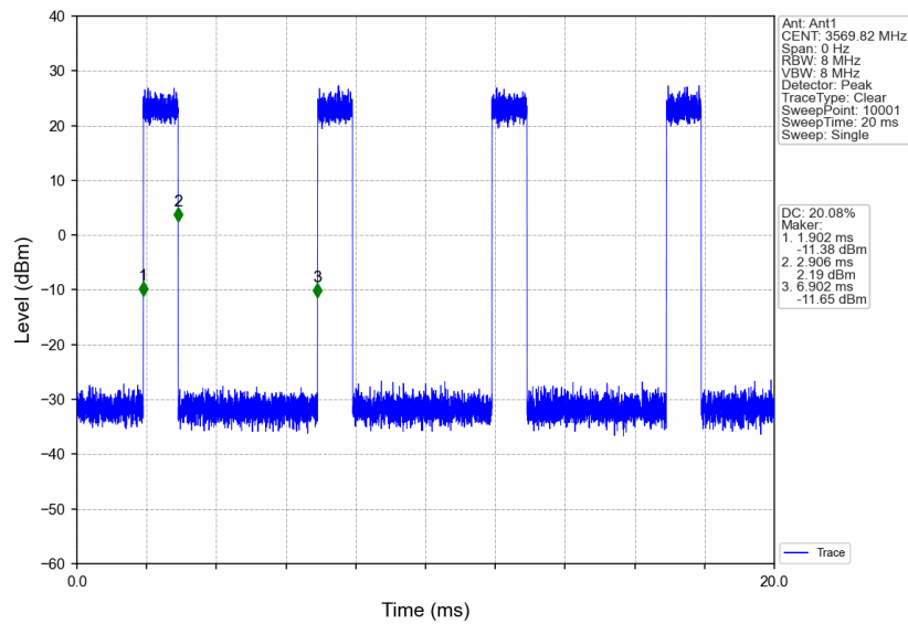
n48_30kHz_SISO_NTNV_40MHz_CP-OFDM_16_QAM_3570MHz_Inner_Full
