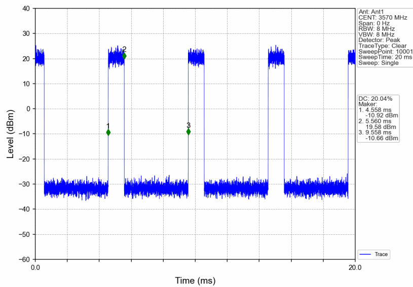
n48_30kHz_SISO_NTNV_40MHz_CP-OFDM QPSK_3570MHz_Inner_Full
