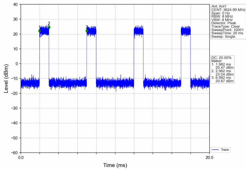
n48_30kHz_SISO_NTNV_40MHz_CP-OFDM QPSK_3624.99MHz_Inner_Full
