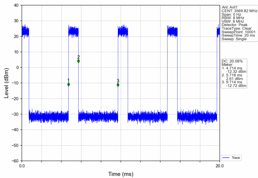
n48_30kHz_SISO_NTNV_40MHz_CP-OFDM QPSK_3570MHz_Inner_Full
