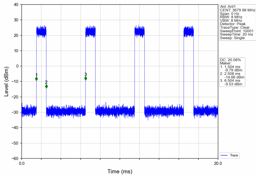
n48_30kHz_SISO_NTNV_40MHz_CP-OFDM QPSK_3679.98MHz_Inner_Full
