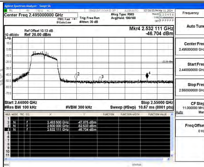
11N20SISO_Ant_High_2462
