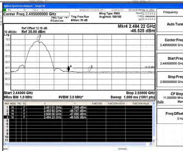
11B_Ant_High_2462_Peak
