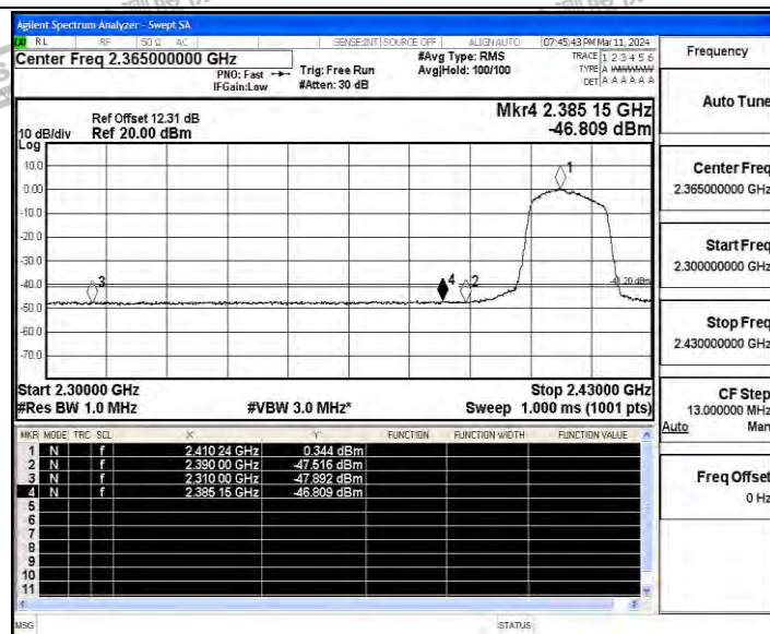
11G_Ant_Low_2412_Peak
