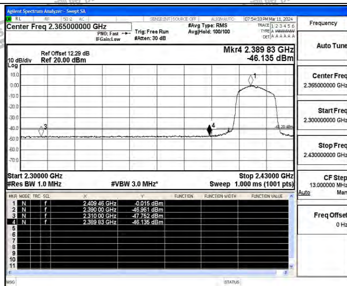
11N20SISO_Ant_Low_2412_Peak
