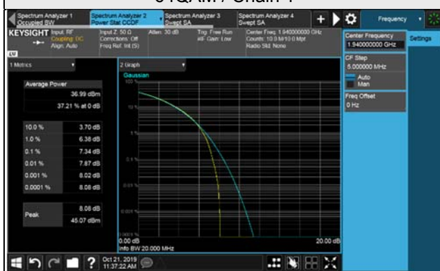
64QAM / Chain 1
