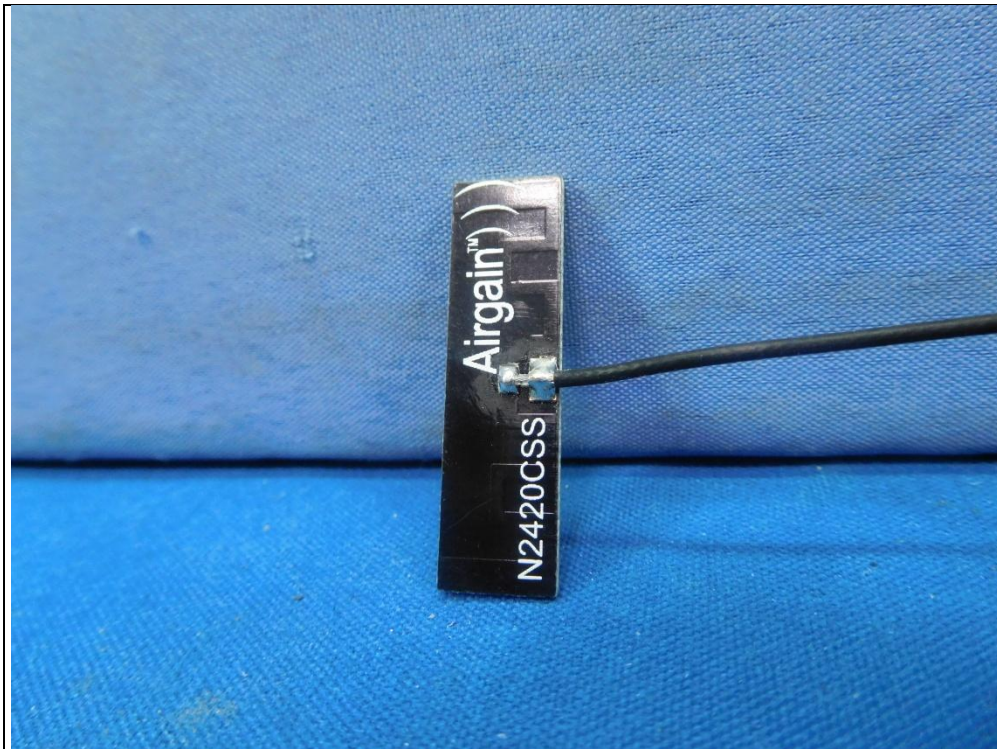
2.4GHz Antenna -2
