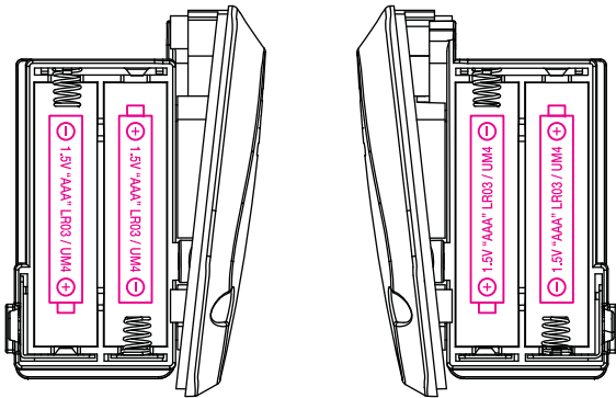
LEFT VIEW RIGHT VIEW BATTERY COMPARTMENT
