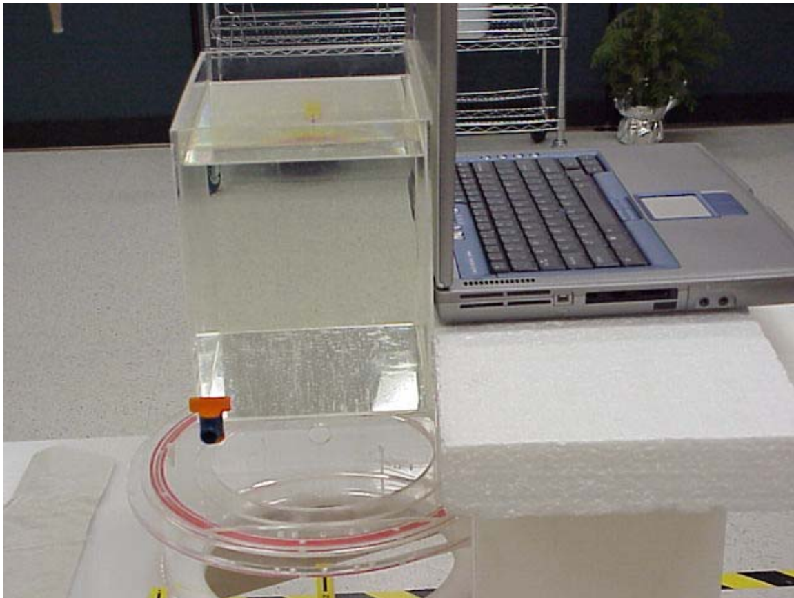
Photo 7. Left antenna bystander position
