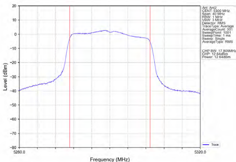
802.11ac(VHT20)_MCH_5300MHz_Ant2_NTNV
