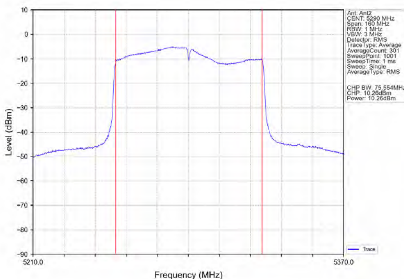
802.11ac(VHT80)_MCH_5290MHz_Ant2_NTNV
