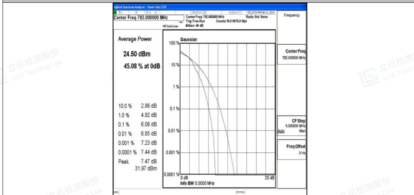
Band13-5MHz-16QAM-23230-25RB#0-PASS
