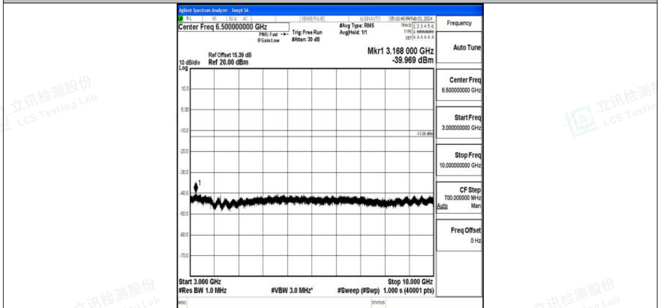
Band13_5MHz_16QAM_23205_1RB#0_3000~10000_3000~10000
