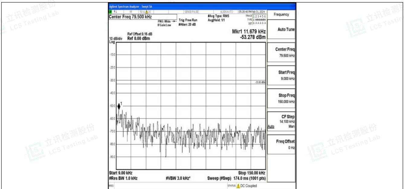
Band13_10MHz_QPSK_23230_1RB#0_0.009~0.15_0.009~0.15
