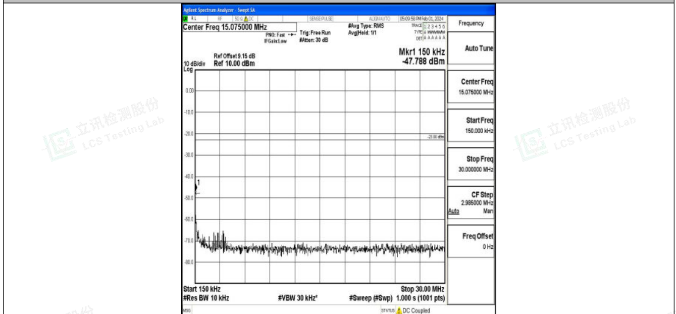
Band13_5MHz_QPSK_23205_1RB#0_0.15~30_0.15~30
