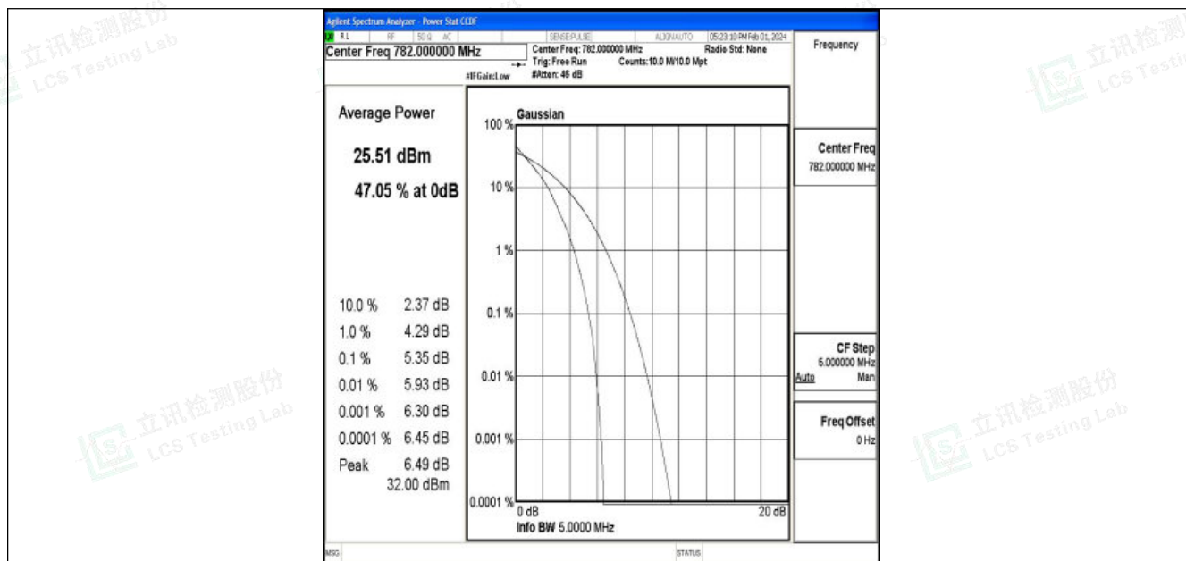
Band13-5MHz-QPSK-23230-25RB#0-PASS
