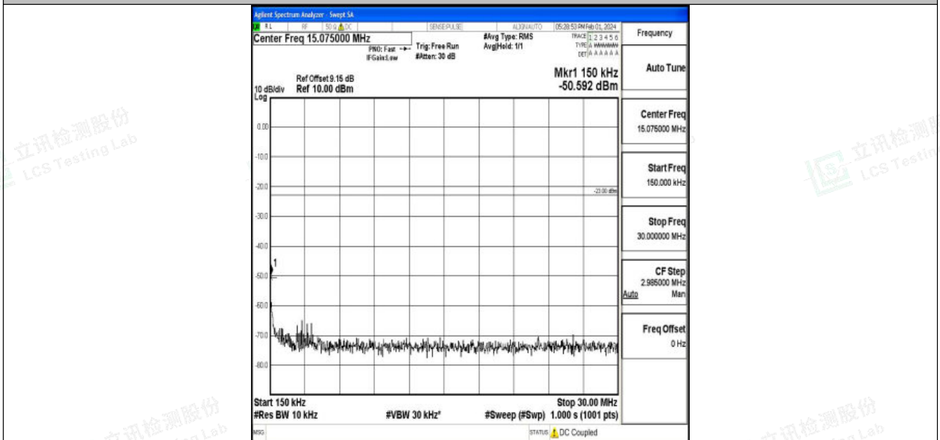
Band13_10MHz_QPSK_23230_1RB#0_0.15~30_0.15~30
