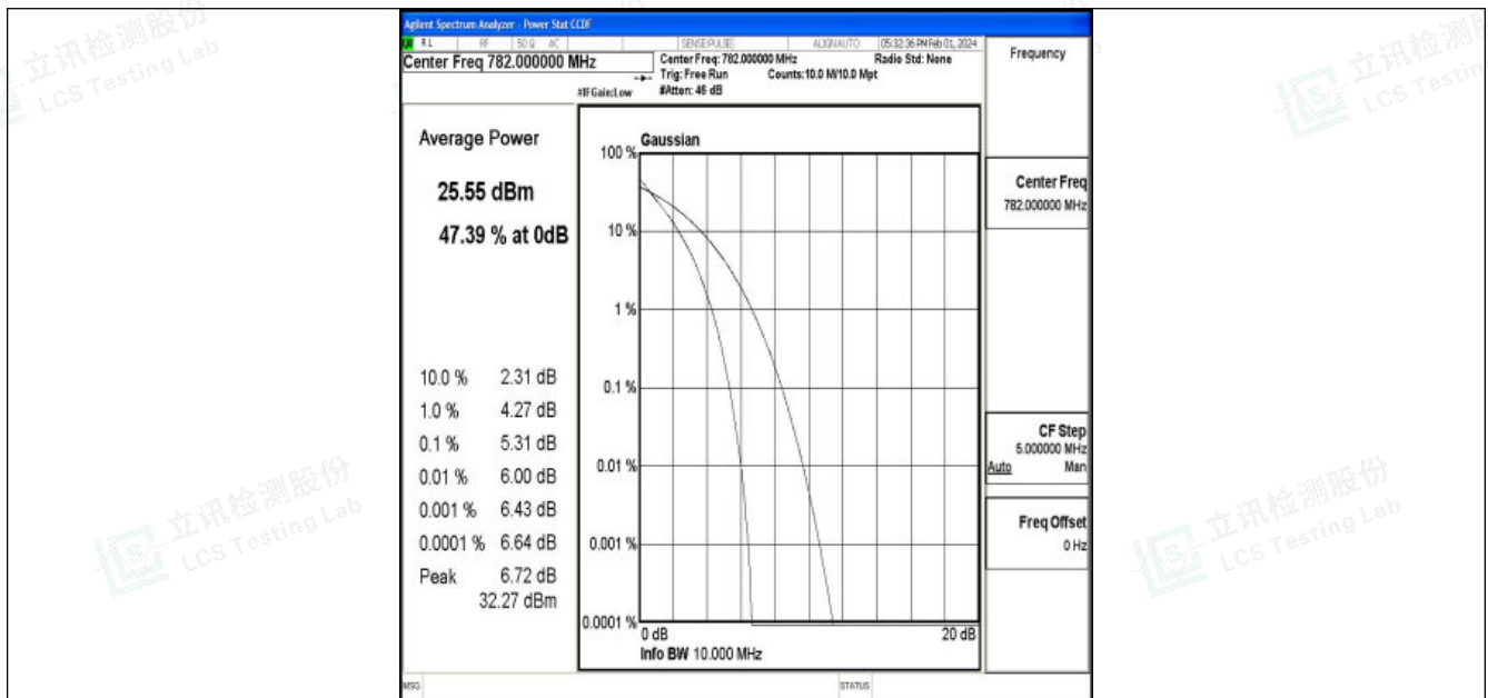
Band13-10MHz-QPSK-23230-50RB#0-PASS
