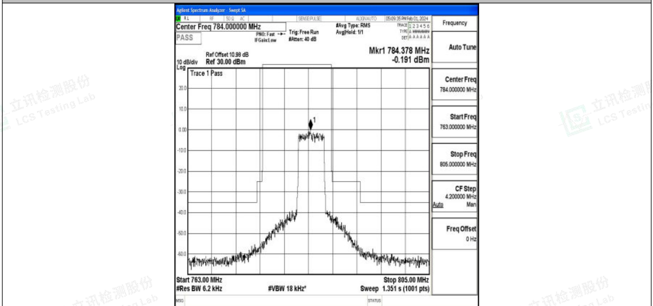
Band13_5MHz_QPSK_23255_25RB#0
