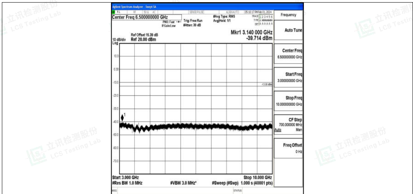
Band13_5MHz_QPSK_23205_1RB#0_3000~10000_3000~10000
