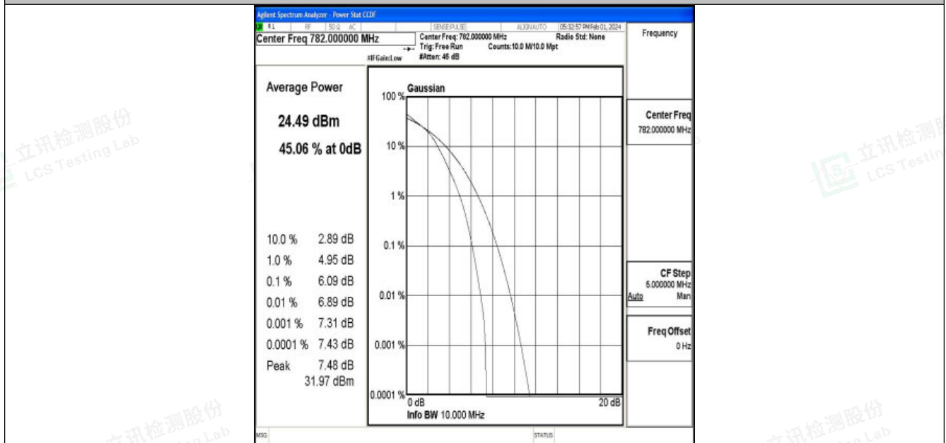
Band13-10MHz-16QAM-23230-50RB#0-PASS
