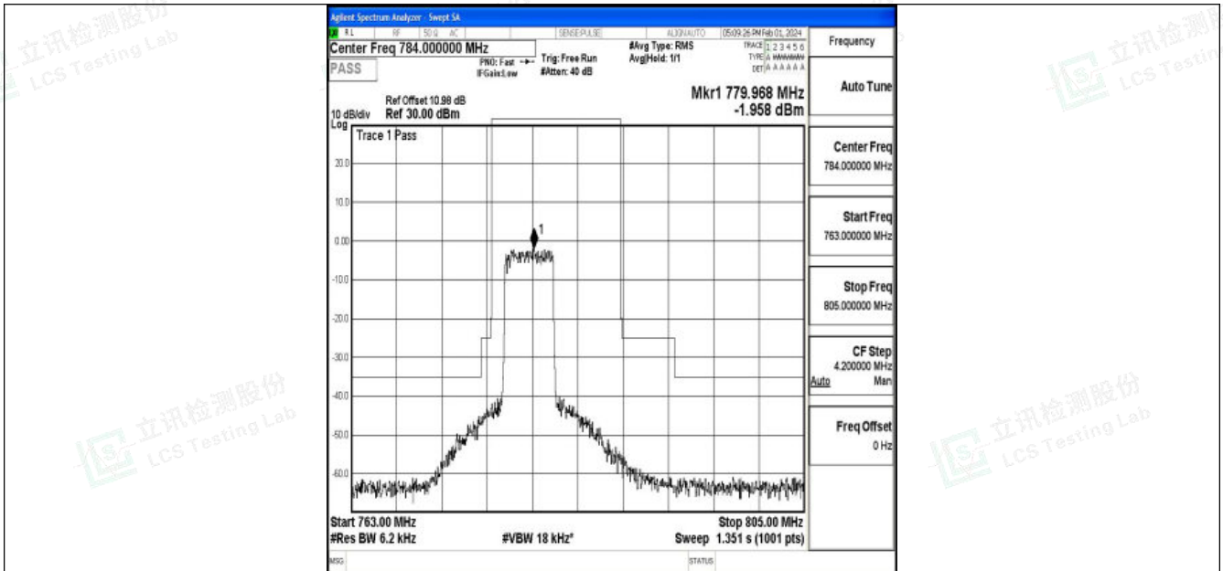
Band13_5MHz_16QAM_23205_25RB#0
