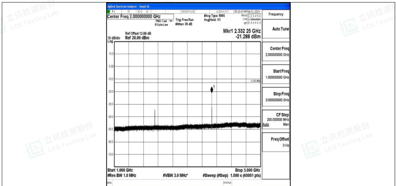
Band13_5MHz_16QAM_23205_1RB#0_1000~3000_1000~3000
