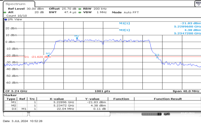
11AX20SISO_Ant1_5240
