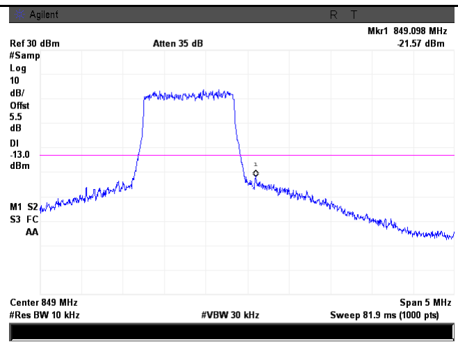
LTE Band 5 - High Channel QPSK-1.4
