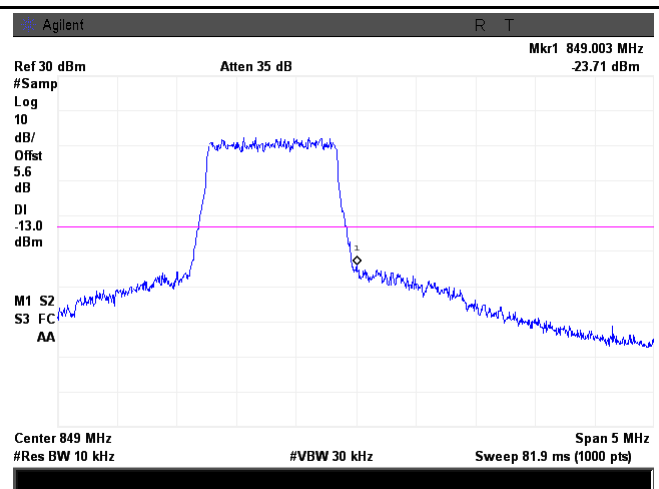
LTE Band 5 - High Channel 16QAM-1.4
