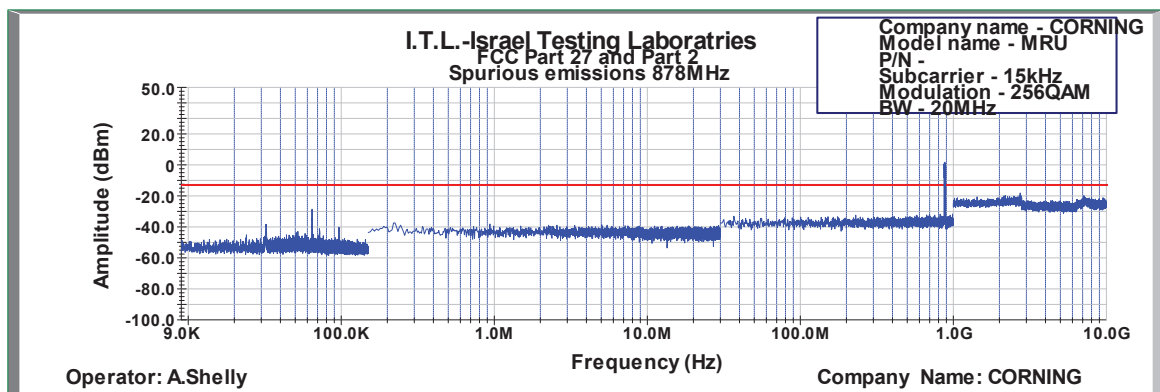
Figure 621: Spurious Emissions at Antenna Terminal 256QAM 20MHz B.W.; 878.0MHz, 15kHz
