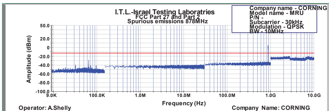
Figure 648: Spurious Emissions at Antenna Terminal QPSK 10MHz B.W.; 878.0MHz, 30kHz
