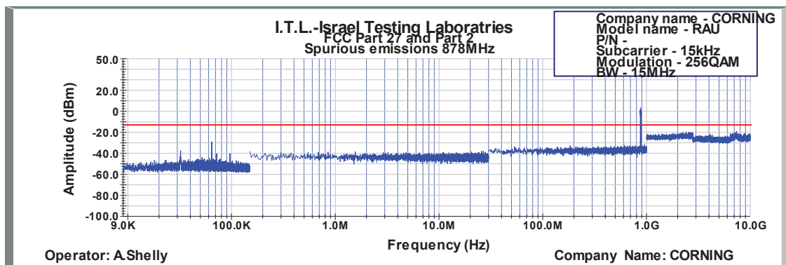
Figure 612: Spurious Emissions at Antenna Terminal 256QAM 15MHz B.W.; 878.0MHz, 15kHz
