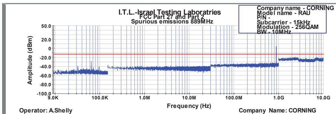
Figure 604: Spurious Emissions at Antenna Terminal 256QAM 10MHz B.W.; 889.0MHz, 15kHz
