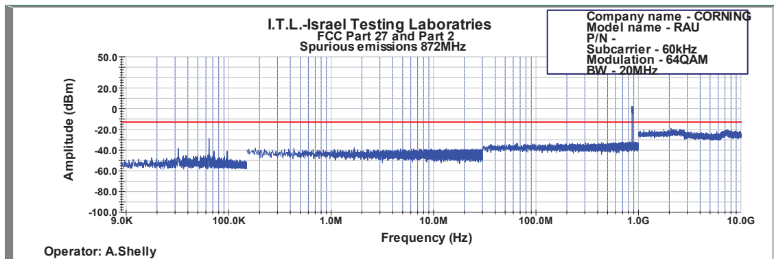
Figure 584: Spurious Emissions at Antenna Terminal 64QAM 20MHz B.W.; 872.0MHz, 60kHz
