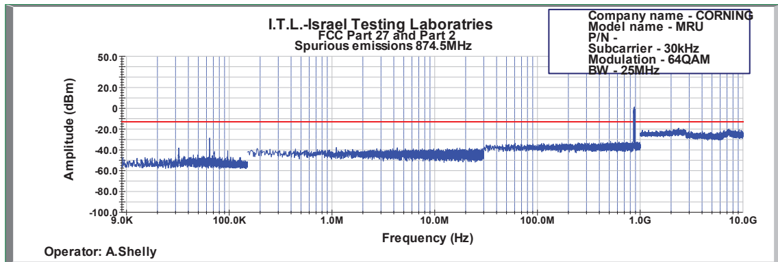
Figure 590: Spurious Emissions at Antenna Terminal 64QAM 25MHz B.W.; 874.5MHz, 30kHz
