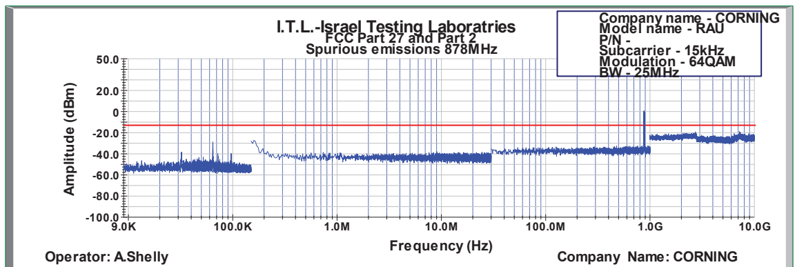
Figure 588: Spurious Emissions at Antenna Terminal 64QAM 25MHz B.W.; 878.0MHz, 15kHz
