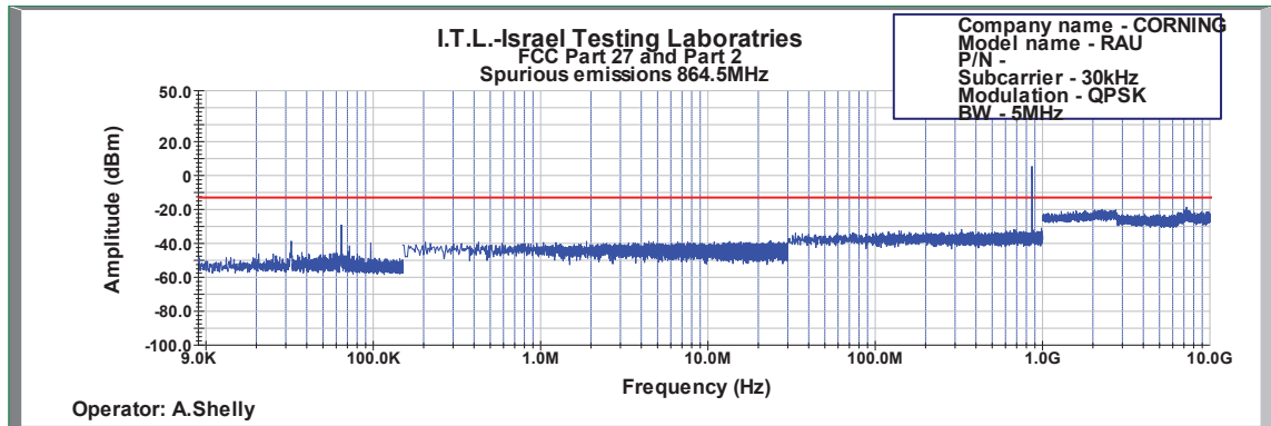
Figure 641: Spurious Emissions at Antenna Terminal QPSK 5MHz B.W.; 864.5MHz, 30kHz
