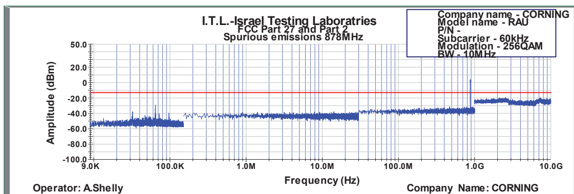
Figure 609: Spurious Emissions at Antenna Terminal 256QAM 10MHz B.W.; 878.0MHz, 60kHz
