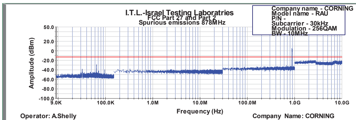
Figure 606: Spurious Emissions at Antenna Terminal 256QAM 10MHz B.W.; 878.0MHz, 30kHz
