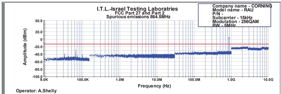
Figure 596: Spurious Emissions at Antenna Terminal 256QAM 5MHz B.W.; 864.5MHz, 15kHz
