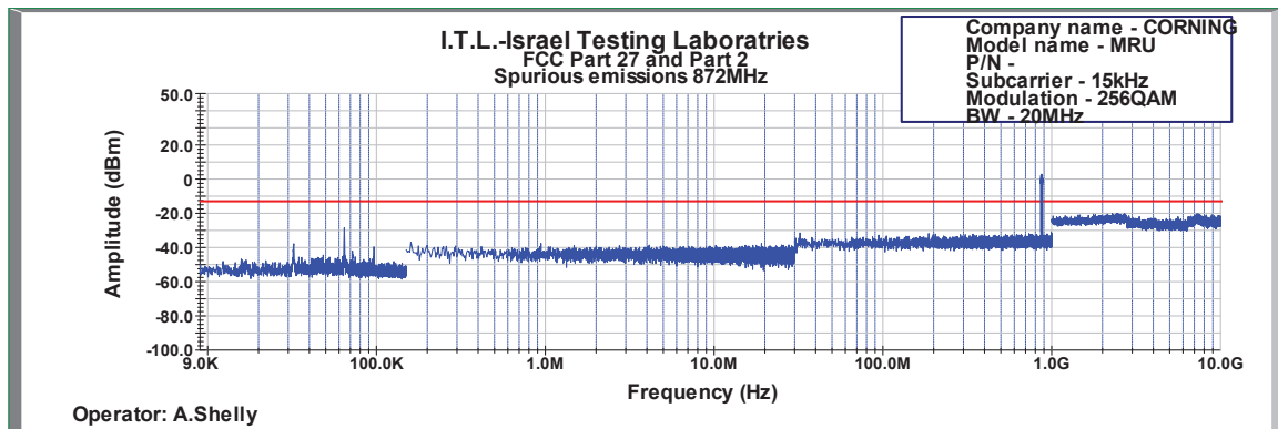
Figure 620: Spurious Emissions at Antenna Terminal 256QAM 20MHz B.W.; 872.0MHz, 15kHz
