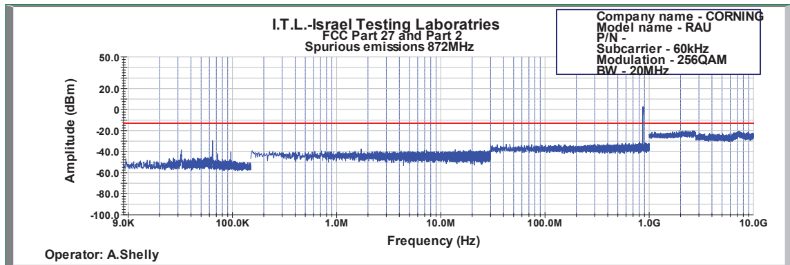
Figure 626: Spurious Emissions at Antenna Terminal 256QAM 20MHz B.W.; 872.0MHz, 60kHz
