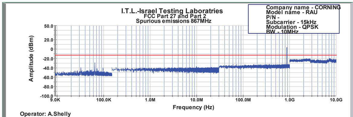
Figure 644: Spurious Emissions at Antenna Terminal QPSK 10MHz B.W.; 867.0MHz, 15kHz
