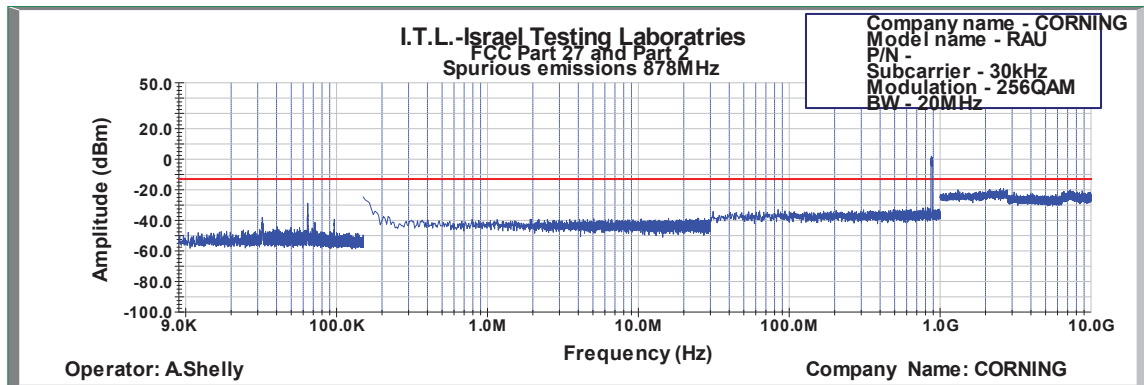
Figure 624: Spurious Emissions at Antenna Terminal 256QAM 20MHz B.W.; 878.0MHz, 30kHz
