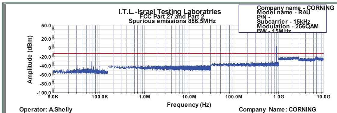
Figure 613: Spurious Emissions at Antenna Terminal 256QAM 15MHz B.W.; 886.5MHz, 15kHz
