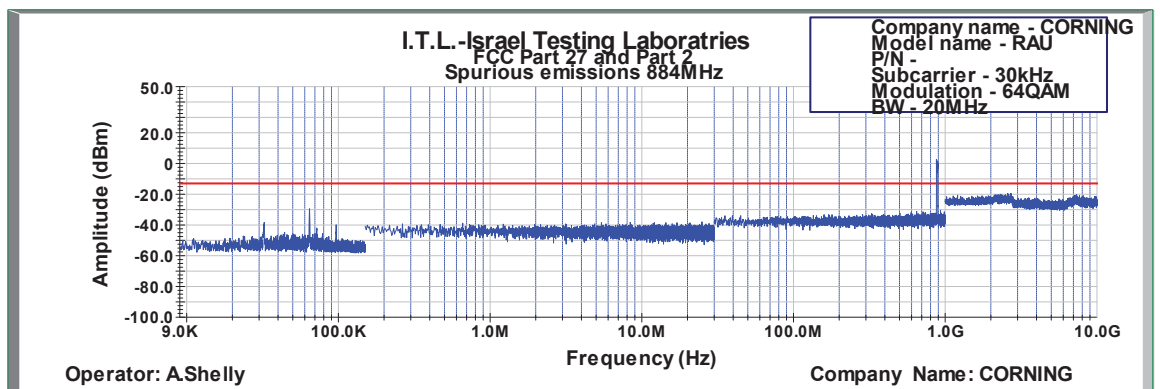
Figure 583: Spurious Emissions at Antenna Terminal 64QAM 20MHz B.W.; 884.0MHz, 30kHz
