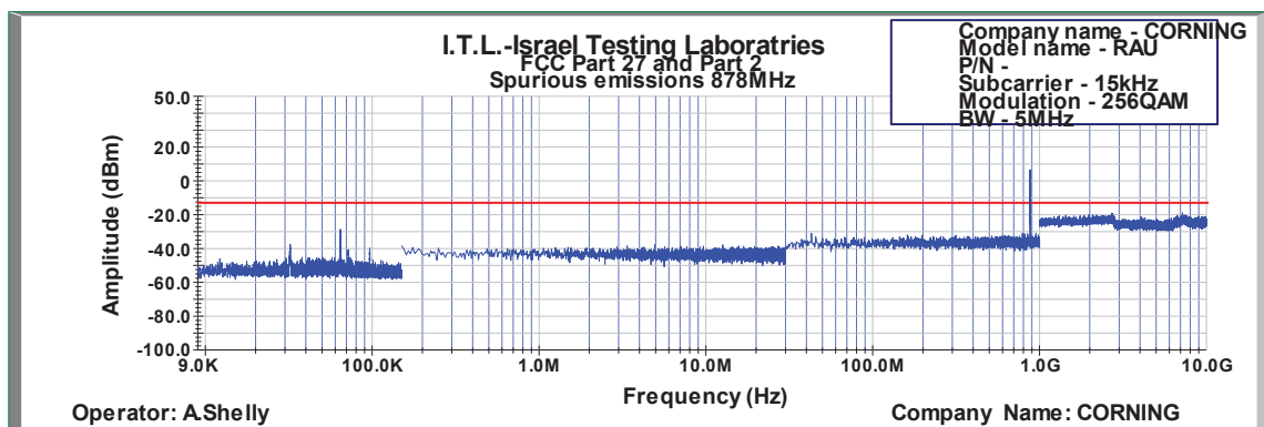
Figure 597: Spurious Emissions at Antenna Terminal 256QAM 5MHz B.W.; 878.0MHz, 15kHz
