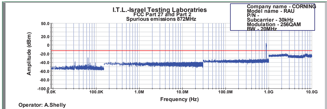
Figure 623: Spurious Emissions at Antenna Terminal 256QAM 20MHz B.W.; 872.0MHz, 30kHz
