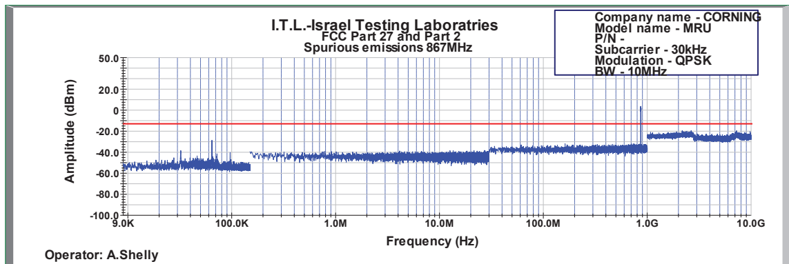
Figure 647: Spurious Emissions at Antenna Terminal QPSK 10MHz B.W.; 867.0MHz, 30kHz
