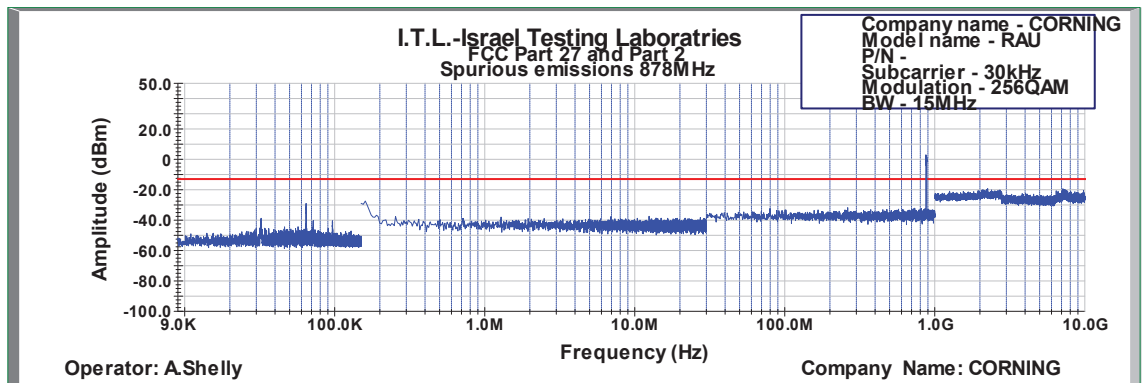
Figure 615: Spurious Emissions at Antenna Terminal 256QAM 15MHz B.W.; 878.0MHz, 30kHz
