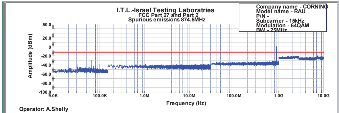
Figure 587: Spurious Emissions at Antenna Terminal 64QAM 25MHz B.W.; 874.5MHz, 15kHz
