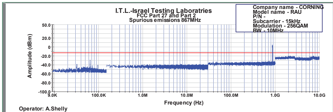
Figure 602: Spurious Emissions at Antenna Terminal 256QAM 10MHz B.W.; 867.0MHz,15kHz
