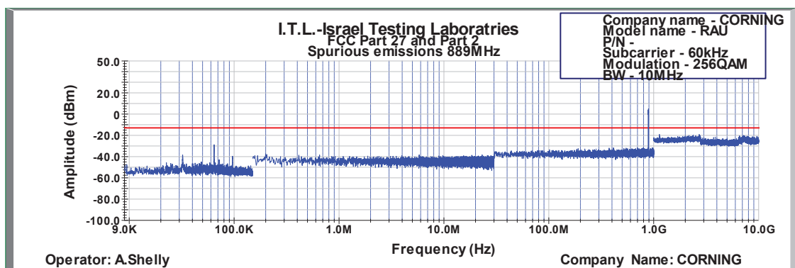
Figure 610: Spurious Emissions at Antenna Terminal 256QAM 10MHz B.W.; 889.0MHz, 60kHz
