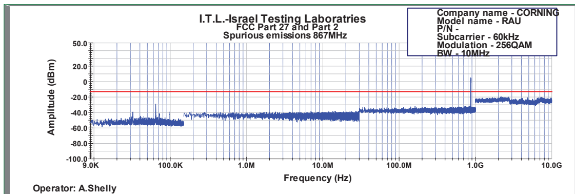
Figure 608: Spurious Emissions at Antenna Terminal 256QAM 10MHz B.W.; 867.0MHz, 60kHz
