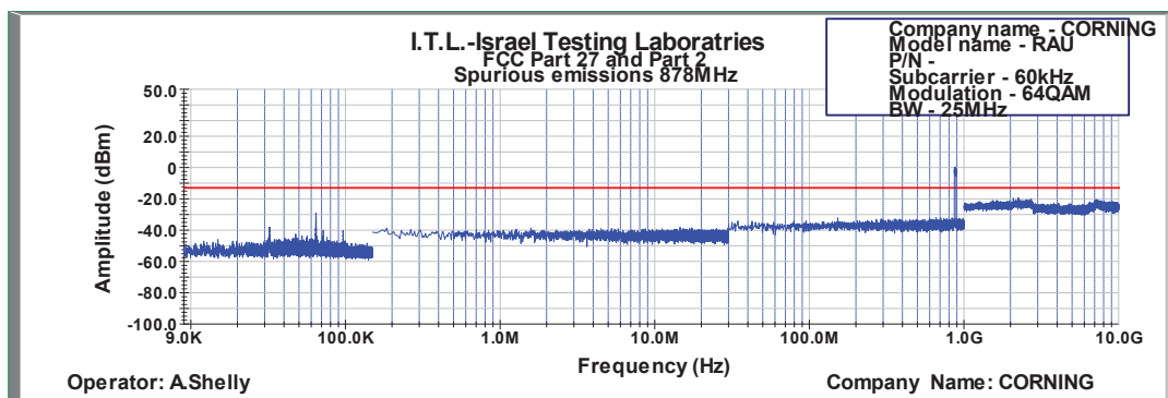
Figure 594: Spurious Emissions at Antenna Terminal 64QAM 25MHz B.W.; 878MHz, 60kHz
