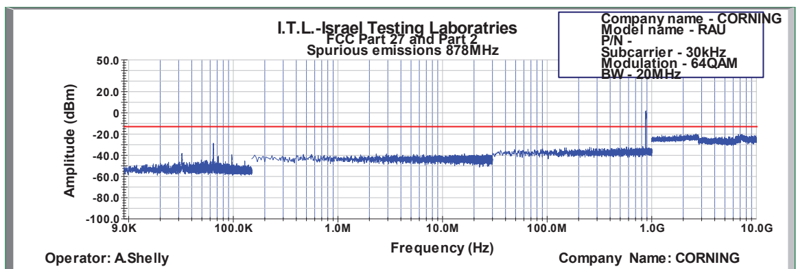
Figure 582: Spurious Emissions at Antenna Terminal 64QAM 20MHz B.W.; 878.0MHz, 30kHz
