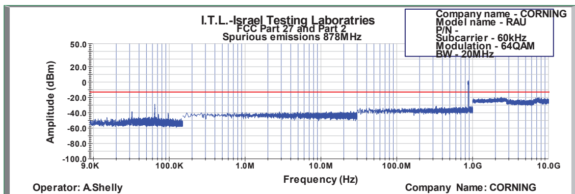
Figure 585: Spurious Emissions at Antenna Terminal 64QAM 20MHz B.W.; 878.0MHz, 60kHz
