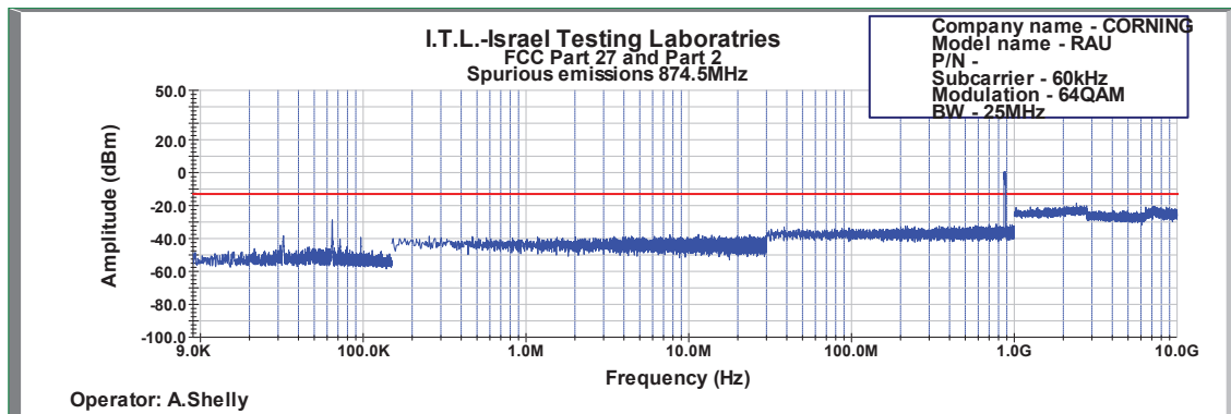
Figure 593: Spurious Emissions at Antenna Terminal 64QAM 25MHz B.W.; 874.5MHz, 60kHz
