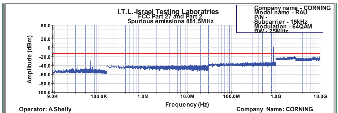
Figure 589: Spurious Emissions at Antenna Terminal 64QAM 25MHz B.W.; 881.5MHz, 15kHz
