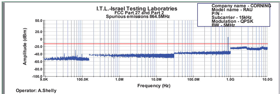
Figure 638: Spurious Emissions at Antenna Terminal QPSK 5MHz B.W.; 864.5MHz, 15kHz
