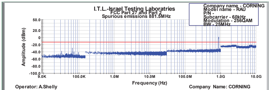
Figure 637: Spurious Emissions at Antenna Terminal 256QAM 25MHz B.W.; 881.5MHz, 60kHz
