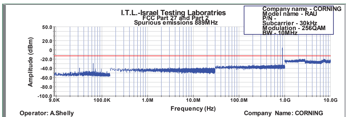
Figure 607: Spurious Emissions at Antenna Terminal 256QAM 10MHz B.W.; 889.0MHz, 30kHz
