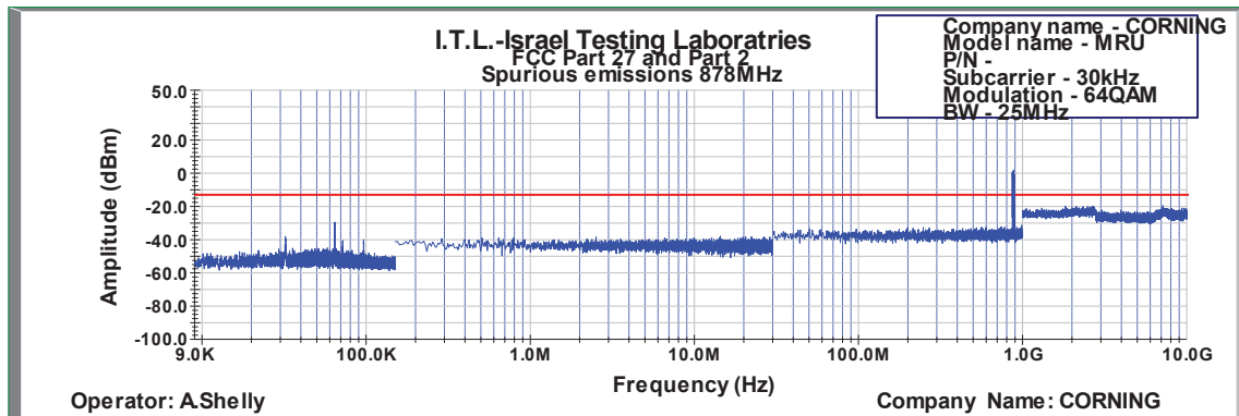
Figure 591: Spurious Emissions at Antenna Terminal 64QAM 25MHz B.W.; 878.0MHz, 30kHz
