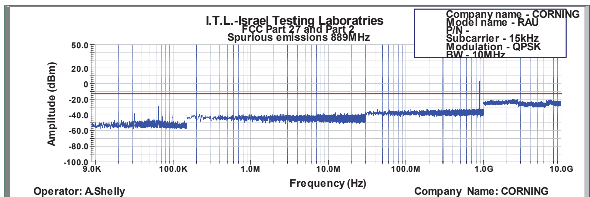
Figure 646: Spurious Emissions at Antenna Terminal QPSK 10MHz B.W.; 889.0MHz, 15kHz
