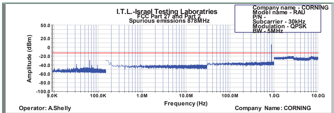
Figure 642: Spurious Emissions at Antenna Terminal QPSK 5MHz B.W.; 878.0MHz, 30kHz
