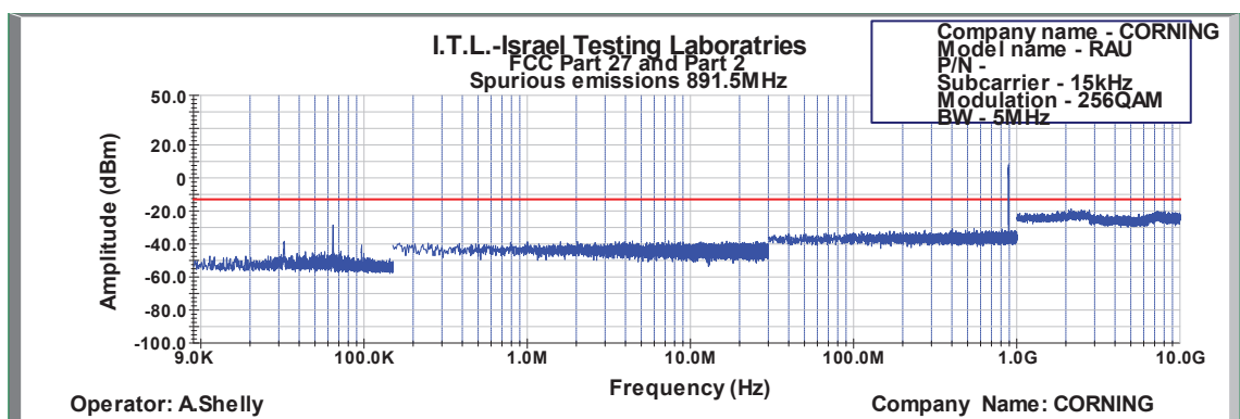
Figure 598: Spurious Emissions at Antenna Terminal 256QAM 5MHz B.W.; 891.5MHz, 15kHz
