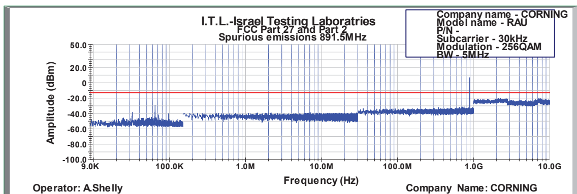
Figure 601: Spurious Emissions at Antenna Terminal 256QAM 5MHz B.W.; 891.5MHz, 30kHz
