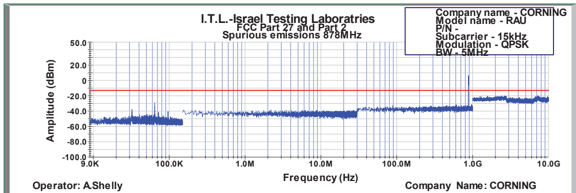
Figure 639: Spurious Emissions at Antenna Terminal QPSK 5MHz B.W.; 878.0MHz, 15kHz
