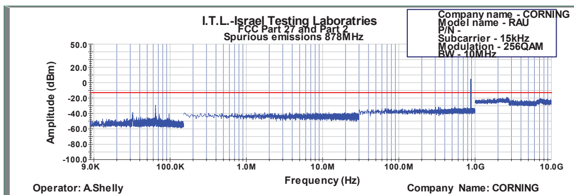
Figure 603: Spurious Emissions at Antenna Terminal 256QAM 10MHz B.W.; 878.0MHz, 15kHz
