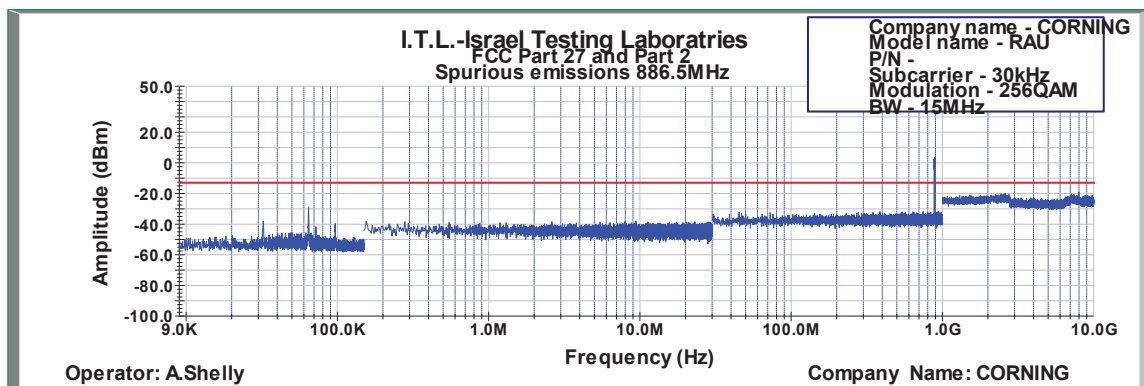
Figure 616: Spurious Emissions at Antenna Terminal 256QAM 15MHz B.W.; 886.5MHz, 30kHz
