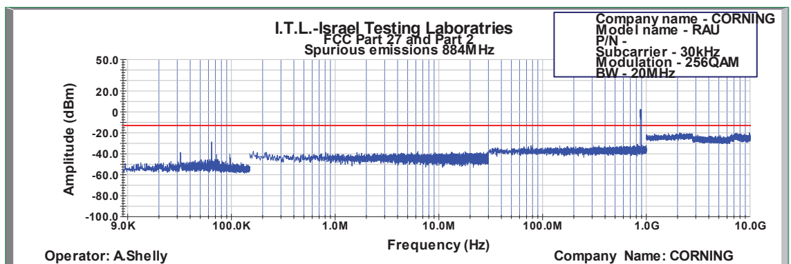
Figure 625: Spurious Emissions at Antenna Terminal 256QAM 20MHz B.W.; 884.0MHz, 30kHz
