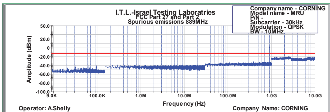
Figure 649: Spurious Emissions at Antenna Terminal QPSK 10MHz B.W.; 889.0MHz, 30kHz
