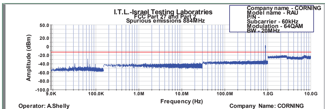
Figure 586: Spurious Emissions at Antenna Terminal 64QAM 20MHz B.W.; 884.0MHz, 60kHz
