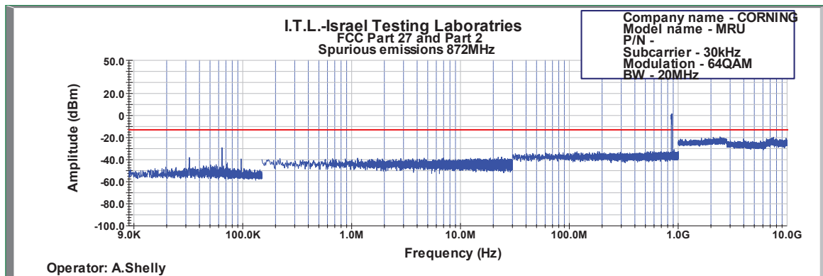
Figure 581: Spurious Emissions at Antenna Terminal 64QAM 20MHz B.W.; 872.0MHz, 30kHz
