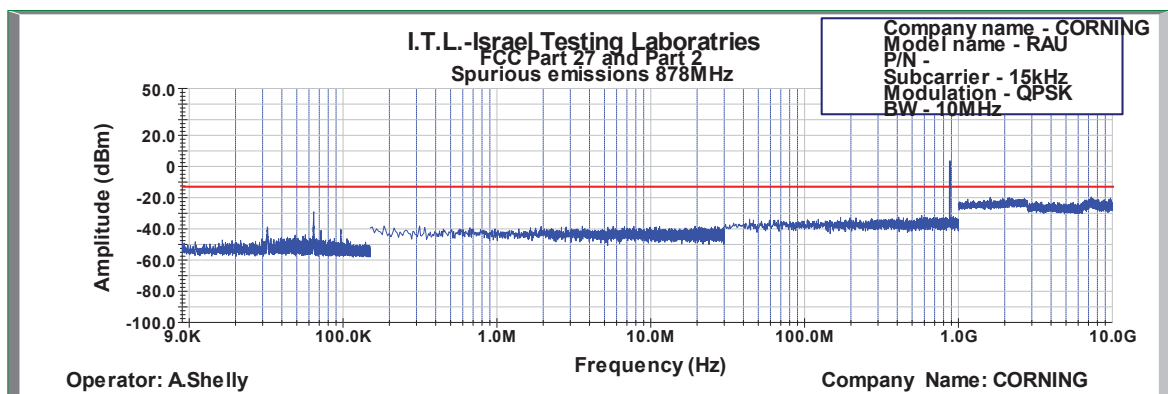
Figure 645: Spurious Emissions at Antenna Terminal QPSK 10MHz B.W.; 878.0MHz, 15kHz
