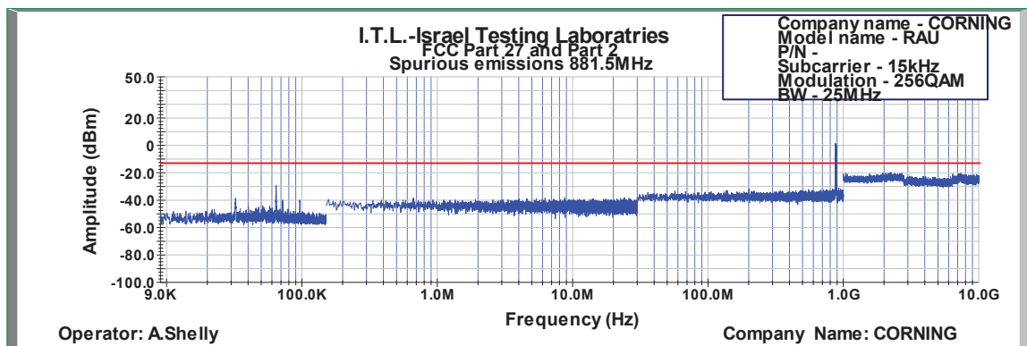
Figure 631: Spurious Emissions at Antenna Terminal 256QAM 25MHz B.W.; 881.5MHz, 15kHz
