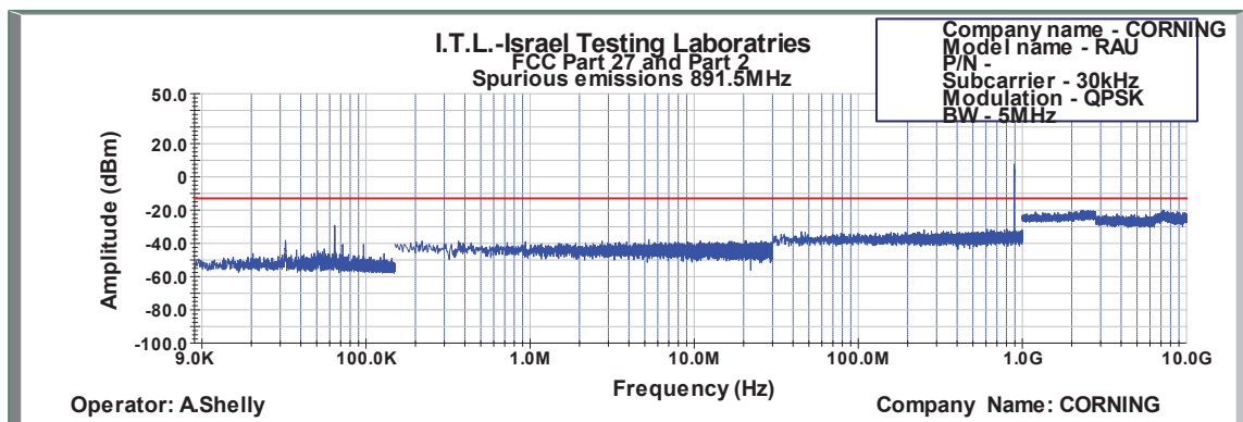
Figure 643: Spurious Emissions at Antenna Terminal QPSK 5MHz B.W.; 891.5MHz, 30kHz
