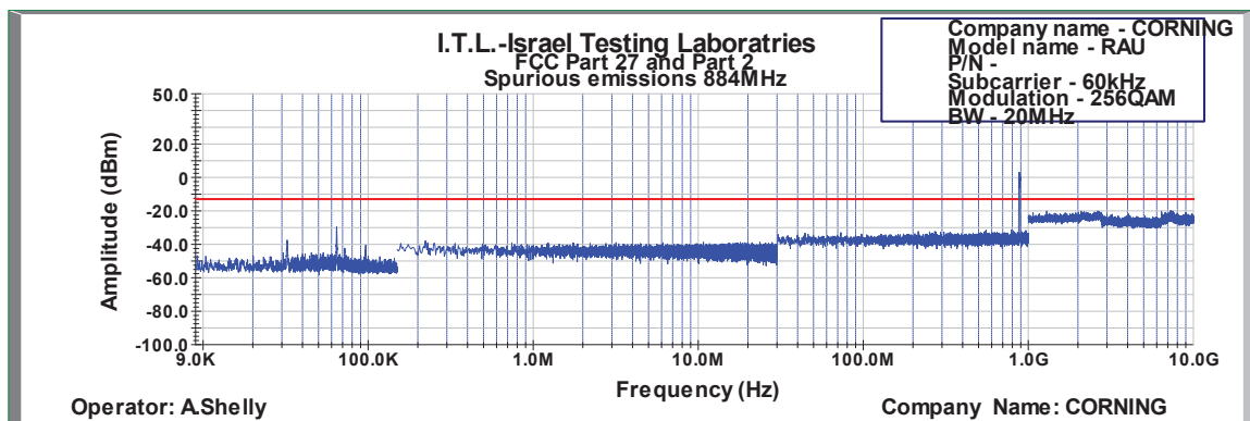
Figure 628: Spurious Emissions at Antenna Terminal 256QAM 20MHz B.W.; 884.0MHz, 60kHz
