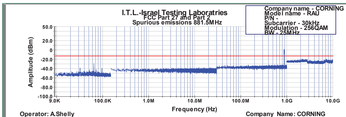
Figure 634: Spurious Emissions at Antenna Terminal 256QAM 25MHz B.W.; 881.5MHz, 30kHz
