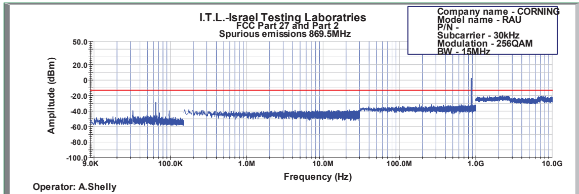
Figure 614: Spurious Emissions at Antenna Terminal 256QAM 15MHz B.W.; 869.5MHz, 30kHz
