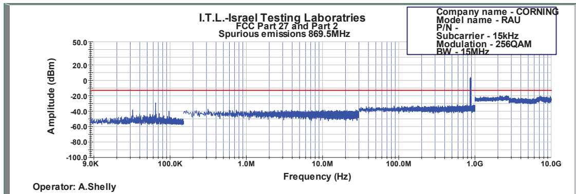
Figure 611: Spurious Emissions at Antenna Terminal 256QAM 15MHz B.W.; 869.5MHz, 15kHz
