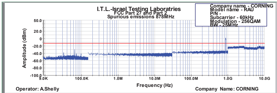
Figure 636: Spurious Emissions at Antenna Terminal 256QAM 25MHz B.W.; 878MHz, 60kHz
