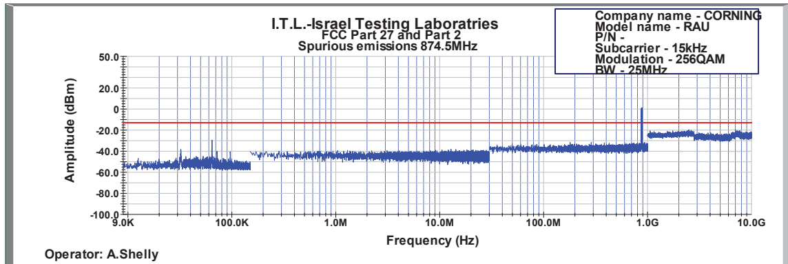
Figure 629: Spurious Emissions at Antenna Terminal 256QAM 25MHz B.W.; 874.5MHz, 15kHz
