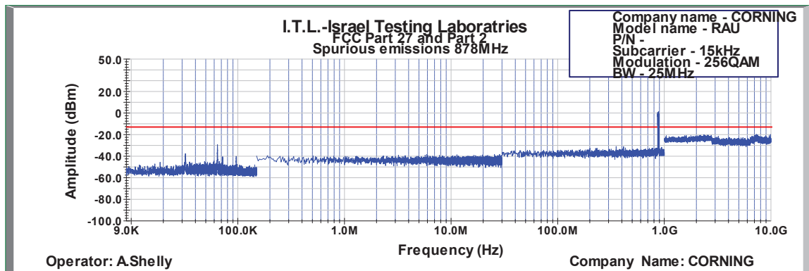
Figure 630: Spurious Emissions at Antenna Terminal 256QAM 25MHz B.W.; 878.0MHz, 15kHz
