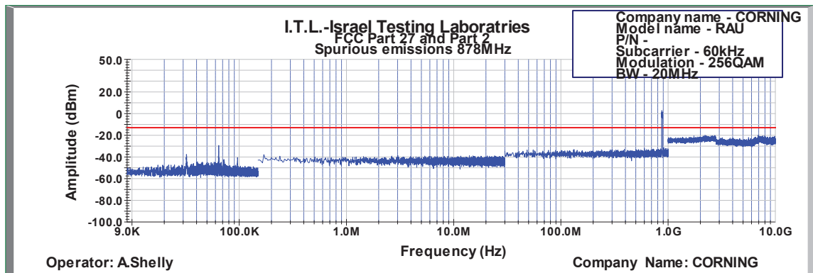
Figure 627: Spurious Emissions at Antenna Terminal 256QAM 20MHz B.W.; 878.0MHz, 60kHz
