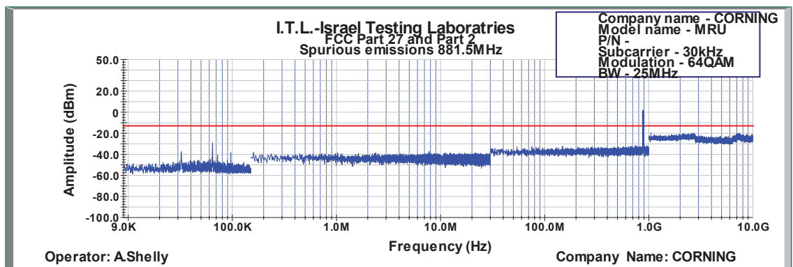
Figure 592: Spurious Emissions at Antenna Terminal 64QAM 25MHz B.W.; 881.5MHz, 30kHz
