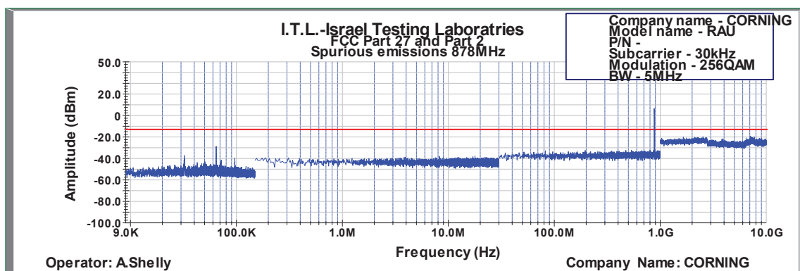
Figure 600: Spurious Emissions at Antenna Terminal 256QAM 5MHz B.W.; 878.0MHz, 30kHz
