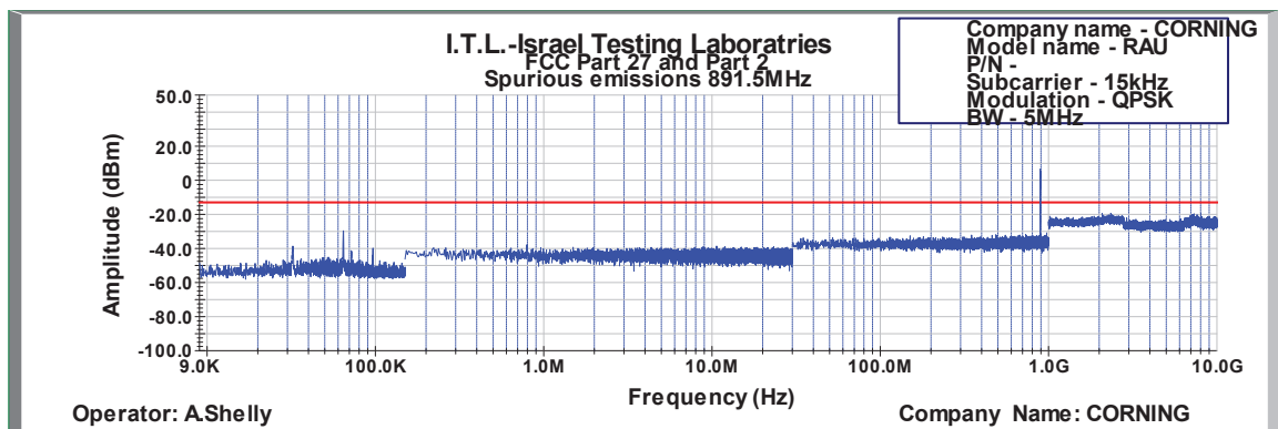
Figure 640: Spurious Emissions at Antenna Terminal QPSK 5MHz B.W.; 891.5MHz, 15kHz
