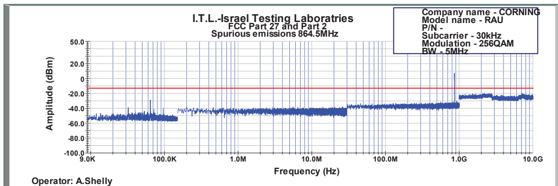
Figure 599: Spurious Emissions at Antenna Terminal 256QAM 5MHz B.W.; 864.5MHz, 30kHz
