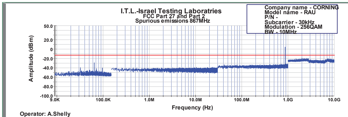
Figure 605: Spurious Emissions at Antenna Terminal 256QAM 10MHz B.W.; 867.0MHz, 30kHz
