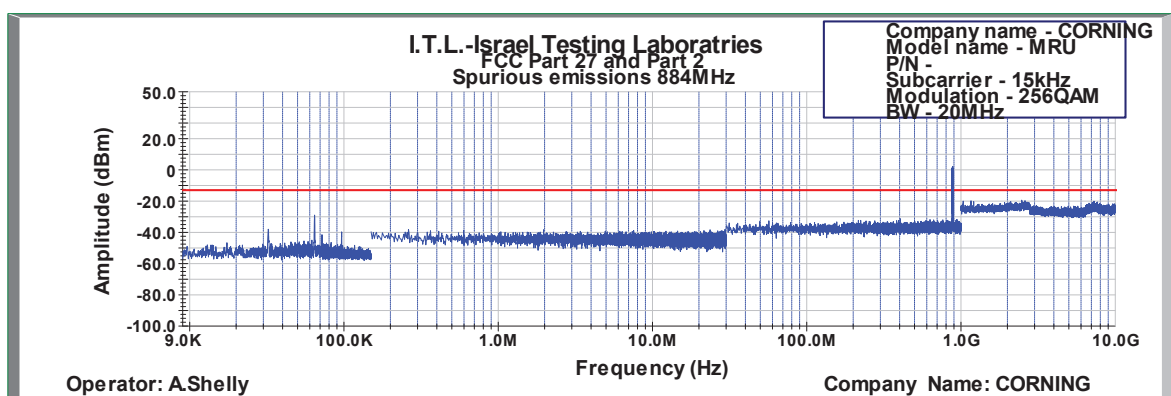
Figure 622: Spurious Emissions at Antenna Terminal 256QAM 20MHz B.W.; 884.0MHz, 15kHz
