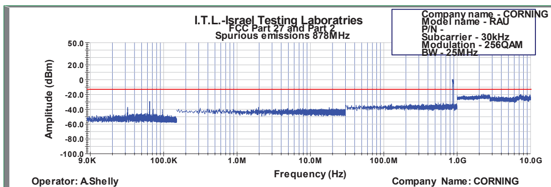
Figure 633: Spurious Emissions at Antenna Terminal 256QAM 25MHz B.W.; 878.0MHz, 30kHz
