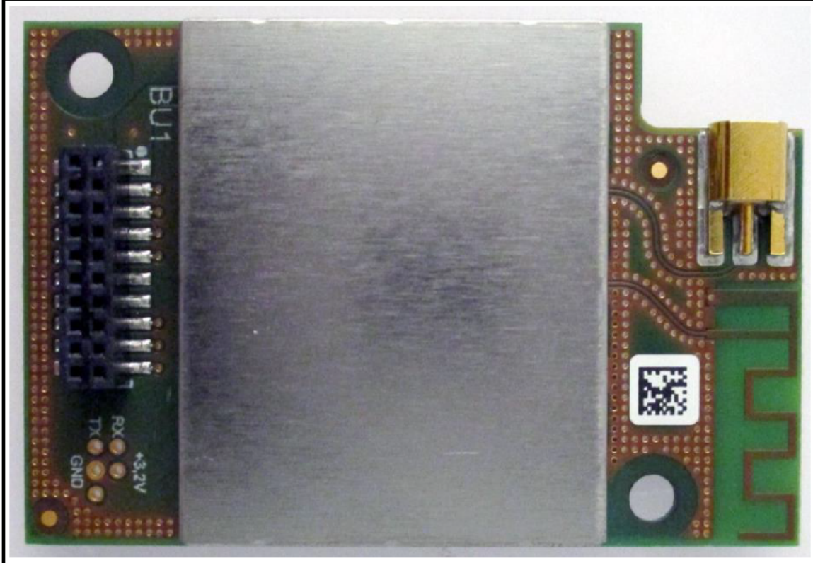
TC242C01_EUT7.2 – conducted sample top view
