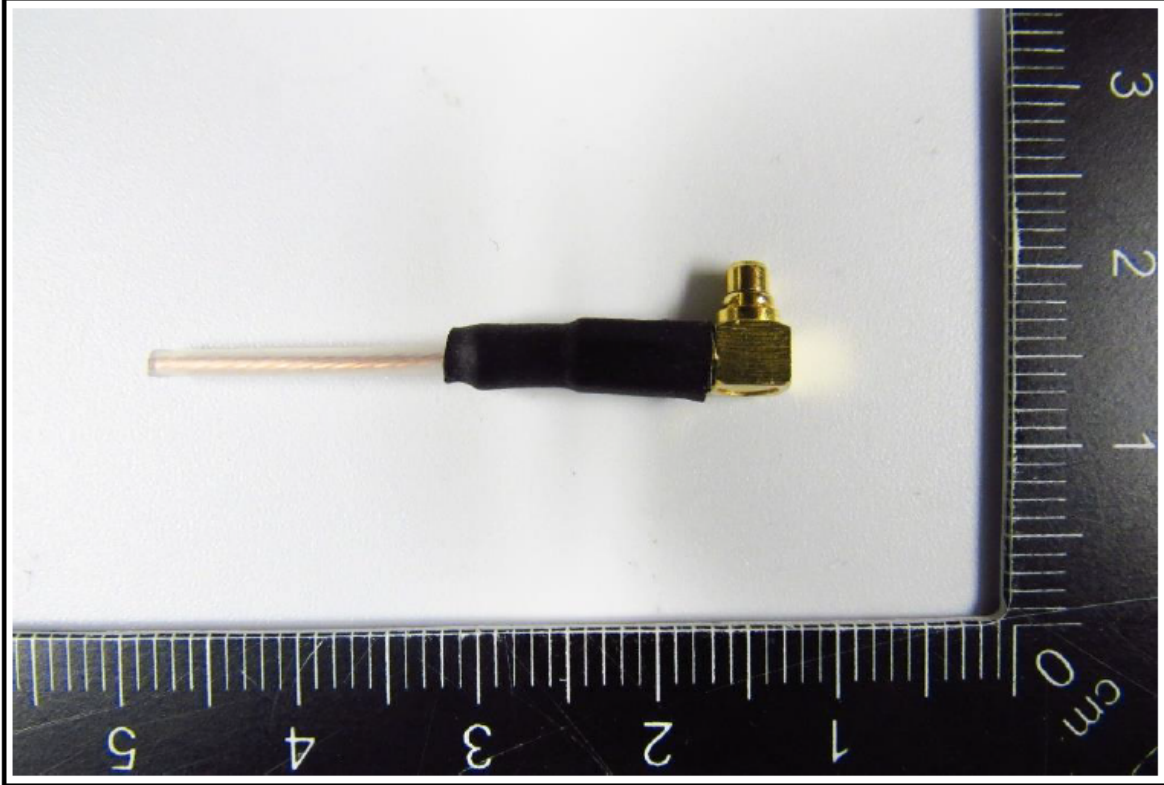
AA080004 (Monopole 35mm)
