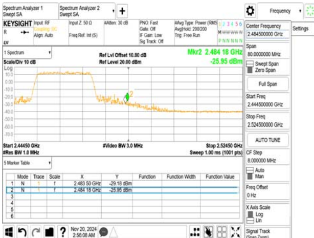
802.11ax_20MHz_2462MHz_RU106_54
