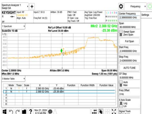
802.11ax_20MHz_2417MHz_RU106_53
