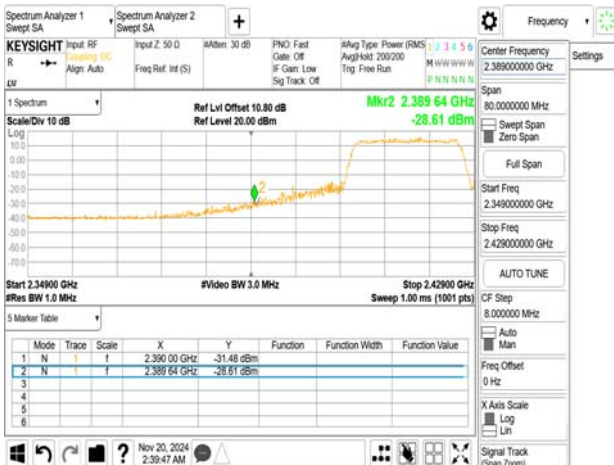
802.11ax_20MHz_2417MHz_RU106_53
