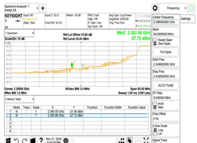
802.11ax_20MHz_2432MHz_RU106_53
