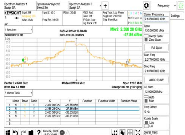
802.11ax_20MHz_2437MHz_RU106_54
