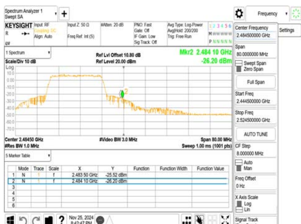
802.11ax_20MHz_2467MHz_RU242
