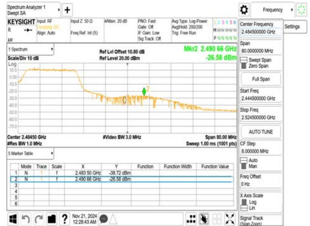
802.11ax_40MHz_2447MHz_RU484
