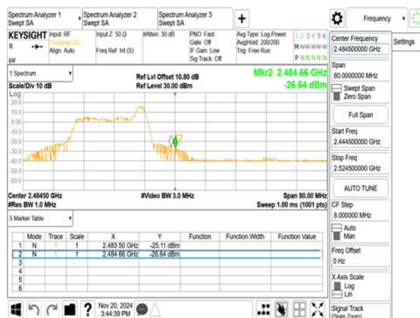
802.11ax_20MHz_2467MHz_RU52_40
