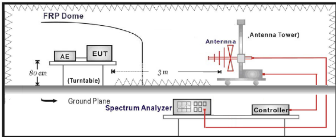
Radiated Spurious Measurement: 30MHz to 1GHz
