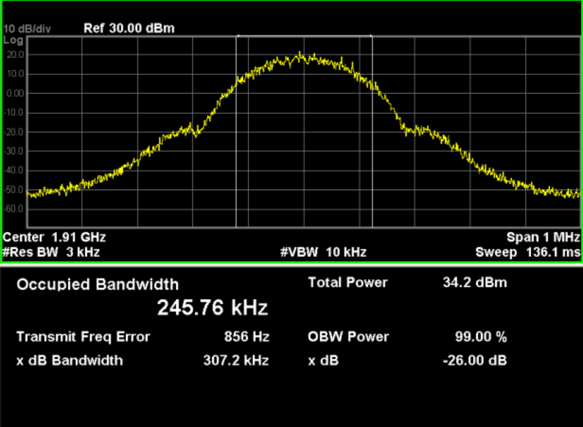
GSM1900 (EDGE 8 Link)
