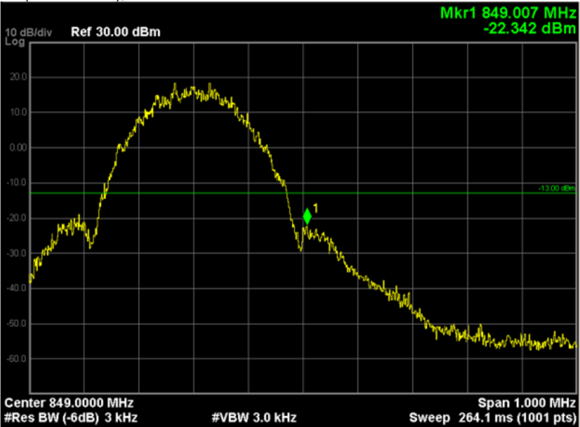
GSM850 (EDGE 8 Link), Channel 251
