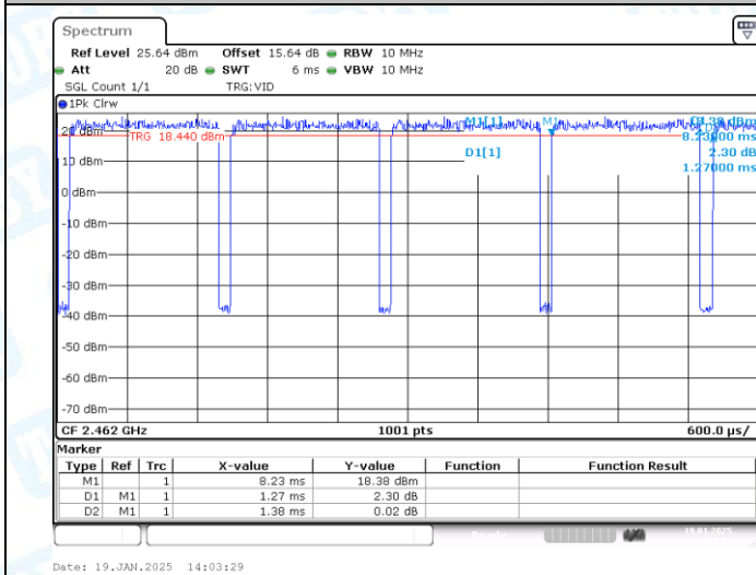
NTNV-11N20-CDD-Ant1-2462
