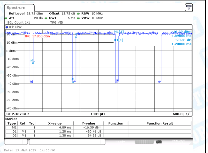
NTNV-11N20-CDD-Ant2-2437
