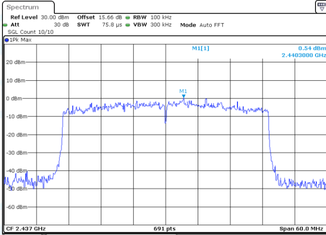
11AX40-CDD-Ant1-2437-0~Reference-PASS
