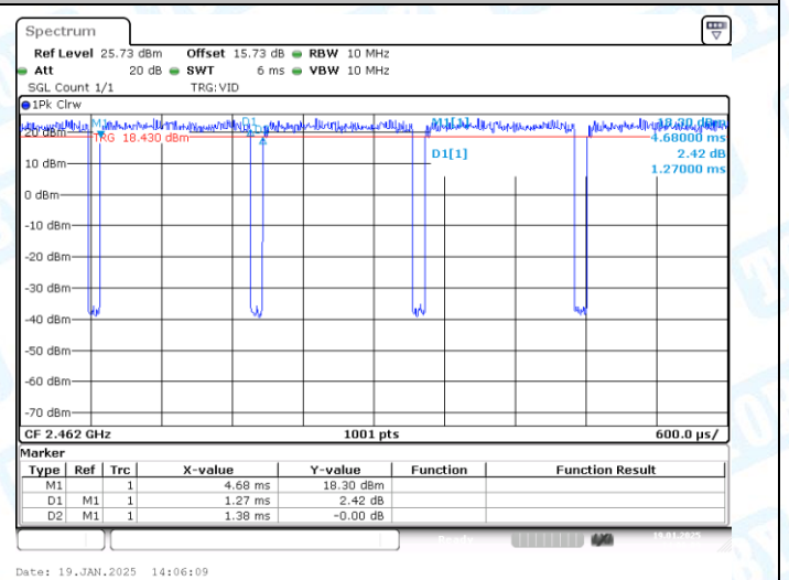
NTNV-11N20-CDD-Ant2-2462
