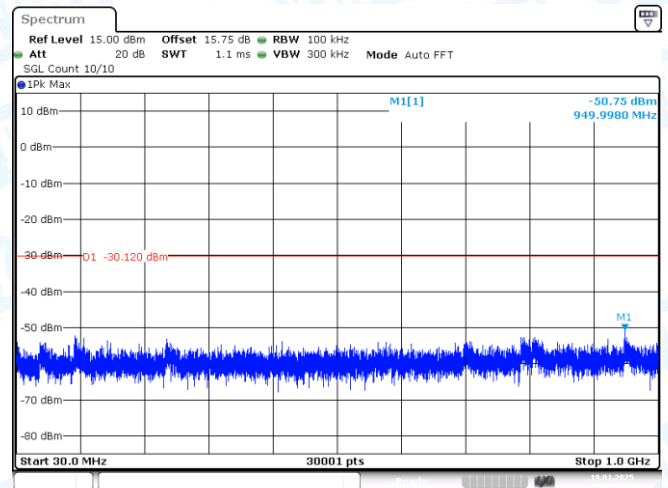
11AX40-CDD-Ant2-2437-0~Reference-PASS
