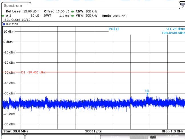
11AX40-CDD-Ant1-2437-0~Reference-PASS
