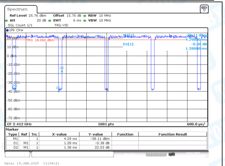
NTNV-11N20-CDD-Ant2-2412
