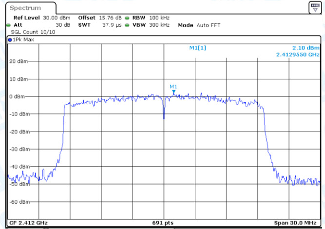
11AX20-CDD-Ant2-2412-0~Reference-PASS
