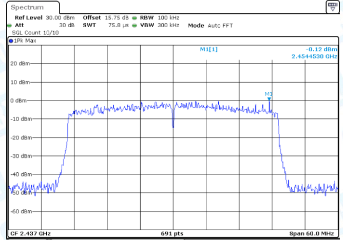
11AX40-CDD-Ant2-2437-0~Reference-PASS
