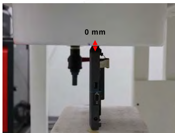
Fig.7 EUT Top side with optional battery to flat phantom
