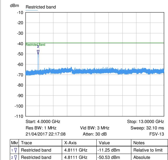
Ch 11: trace 4; 4000 - 13000 MHz
