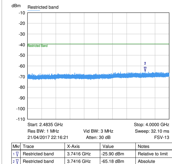
Ch 11: trace 3; 2483.5 - 4000 MHz
