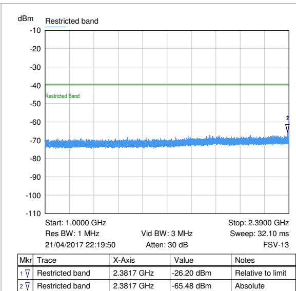
Ch 19: trace 2; 1000 - 2390 MHz
