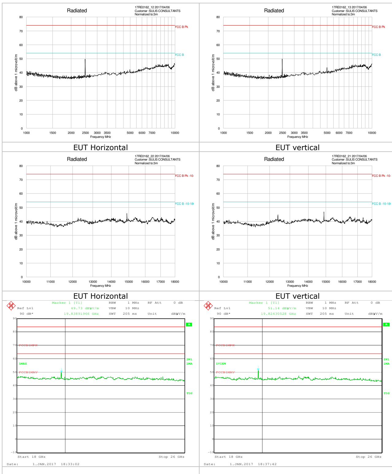
Figure 8: Radiated Spurious Emissions; Channel 26
