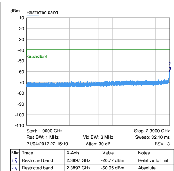
Ch 11: trace 2; 1000 - 2390 MHz
