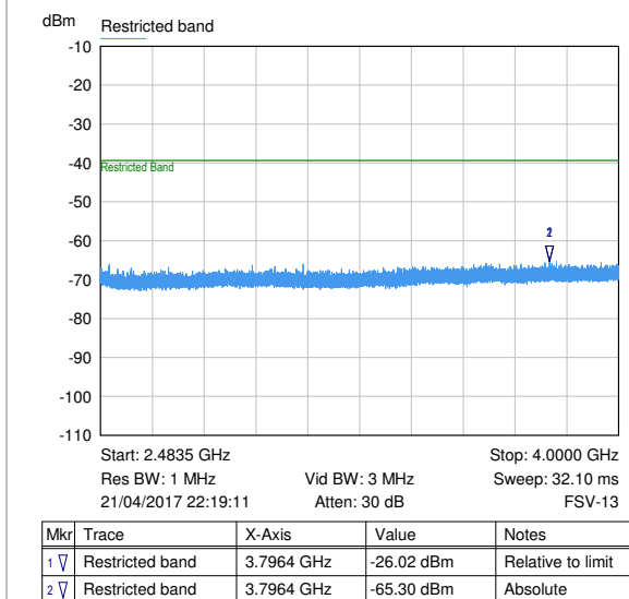
Ch 19: trace 3; 2483.5 - 4000 MHz
