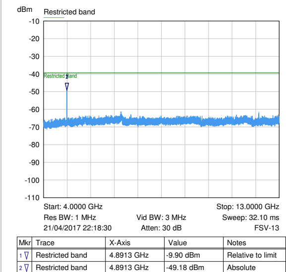
Ch 19: trace 4; 4000 - 13000 MHz
