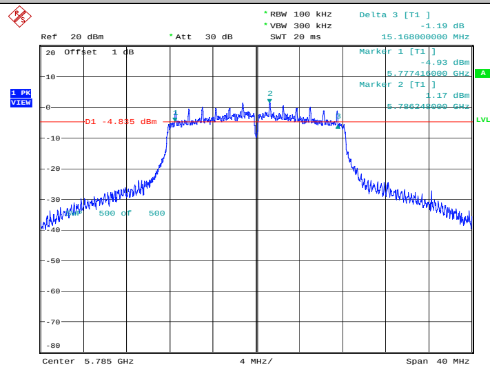
11A_Ant1_5785
