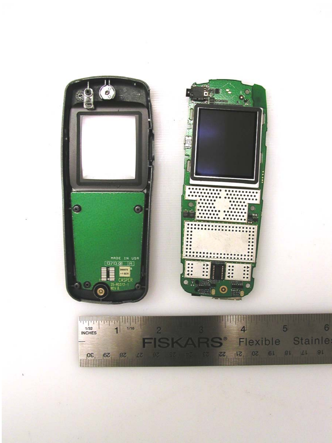
Front housing assembly with main printed wiring board removed
