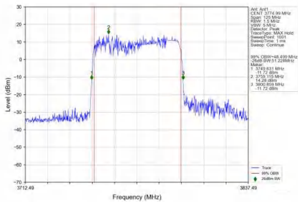
n78a_15kHz_SISO_NTNV_50MHz_DFT-s-OFDM_256_QAM_3774.99MHz_Outer_Full_Ant1
