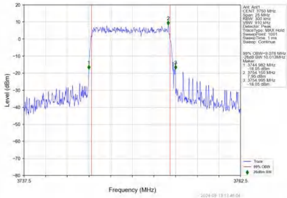
n78a_15kHz_SISO_NTNV_10MHz_DFT-s-OFDM_256_QAM_3750MHz_Outer_Full
