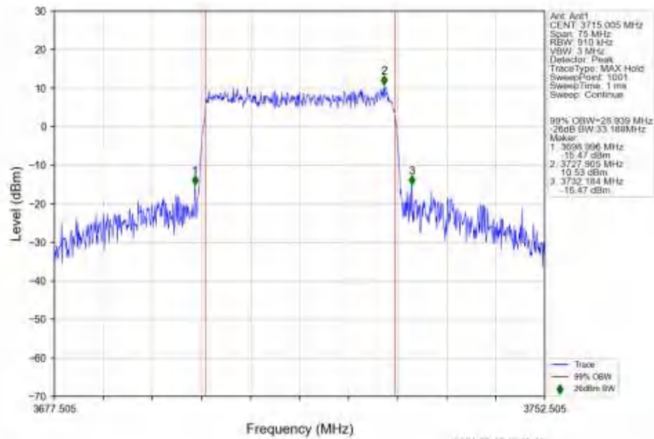
n78a_15kHz_SISO_NTNV_30MHz_CP-OFDM_64_QAM_3715.005MHz_Outer_Full
