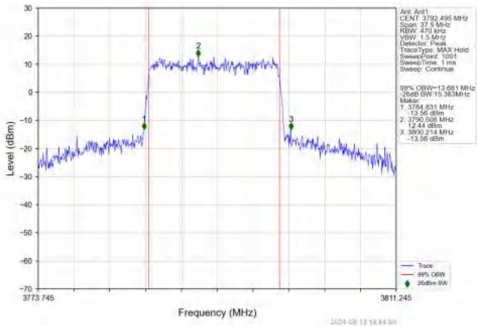
n78a_15kHz_SISO_NTNV_15MHz_DFT-s-OFDM_QPSK_3792.495MHz_Outer_Full
