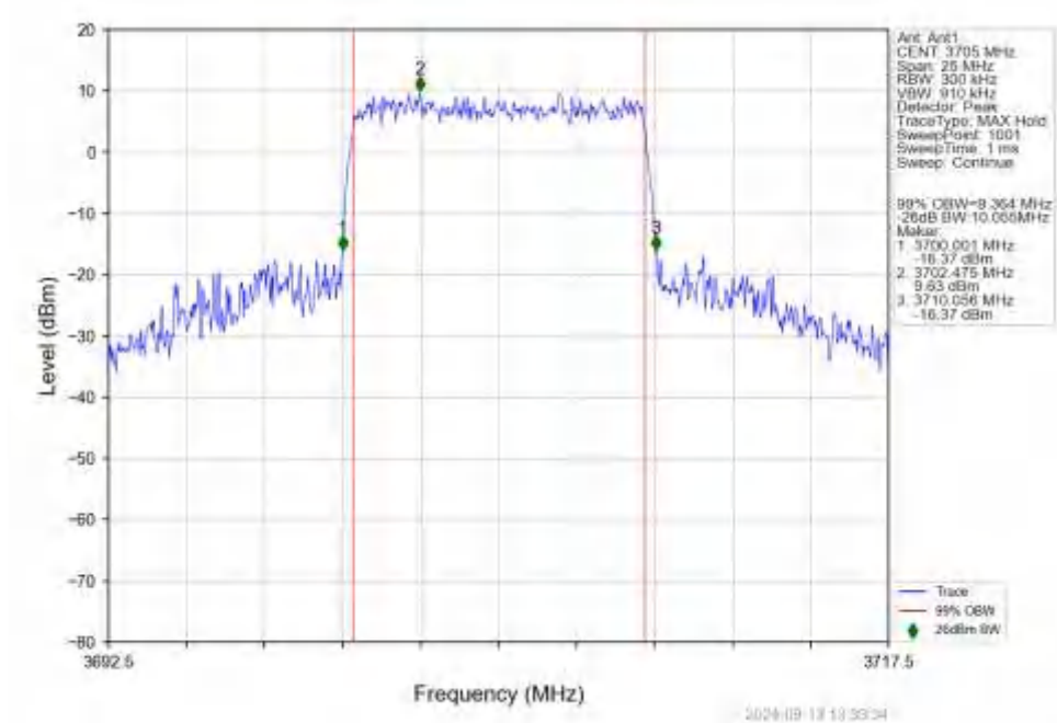
n78a_15kHz_SISO_NTNV_10MHz_CP-OFDM_QPSK_3705MHz_Outer_Full
