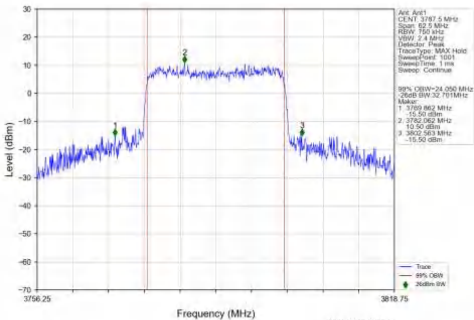
n78a_15kHz_SISO_NTNV_25MHz_CP-OFDM_QPSK_3787.5MHz_Outer_Full
