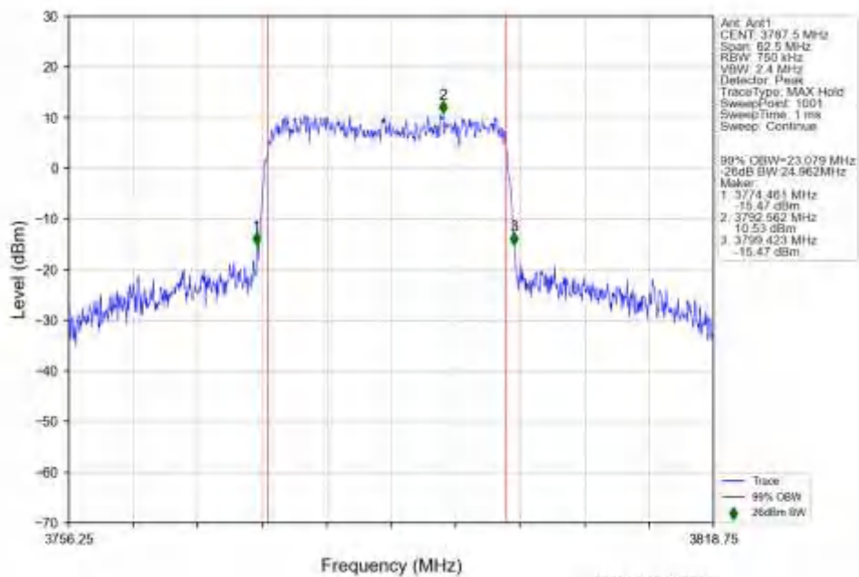
n78a_15kHz_SISO_NTNV_25MHz_DFT-s-OFDM_64_QAM_3787.5MHz_Outer_Full
