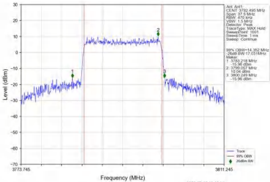
n78a_15kHz_SISO_NTNV_15MHz_CP-OFDM_QPSK_3792.495MHz_Outer_Full
