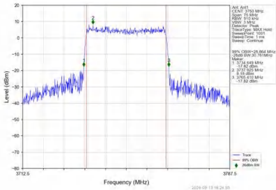
n78a_15kHz_SISO_NTNV_30MHz_CP-OFDM_256_QAM_3750MHz_Outer_Full
