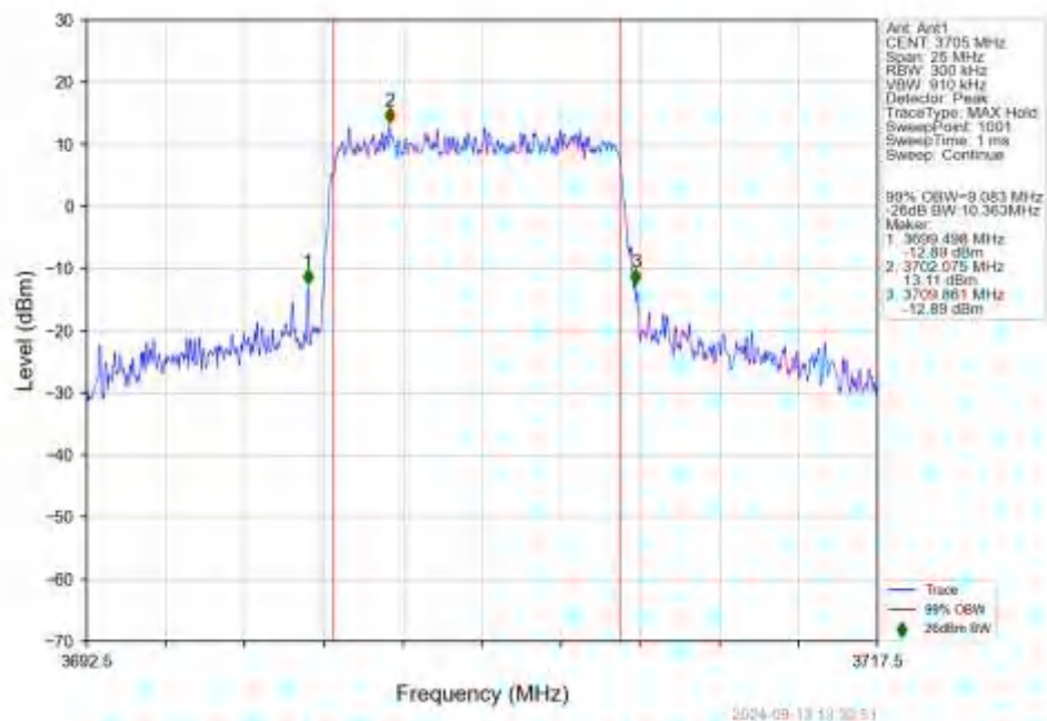
n78a_15kHz_SISO_NTNV_10MHz_DFT-s-OFDM QPSK_3705MHz_Outer_Full
