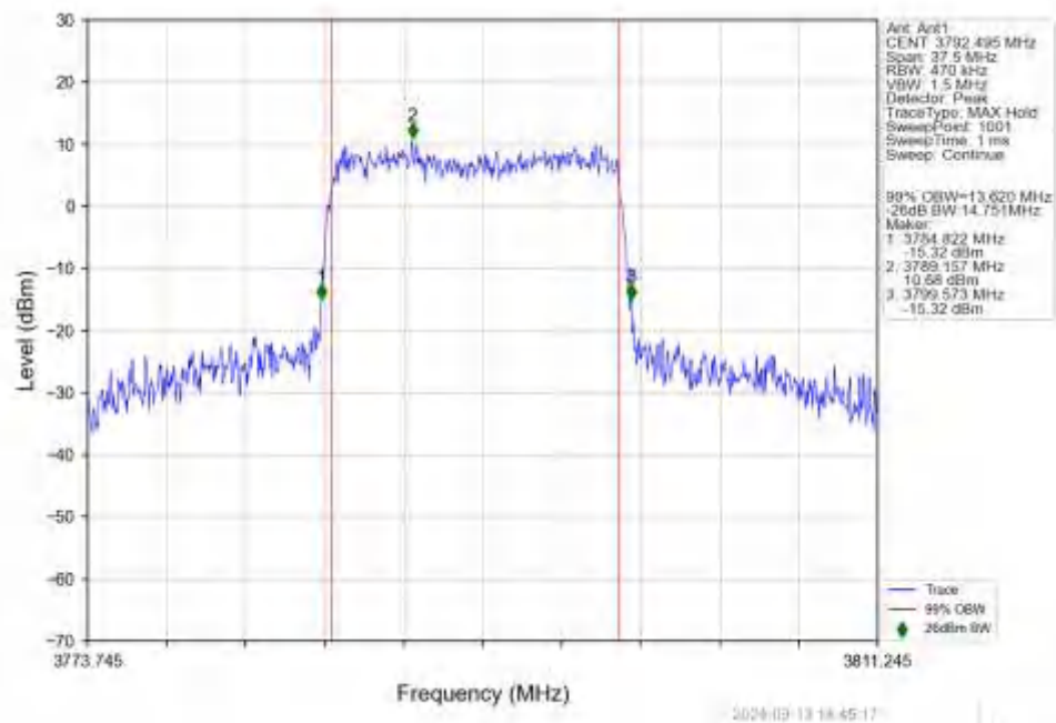
n78a_15kHz_SISO_NTNV_15MHz_DFT-s-OFDM_64_QAM_3792.495MHz_Outer_Full
