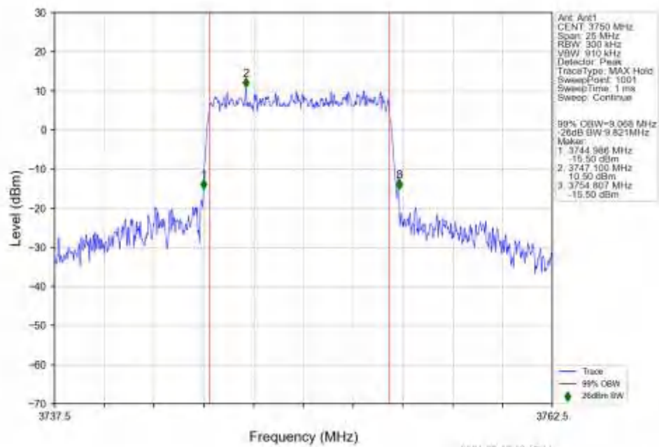
n78a_15kHz_SISO_NTNV_10MHz_DFT-s-OFDM_16_QAM_3750MHz_Outer_Full
