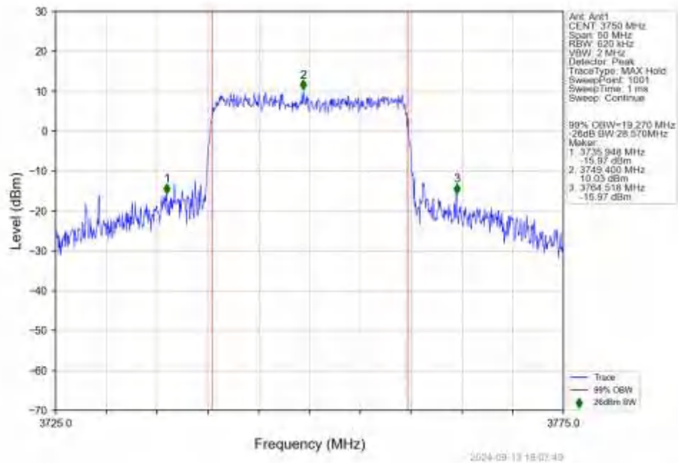
n78a_15kHz_SISO_NTNV_20MHz_CP-OFDM_16_QAM_3750MHz_Outer_Full
