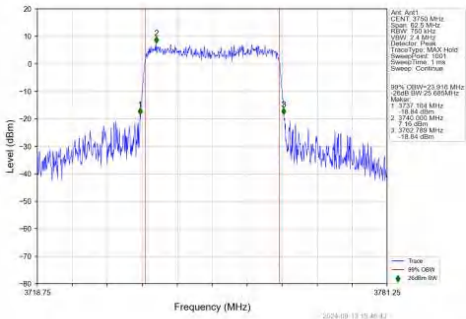
n78a_15kHz_SISO_NTNV_25MHz_CP-OFDM_256_QAM_3750MHz_Outer_Full
