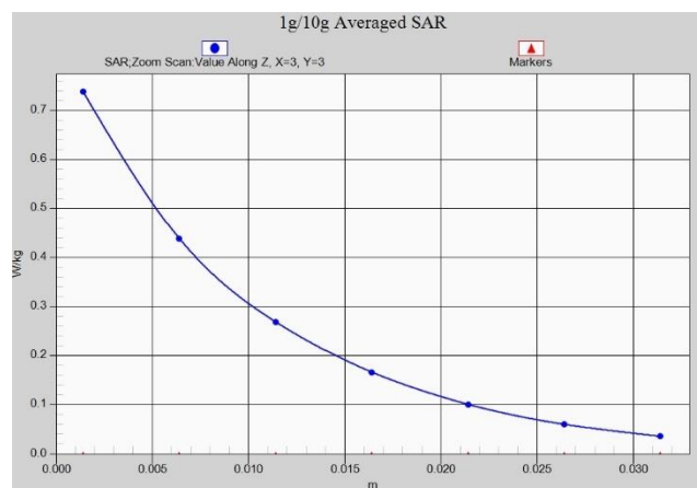
Fig. 1-24 Z-Scan at power reference point (LTE B66 Body)
