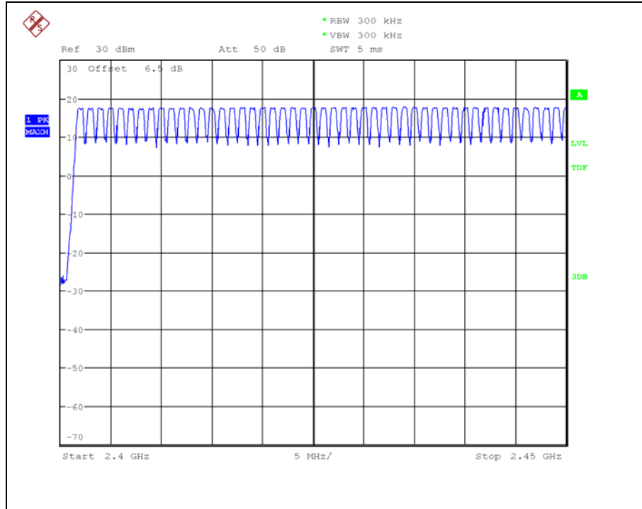
GFSK _ Hopping Mode Number of Hopping Frequencies
