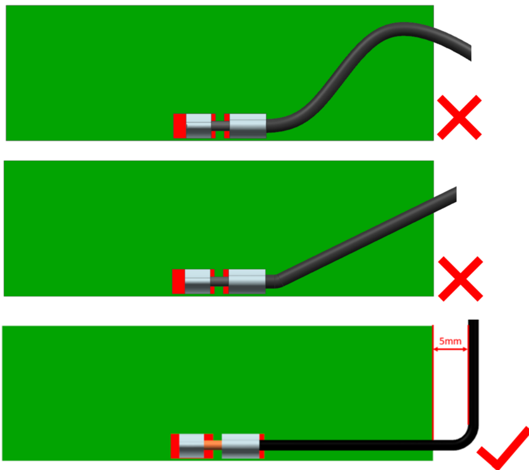
FIGURE 5.2 CABLE BENDING
