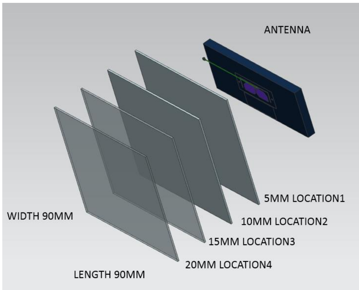
FIGURE 7.1.1 FOUR LOCATIONS WITH PARALLEL PLANE GROUND
