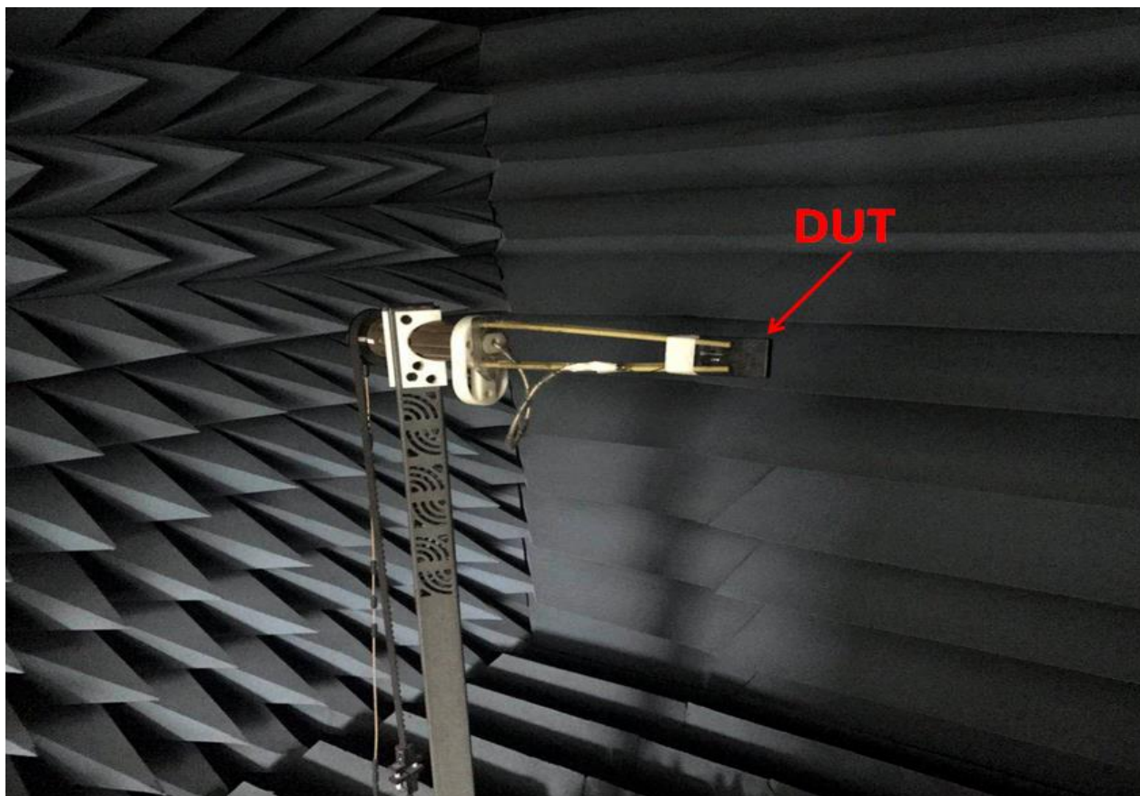
FIGURE4.1.3 ANTENNA LOADED WITH PC/ABS BLOCK OF 1MM THICKNESS TESTED IN OTA CHAMBER
