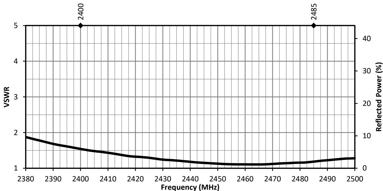
Figure 2. ANT-2.4-CW-RCL VSWR
