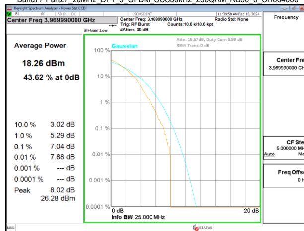
Band77-Part27_20MHz_DFT_s_OFDM_SCS30kHz_256QAM_RB50_0_CH664666
