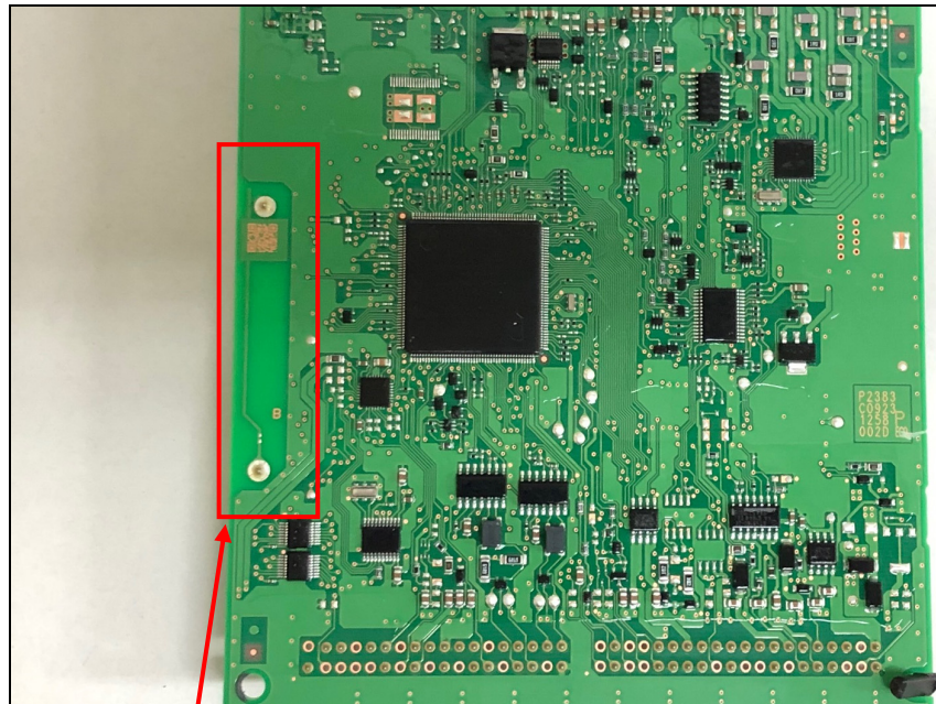
Rx Antenna
