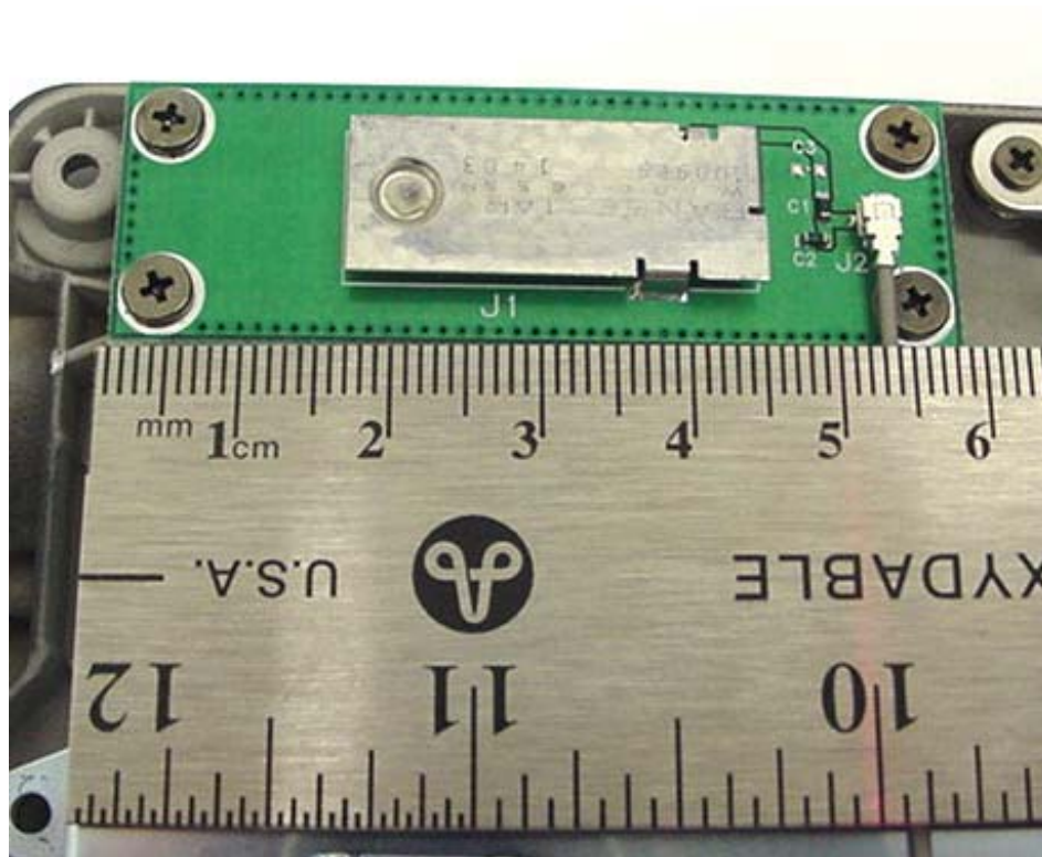
Spacing between WLAN Dual Antennas (Primary)
