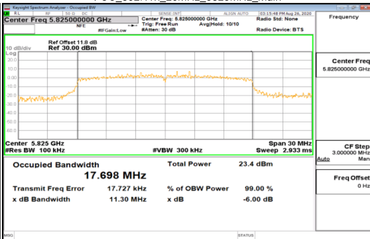
FCC_802.11n_20MHz_5825MHz_Main
