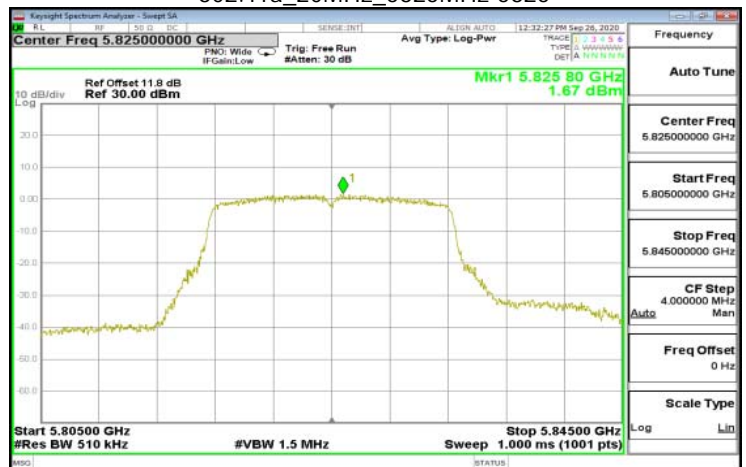
802.11a_20MHz_5825MHz-5825
