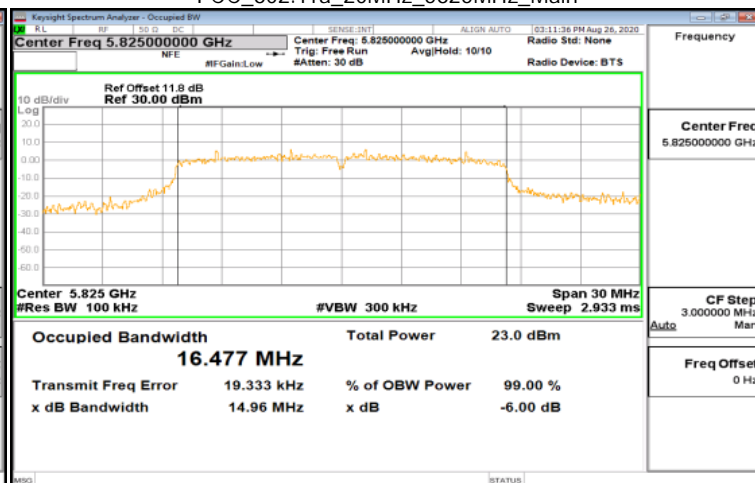
FCC_802.11a_20MHz_5825MHz_Main
