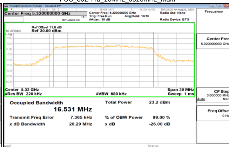
FCC_802.11a_20MHz_5320MHz_Main
