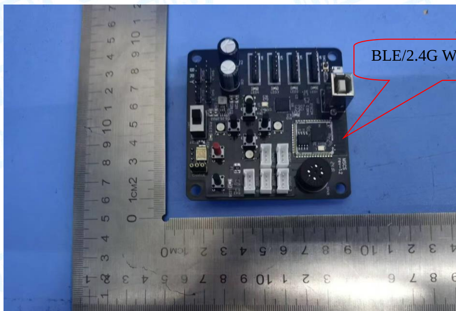
Photo 14 Appearance of PCB
