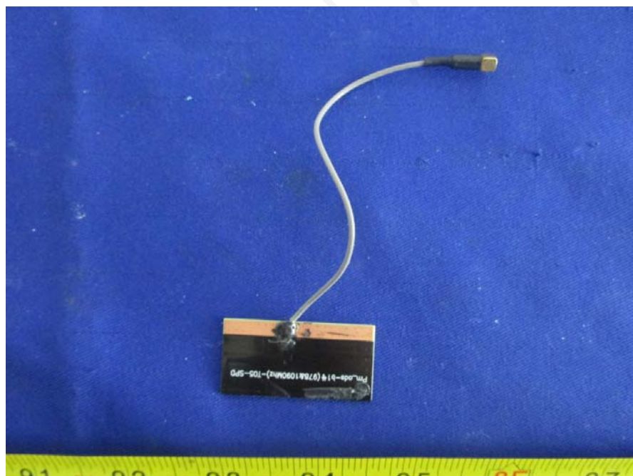
EUT- ADS-B Antenna View
