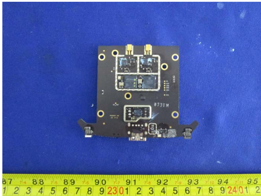
EUT- ADS-B Board Bottom View
