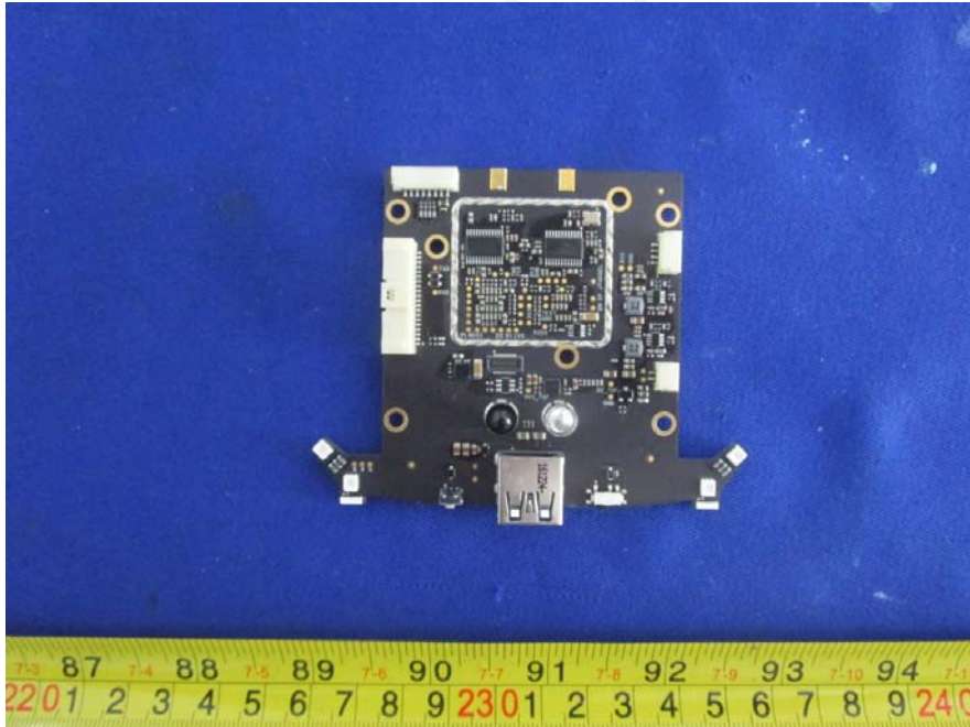
EUT- ADS-B Board Top View
