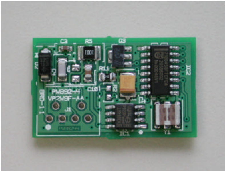
Ford U222/U228 PCB (top)
