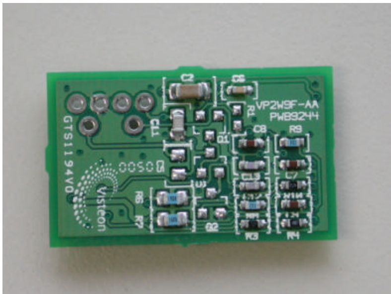
Mazda J56 PCB (bottom)
