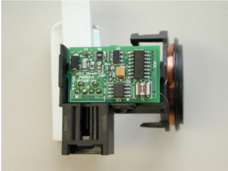
Mazda J56 Case Open
