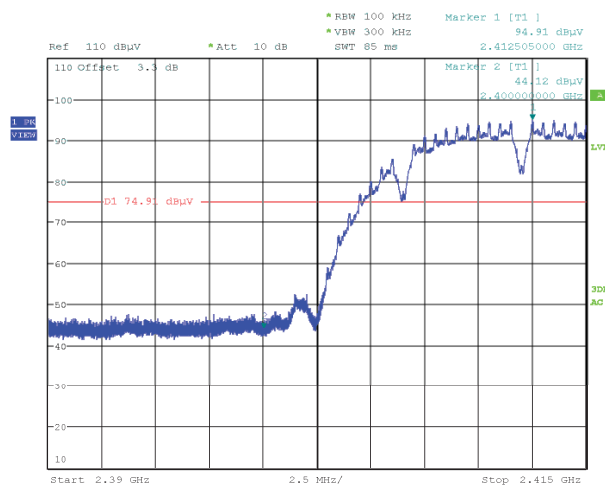
Figure 90: Radiated Emissions at Band Edge (Authorized Band), Spectral Diagram, 802.11b, 2412MHz, with 802.11ac-20, CDD, 5240MHz, Horizontal Antenna Orientation
