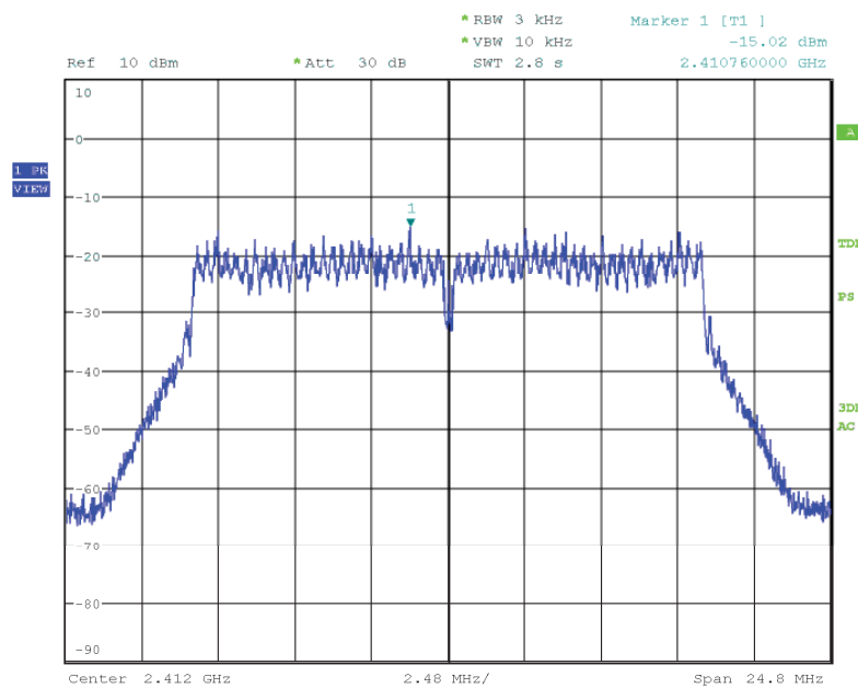
Figure 42: Power Spectral Density, 802.11g, Mode A (2412MHz)
