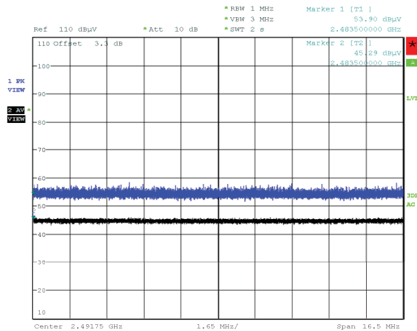
Figure 94: Radiated Emissions at Band Edge (Restricted Band), Spectral Diagram, 802.11b, 2462MHz, with 802.11ac-20, CDD, 5240MHz, Horizontal Antenna Orientation
