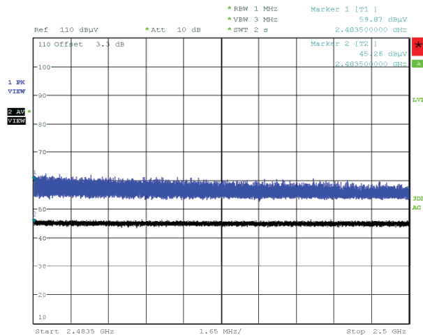
Figure 104: Radiated Emissions at Band Edge (Restricted Band), Spectral Diagram, 802.11g, 2457MHz, with 802.11ac-20, CDD, 5240MHz, Horizontal Antenna Orientation
