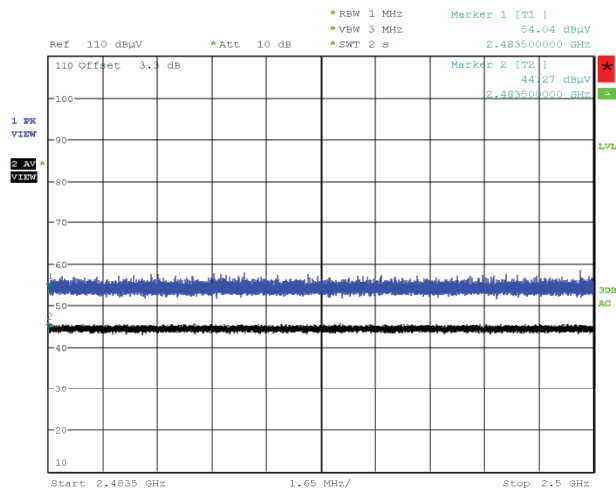
Figure 87: Radiated Emissions at Band Edge (Restricted Band), Spectral Diagram, 802.11n-20, 2457MHz, Vertical Antenna Orientation
