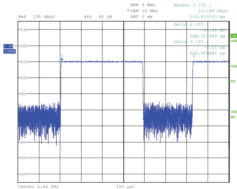
Figure 57: Duty Cycle, BLE 1M-PHY, Mode B (2440MHz)
