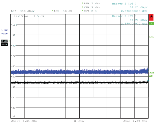
Figure 73: Radiated Emissions at Band Edge (Restricted Band), Spectral Diagram, 802.11g, 2417MHz, Vertical Antenna Orientation
