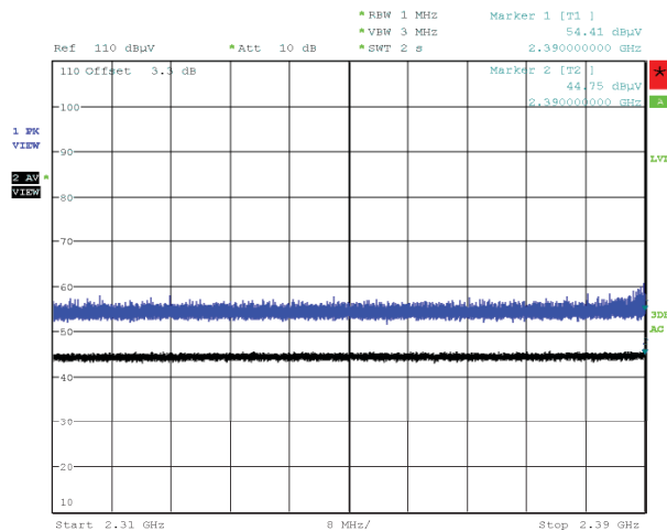
Figure 110: Radiated Emissions at Band Edge (Restricted Band), Spectral Diagram, 802.11n-20, 2412MHz, with 802.11ac-20, CDD, 5240MHz, Horizontal Antenna Orientation
