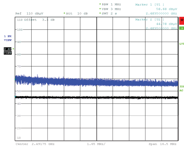
Figure 118: Radiated Emissions at Band Edge (Restricted Band), Spectral Diagram, 802.11n-20, 2462MHz, with 802.11ac-20, CDD, 5240MHz, Horizontal Antenna Orientation
