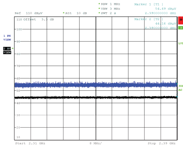
Figure 92: Radiated Emissions at Band Edge (Restricted Band), Spectral Diagram, 802.11b, 2412MHz, with 802.11ac-20, CDD, 5240MHz, Horizontal Antenna Orientation
