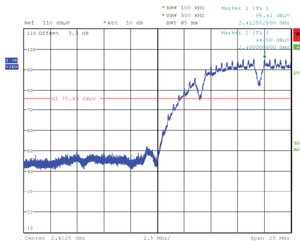
Figure 60: Radiated Emissions at Band Edge (Authorized Band), Spectral Diagram, 802.11b, 2412MHz, Horizontal Antenna Orientation
