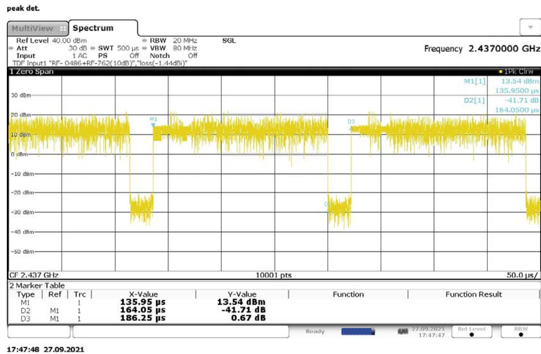
Figure 56: Duty Cycle, 802.11n-20, Mode B (2437MHz)
