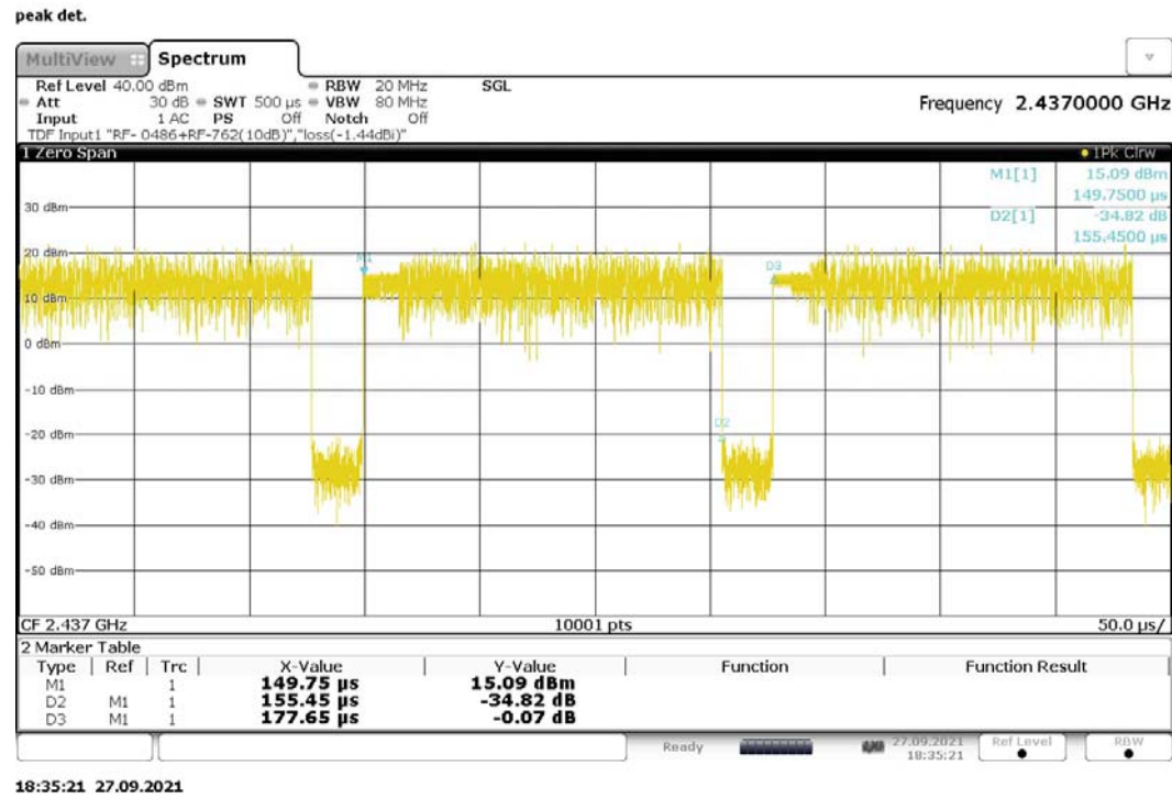
Figure 55: Duty Cycle, 802.11g, Mode B (2437MHz)
