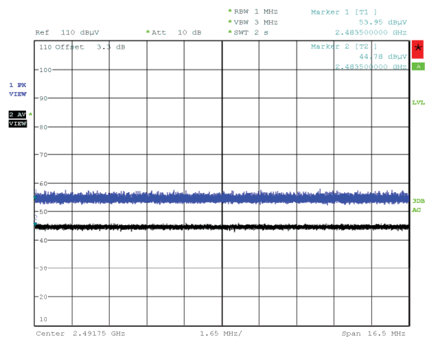
Figure 117: Radiated Emissions at Band Edge (Restricted Band), Spectral Diagram, 802.11n-20, 2457MHz, with 802.11ac-20, CDD, 5240MHz, Vertical Antenna Orientation
