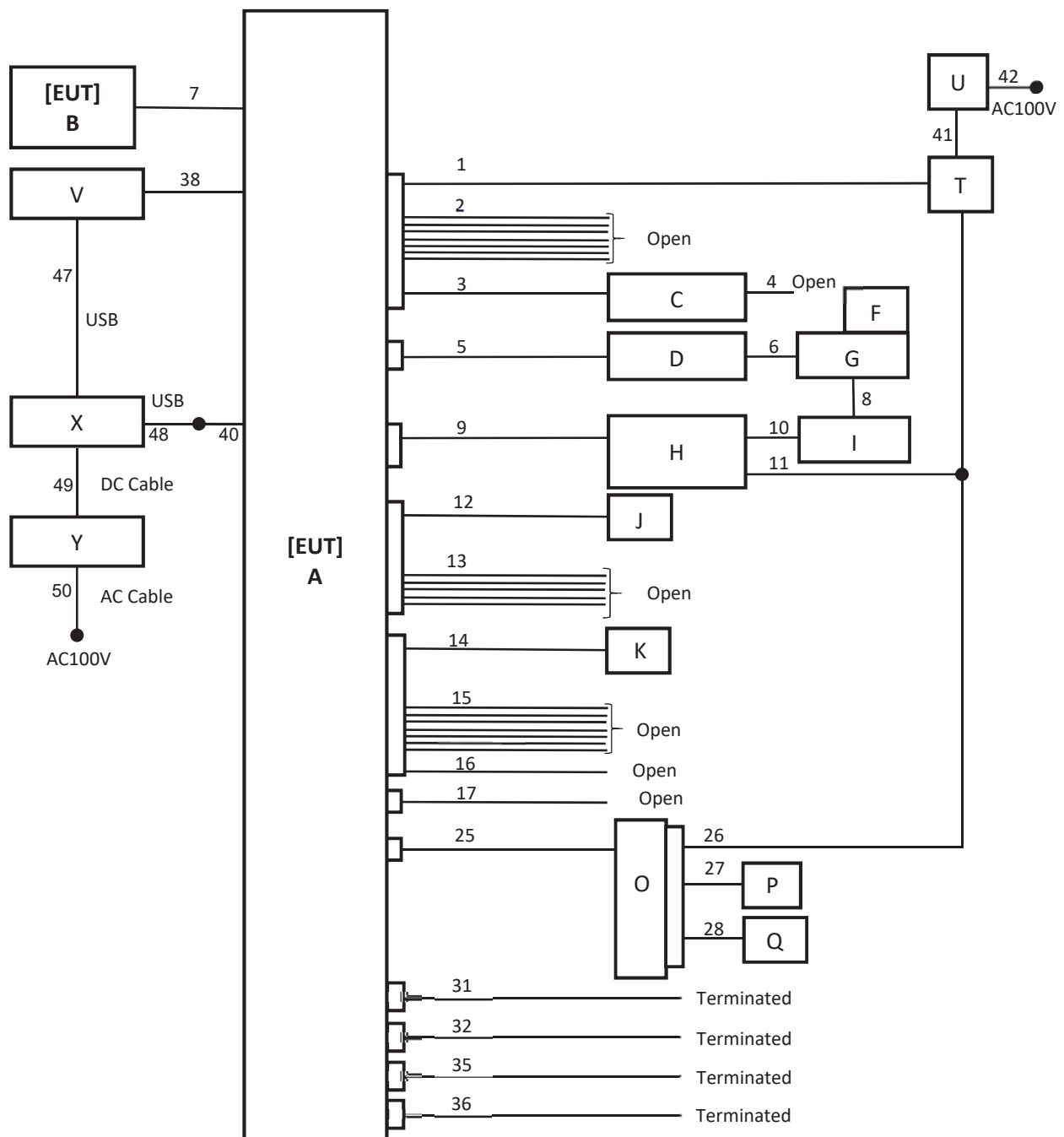
Figure 1: Block Diagram
