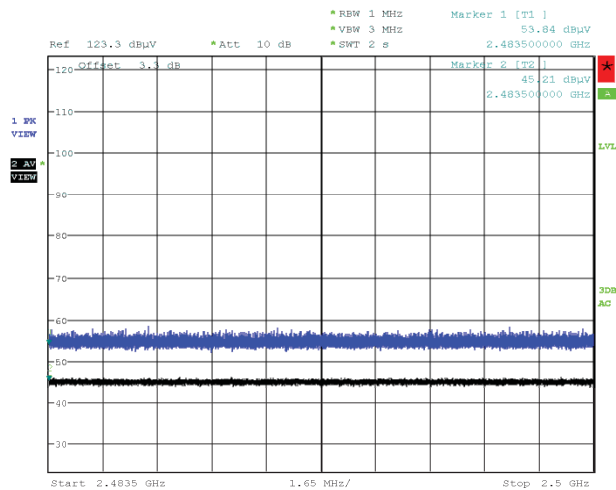
Figure 89: Radiated Emissions at Band Edge (Restricted Band), Spectral Diagram, 802.11n-20, 2462MHz, Vertical Antenna Orientation
