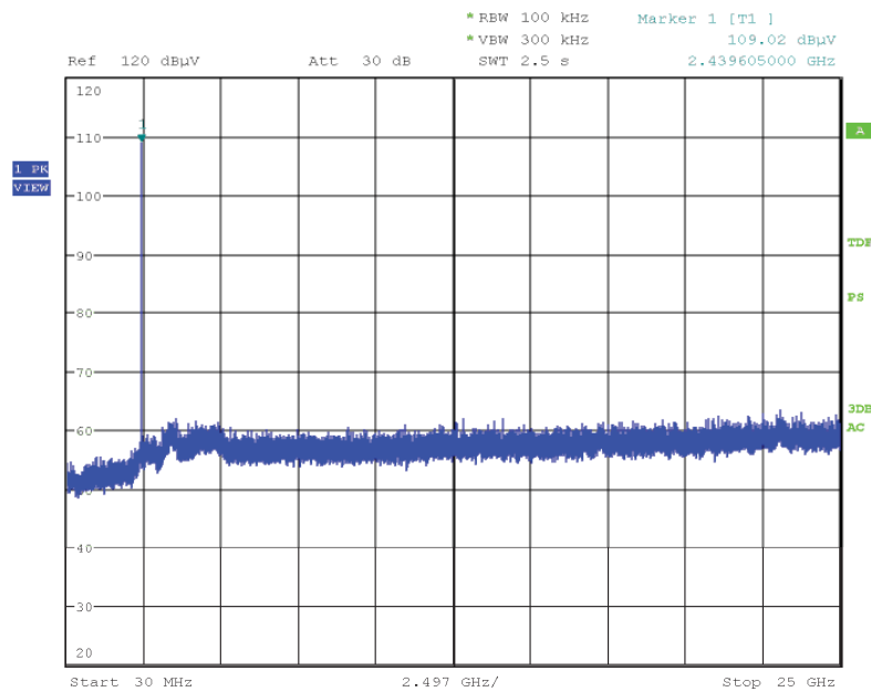
Figure 34: Conducted Spurious Emissions, 30MHz - 25GHz, BLE 1M-PHY, Mode B (2440MHz)
