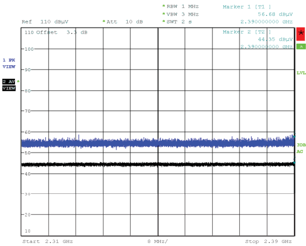
Figure 103: Radiated Emissions at Band Edge (Restricted Band), Spectral Diagram, 802.11g, 2417MHz, with 802.11ac-20, CDD, 5240MHz, Vertical Antenna Orientation
