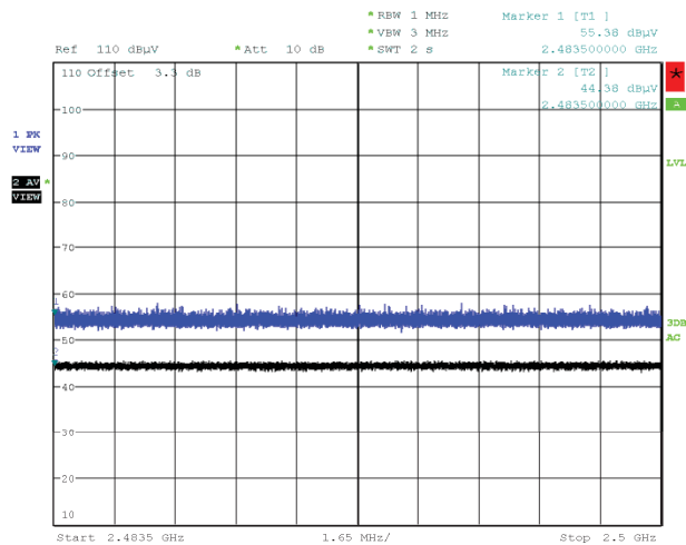
Figure 77: Radiated Emissions at Band Edge (Restricted Band), Spectral Diagram, 802.11g, 2462MHz, Vertical Antenna Orientation
