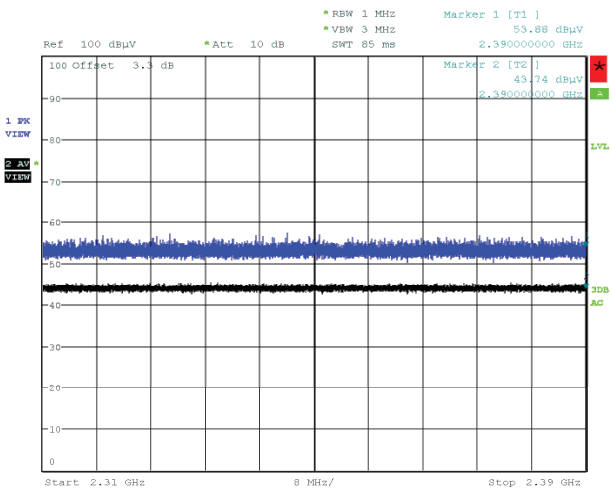
Figure 63: Radiated Emissions at Band Edge (Restricted Band), Spectral Diagram, 802.11b, 2412MHz, Vertical Antenna Orientation
