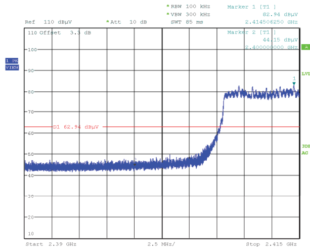
Figure 113: Radiated Emissions at Band Edge (Authorized Band), Spectral Diagram, 802.11n-20, 2417MHz, with 802.11ac-20, CDD, 5240MHz, Vertical Antenna Orientation
