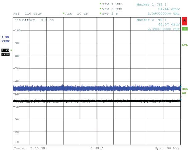
Figure 69: Radiated Emissions at Band Edge (Restricted Band), Spectral Diagram, 802.11g, 2412MHz, Vertical Antenna Orientation
