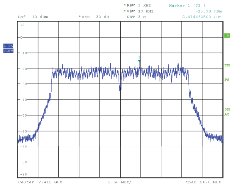
Figure 45: Power Spectral Density, 802.11n-20, Mode A (2412MHz)
