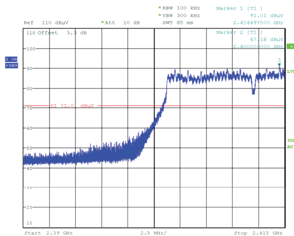
Figure 108: Radiated Emissions at Band Edge (Authorized Band), Spectral Diagram, 802.11n-20, 2412MHz, with 802.11ac-20, CDD, 5240MHz, Horizontal Antenna Orientation
