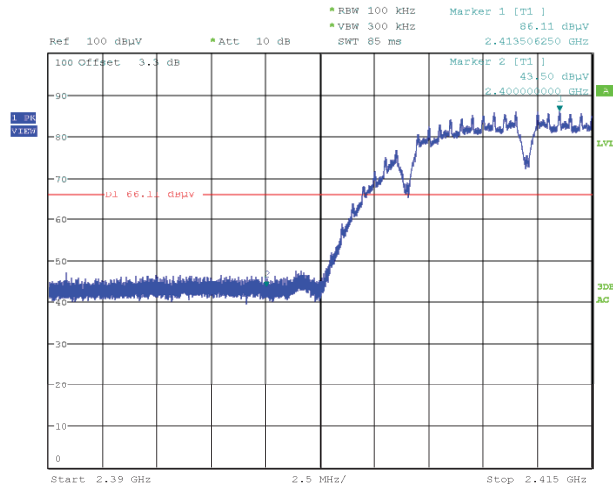
Figure 61: Radiated Emissions at Band Edge (Authorized Band), Spectral Diagram, 802.11b, 2412MHz, Vertical Antenna Orientation
