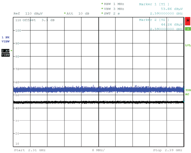
Figure 111: Radiated Emissions at Band Edge (Restricted Band), Spectral Diagram, 802.11n-20, 2412MHz, with 802.11ac-20, CDD, 5240MHz, Vertical Antenna Orientation
