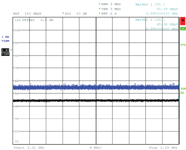
Figure 99: Radiated Emissions at Band Edge (Restricted Band), Spectral Diagram, 802.11g, 2412MHz, with 802.11ac-20, CDD, 5240MHz, Vertical Antenna Orientation
