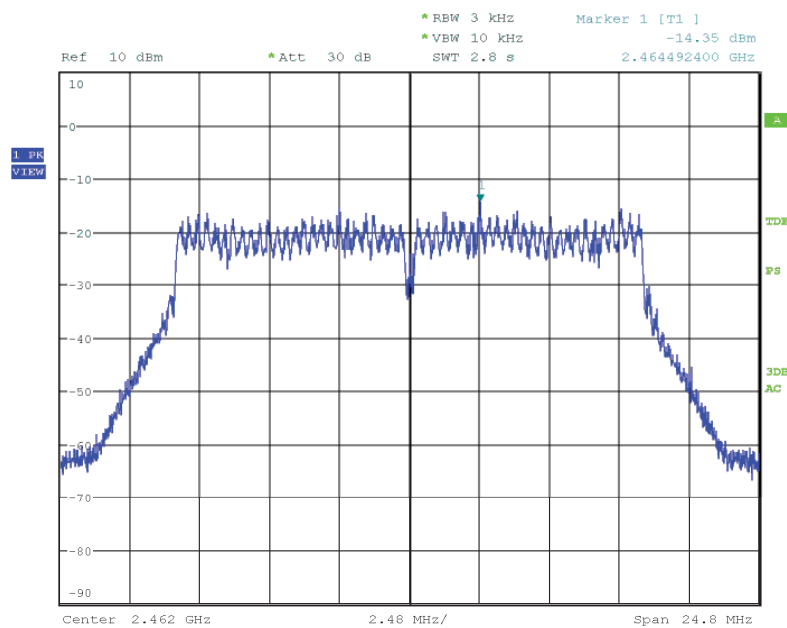
Figure 44: Power Spectral Density, 802.11g, Mode C (2462MHz)
