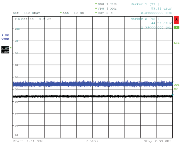
Figure 85: Radiated Emissions at Band Edge (Restricted Band), Spectral Diagram, 802.11n-20, 2417MHz, Vertical Antenna Orientation
