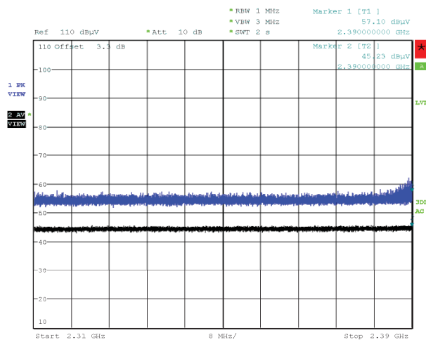
Figure 114: Radiated Emissions at Band Edge (Restricted Band), Spectral Diagram, 802.11n-20, 2417MHz, with 802.11ac-20, CDD, 5240MHz, Horizontal Antenna Orientation
