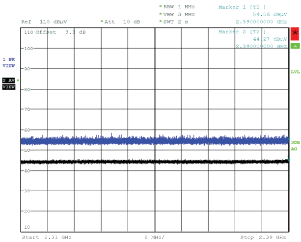
Figure 81: Radiated Emissions at Band Edge (Restricted Band), Spectral Diagram, 802.11n-20, 2412MHz, Vertical Antenna Orientation
