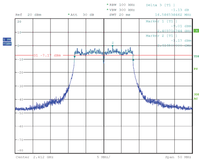
Figure 5: 6dB Bandwidth, 802.11g, Mode A (2412MHz)
