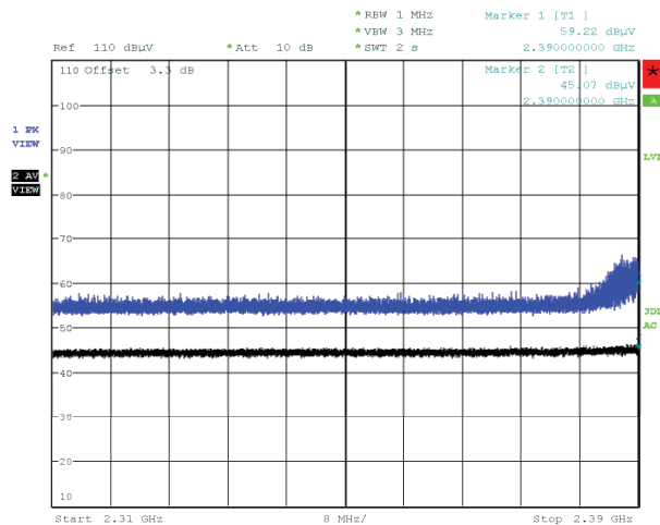
Figure 102: Radiated Emissions at Band Edge (Restricted Band), Spectral Diagram, 802.11g, 2417MHz, with 802.11ac-20, CDD, 5240MHz, Horizontal Antenna Orientation
