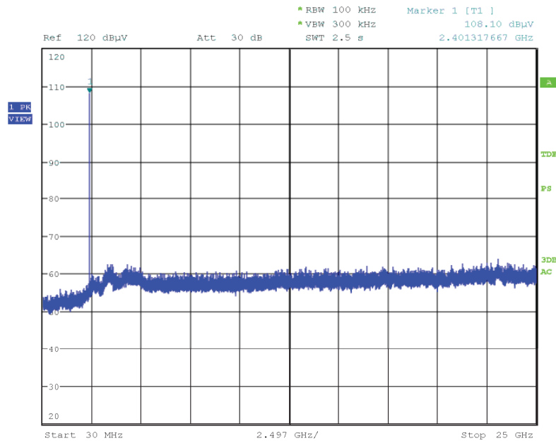
Figure 33: Conducted Spurious Emissions, 30MHz - 25GHz, BLE 1M-PHY, Mode A (2402MHz)
