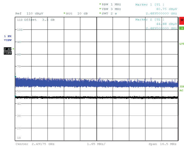
Figure 116: Radiated Emissions at Band Edge (Restricted Band), Spectral Diagram, 802.11n-20, 2457MHz, with 802.11ac-20, CDD, 5240MHz, Horizontal Antenna Orientation
