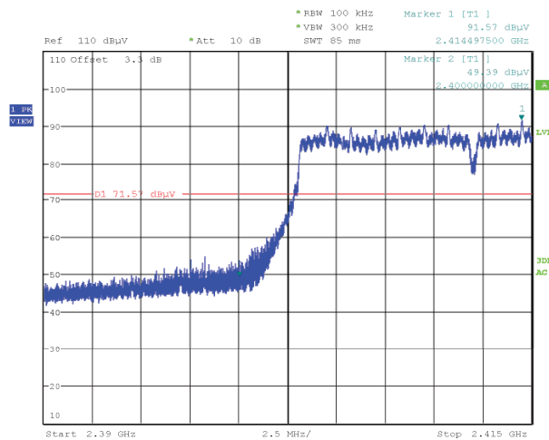
Figure 78: Radiated Emissions at Band Edge (Authorized Band), Spectral Diagram, 802.11n-20, 2412MHz, Horizontal Antenna Orientation
