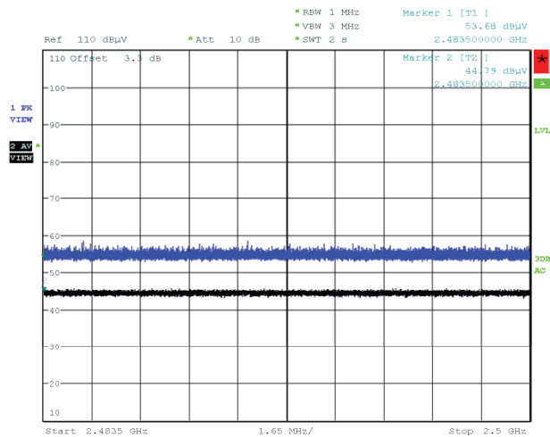
Figure 75: Radiated Emissions at Band Edge (Restricted Band), Spectral Diagram, 802.11g, 2457MHz, Vertical Antenna Orientation
