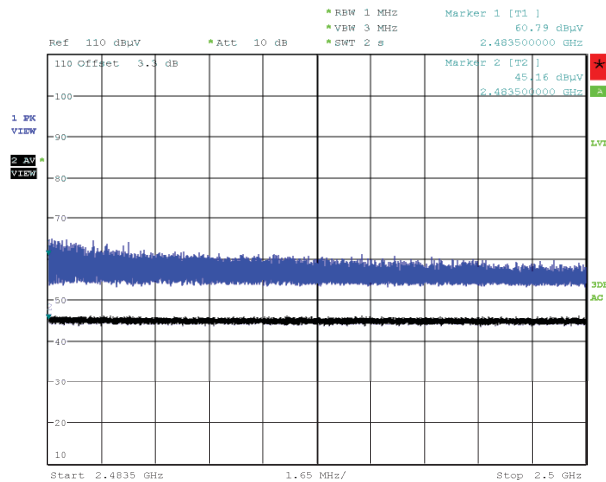
Figure 106: Radiated Emissions at Band Edge (Restricted Band), Spectral Diagram, 802.11g, 2462MHz, with 802.11ac-20, CDD, 5240MHz, Horizontal Antenna Orientation
