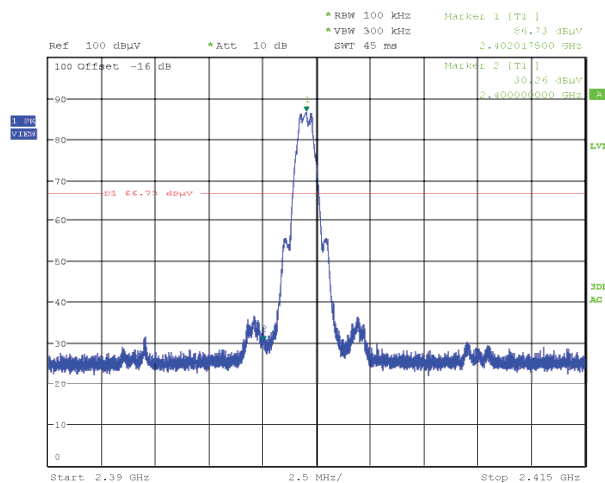
Figure 120: Radiated Emissions at Band Edge (Authorized Band), Spectral Diagram, BLE 1M-PHY, 2402MHz, Horizontal Antenna Orientation
