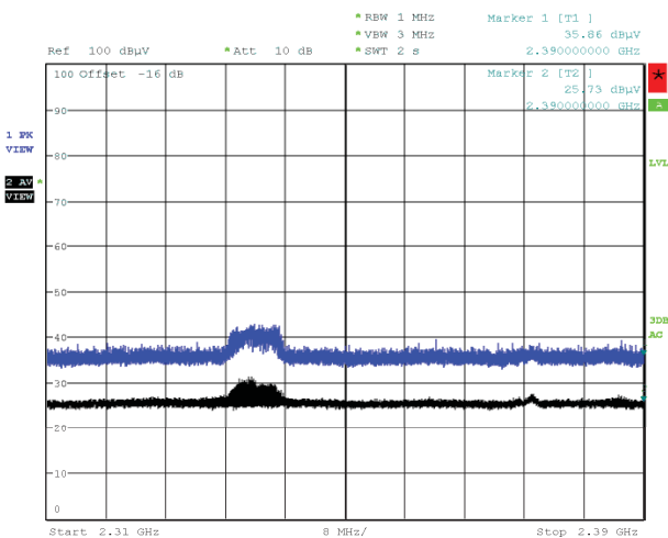
Figure 129: Radiated Emissions at Band Edge (Restricted Band), Spectral Diagram, BLE 2M-PHY, 2402MHz, Vertical Antenna Orientation
