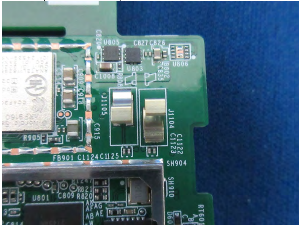
(37) EUT Photo (BT LE+WiFi Antenna)
